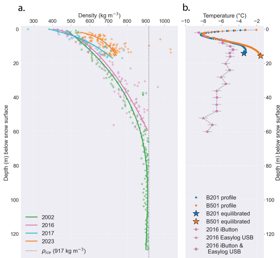
Figure 12. Eclipse 2023 (a) firn densities and (b) borehole temperatures in comparison to measurements at Eclipse from 2002, 2016 and 2017. Measured density values are shown by circles in panel (a) with a curve fitted to each year’s data. The density of solid ice is shown in panel (a) by the dotted gray line. Curves are not fitted to temperature data in panel (b). Uncertainty in 2016 temperature measurements is shown by the gray error bars. Error bars for 2023 measurements are too short to be visible behind the markers.
