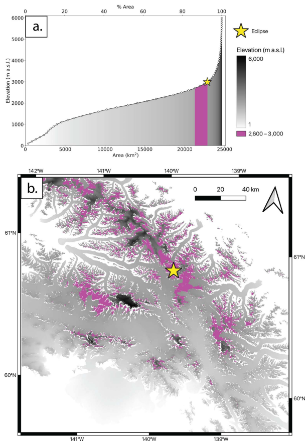
Figure 11. Hypsometric curve (a) and elevation map (b) of Eclipse Icefield and the surrounding area. Elevation is shown by the grayscale shading, with higher elevations indicated by darker grays. Elevations between 2,600 m a.s.l. and 3,000 m a.s.l. (the approximate elevations of the Kaskawulsh/Hubbard divide and Eclipse) are shown in magenta. The location of Eclipse is indicated with a yellow star.
