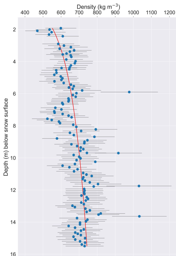
Figure 4. Firm densities of 2023 core B501 with uncertainty values (gray) and a best-fit logarithmic curve (red). Measured densities begin at 1.92 m because the snow above that depth was too crumbly for accurate volume measurements.
