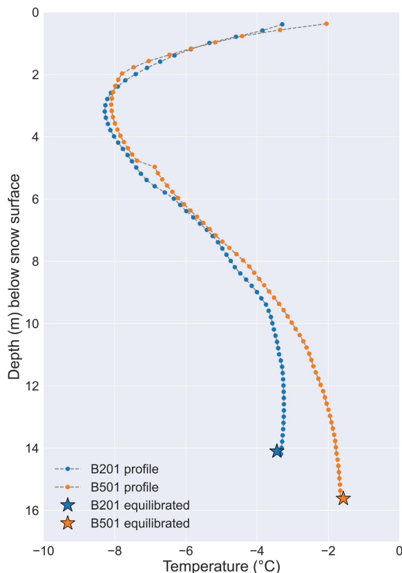
Figure 5. Borehole temperatures measured at Eclipse in 2023. Full 2023 profiles (circles) were acquired with 15 s sensor equilibration at each depth. Near the bottom of each borehole, one measurement (star marker) was acquired after allowing the sensor to equilibrate for 1.5 hours.
