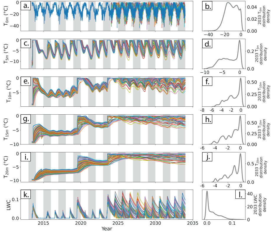
Figure B2. Temperature (a-j) and liquid water content (LWC; k-l) timeseries and distribution plots for model runs that produce realistic results at Eclipse Icefield. Temperatures are shown at 0 m (a-b), 5 m (c-d), 10 m (e-f), 15 m (g-h), 20 m (i-j) depth. LWC is calculated for the entire firn column. All model runs were forced using downscaled NARR air temperatures during the spinp period (pre-2013), elevation-corrected Divide AWS data from 2013–2024, and temperatures randomly drawn from a Gaussian distribution described by the mean and standard deviation of elevation-corrected 2013–2024 Divide AWS temperatures from 2024–2033. Forcing temperatures from 2024–2033 assume a continuation of current climate conditions. Gray bars show odd-numbered years (e.g. 2015, 2017, etc.). Values on the x-axis of the righthand panels (distributions) correspond to those on the y-axis of the lefthand panels (timeseries). Distributions are shown for 2033 outputs only.
