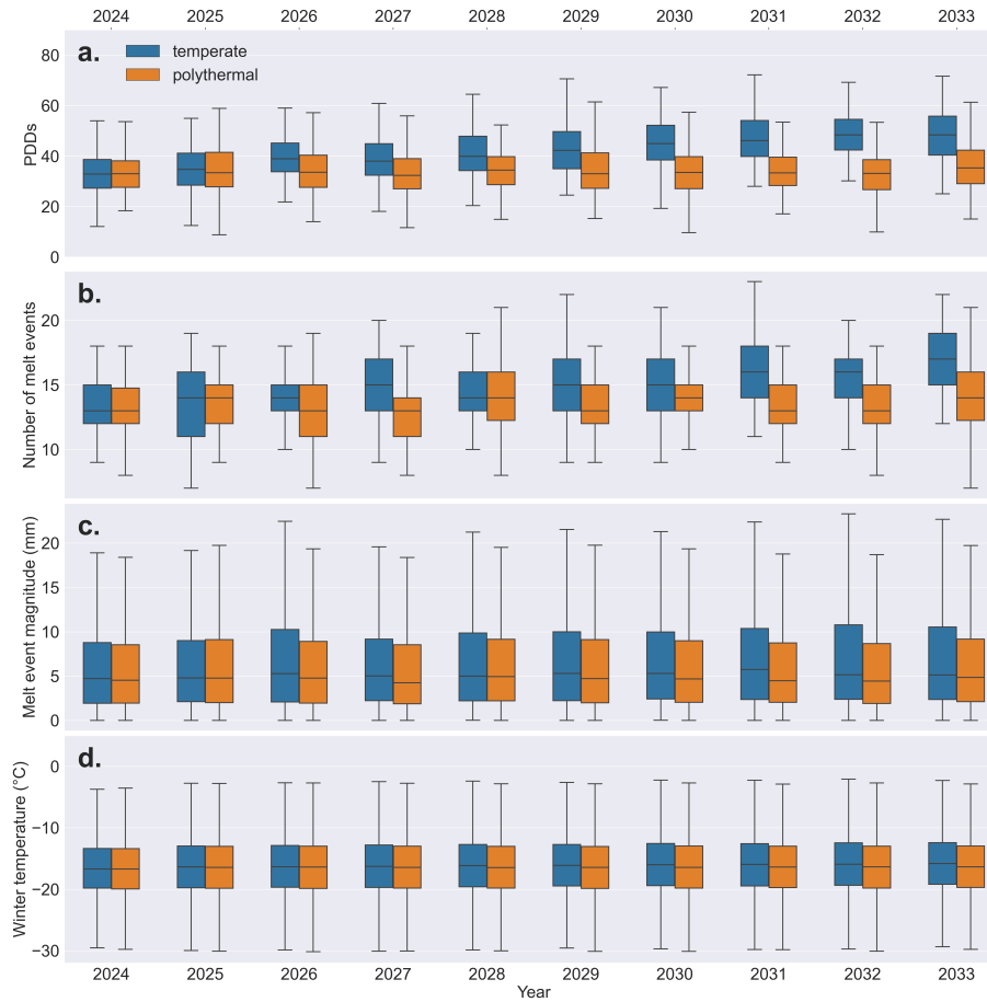
Figure 8. Positive-Melt season positive degree days (PDDs, a) from May through September, number of melt events (b), melt event magnitude (c), and wintertime temperatures (d) each year for model runs that produce year-round temperate firn at 15 m depth by 2033 (blue) and those that don't do not (orange). We define the melt season here as May-September, and wintertime as October-March. Outliers are excluded for clarity.
