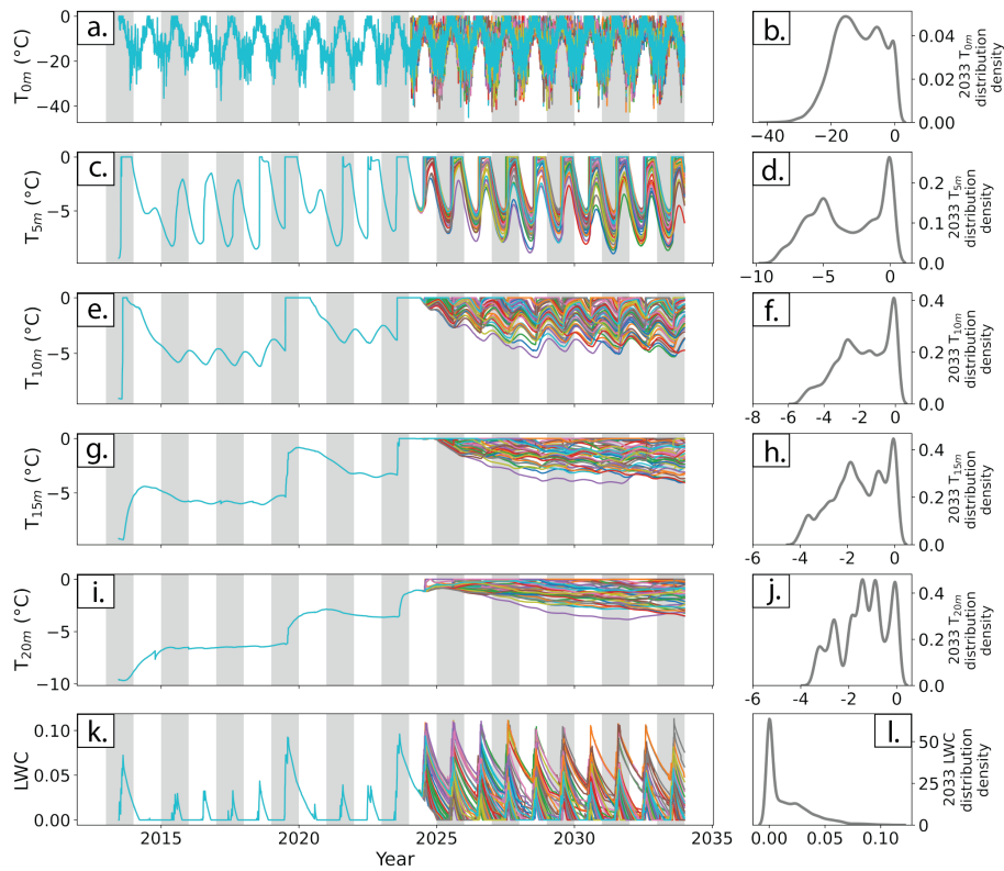
Figure 6. Firn temperature (a-j) and liquid water content (LWC; k-l) timeseries and distribution plots for replicate runs of our reference model at Eclipse Icefield. Temperatures are shown at 0 m (a-b), 5 m (c-d), 10 m (e-f), 15 m (g-h), and 20 m (i-j) depth. LWC is calculated for the entire firn column. A degree day factor (DDF) of 6.2 and a surface density of 450 \text{ kg m}^{-3} were used for all fifty model runs. All model runs were forced using downscaled NARR air temperatures during the spinup period (pre-2013), elevation-corrected Divide AWS data from 2013–2024, and temperatures randomly drawn from a Gaussian distribution described by the mean and standard deviation of elevation-corrected 2013–2024 Divide AWS temperatures from 2024–2033. Forcing temperatures from 2024–2033 assume a continuation of current climate conditions. Gray bars show odd-numbered years (e.g. 2015, 2017, etc.). Values on the x-axis of the righthand panels (distributions) correspond to those on the y-axis of the lefthand panels (timeseries). Distributions include all output values over the course of 2033 (Jan 1 through Dec 31).
