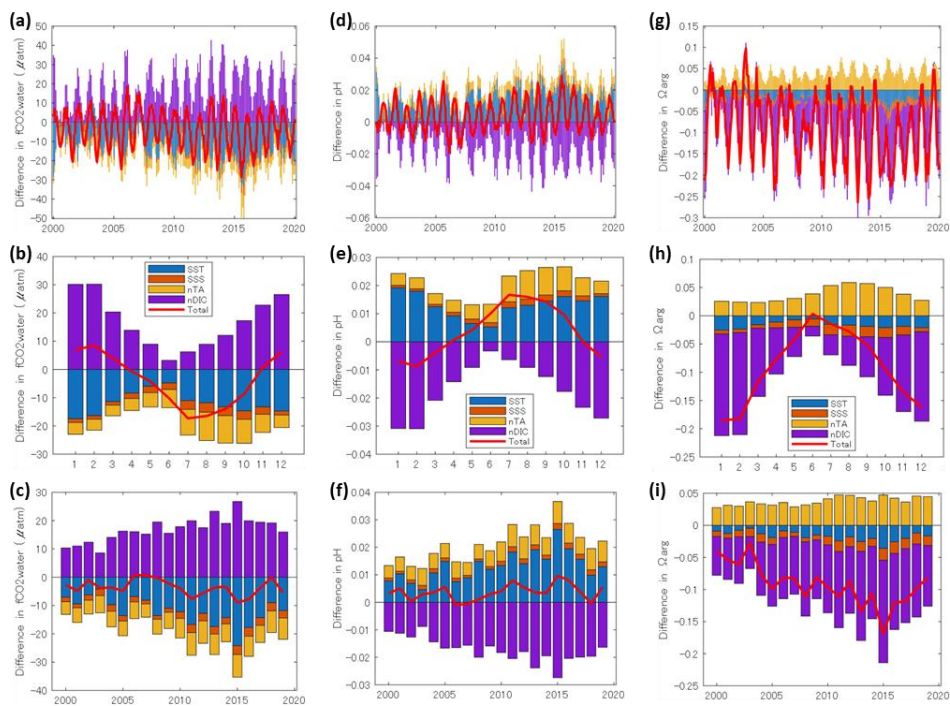
Figures 5. (a): Temporal contributions in the PLS analysis by of Sea Surface Temperature (SST), Sea Surface Salinity (SSS), normalized Total Alkalinity (nTA), and normalized Dissolved Inorganic Carbon (nDIC) in the PLS analysis-SST, SSS, nTA, and nDIC to the difference between Area A and B in (a-c) in-seawater \text{CO}_2 fugacity ( \text{fCO}_2 ), (d-f) pH-between-Area-A-and-B, and (g-i) aragonite saturation state ( \Omega_{\text{arg}} ). Panels show (a, d, g) the temporal contributions, (b, e, h) monthly averages, and (c, f, i) yearly averages. Red lines indicate the sum of contributions, which closely matches the temporal variation of the differences ( d_{AB} ) in each variables. The corresponding monthly averages. (e): The corresponding yearly averages. (d): Temporal contributions in the PLS analysis by SST, SSS, nTA, and nDIC to the difference in \Omega_{\text{calc}} between Area A and B. (e): The monthly averages. (f): The yearly averages. The red lines represent the sum of each contribution and is almost equal to temporal variation of d_{AB} of seawater \text{fCO}_2 and \Omega_{\text{calc}} .
