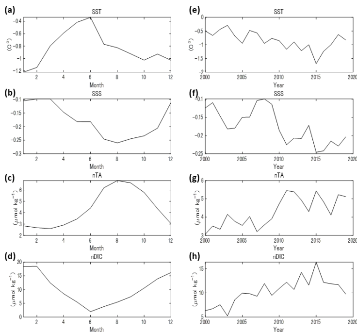
Figure 3. The differences in Sea Surface Temperature (SST) , Sea Surface Salinity (SSS) , normalized Total Alkalinity (nTA) , and normalized Dissolved Inorganic Carbon (nDIC) between Areas A and B ( dAB ). (a)–(d): Seasonal variations. (e)–(h): Annual variations. Although the time step in this study was 0.1 year, the monthly values were calculated by spline interpolation of values at 1/12-year intervals. The same applies to the other figures.
