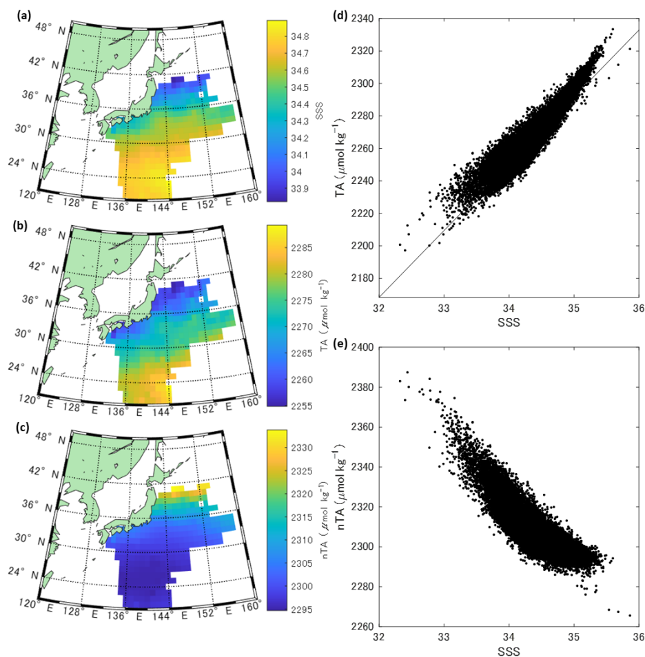
Figure 1 (a–c): Spatial distribution of (a) mean Sea surface Salinity (SSS) (b) Total Alkalinity (TA) and (c) normalized TA (nTA).
