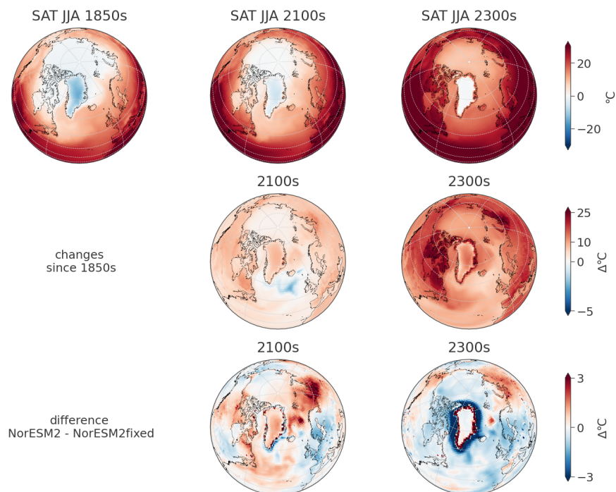
Figure A4. Arctic summer (JJA) surface air temperature as shown in Fig. 2 on Arctic projection. Absolute values 1850, 2100 and 2300 for NorESM2 (top row), changes since the start of the simulation for NorESM2 (second row) and as difference between NorESM2 and NorESM2fixed (third row). To cover differences of the initial climate state in NorESM2 and NorESM2fixed, the last row is calculated as double differences, meaning the difference of changes since the 1850s of the respective simulations.
