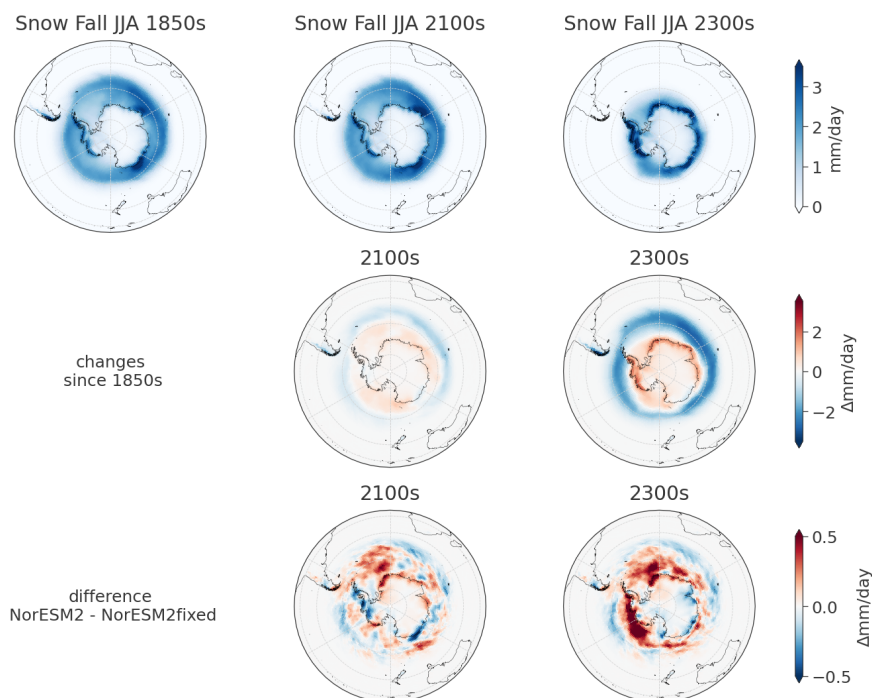
Figure A8. Antarctic winter (JJA) snow fall with absolute values 1850, 2100 and 2300 for NorESM2 (top row), changes since the start of the simulation for NorESM2 (second row) and as difference between NorESM2 and NorESM2fixed (third row). To cover differences of the initial climate state in NorESM2 and NorESM2fixed, the last row is calculated as double differences, meaning the difference of changes since the 1850s of the respective simulations.
