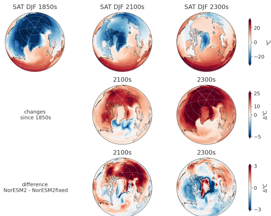
Figure A3. Arctic winter (DJF) surface air temperature. Absolute values 1850, 2100 and 2300 for NorESM2 (top row), changes since the start of the simulation for NorESM2 (second row) and as difference between NorESM2 and NorESM2fixed (third row). To cover differences of the initial climate state in NorESM2 and NorESM2fixed, the last row is calculated as double differences, meaning the difference of changes since the 1850s of the respective simulations.
