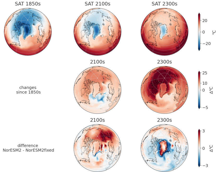
Figure A2. Annual surface air temperature as shown in Fig. 2 on Arctic projection. Absolute values 1850, 2100 and 2300 for NorESM2 (top row), changes since the start of the simulation for NorESM2 (second row) and as difference between NorESM2 and NorESM2fixed (third row). To cover differences of the initial climate state in NorESM2 and NorESM2fixed, the last row is calculated as double differences, meaning the difference of changes since the 1850s of the respective simulations.
