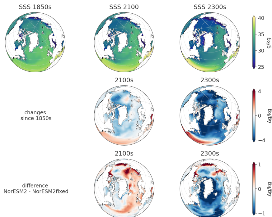
Figure A9. Sea salinity evolution as shown in Fig. 6 on Arctic projection. Absolute values 1850s, 2100s and 2300s for NorESM2 (top row), changes since the start of the simulation for NorESM2 (second row) and as difference between NorESM2 and NorESM2fixed (third row). To cover differences of the initial climate state in NorESM2 and NorESM2fixed, we show double differences here, meaning the difference of the anomaly in 2100s (and 2300s) for NorESM2 and NorESM2fixed.
