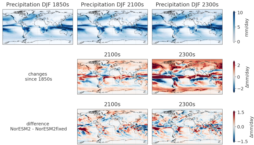
Figure A4. DJF precipitation with absolute values 1850, 2100 and 2300 for NorESM2 (top row), changes since the start of the simulation for NorESM2 (second row) and as difference between NorESM2 and NorESM2fixed (third row). To cover differences of the initial climate state in NorESM2 and NorESM2fixed, the last row is calculated as double differences, meaning the difference of changes since the 1850s of the respective simulations.
