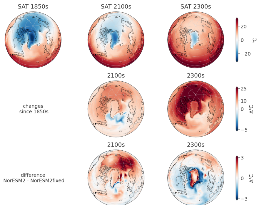
Figure A1. Annual surface air temperature as shown in Fig. 2 on Arctic projection. Absolute values 1850, 2100 and 2300 for NorESM2 (top row), changes since the start of the simulation for NorESM2 (second row) and as difference between NorESM2 and NorESM2fixed (third row). To cover differences of the initial climate state in NorESM2 and NorESM2fixed, the last row is calculated as double differences, meaning the difference of changes since the 1850s of the respective simulations.
