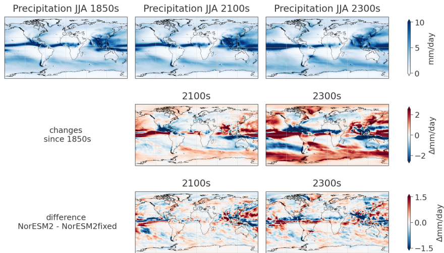
Figure A5. JJA precipitation with absolute values 1850, 2100 and 2300 for NorESM2 (top row), changes since the start of the simulation for NorESM2 (second row) and as difference between NorESM2 and NorESM2fixed (third row). To cover differences of the initial climate state in NorESM2 and NorESM2fixed, the last row is calculated as double differences, meaning the difference of changes since the 1850s of the respective simulations.
