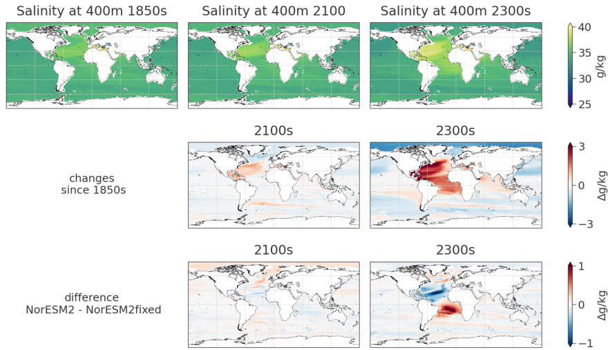
Figure A9. Sea salinity evolution as shown in Fig. 6 on 400 m depth. Absolute values 1850s, 2100s and 2300s for NorESM2 (top row), changes since the start of the simulation for NorESM2 (second row) and as difference between NorESM2 and NorESM2fixed (third row). To cover differences of the initial climate state in NorESM2 and NorESM2fixed, we show double differences here, meaning the difference of the anomaly in 2100s (and 2300s) for NorESM2 and NorESM2fixed.
