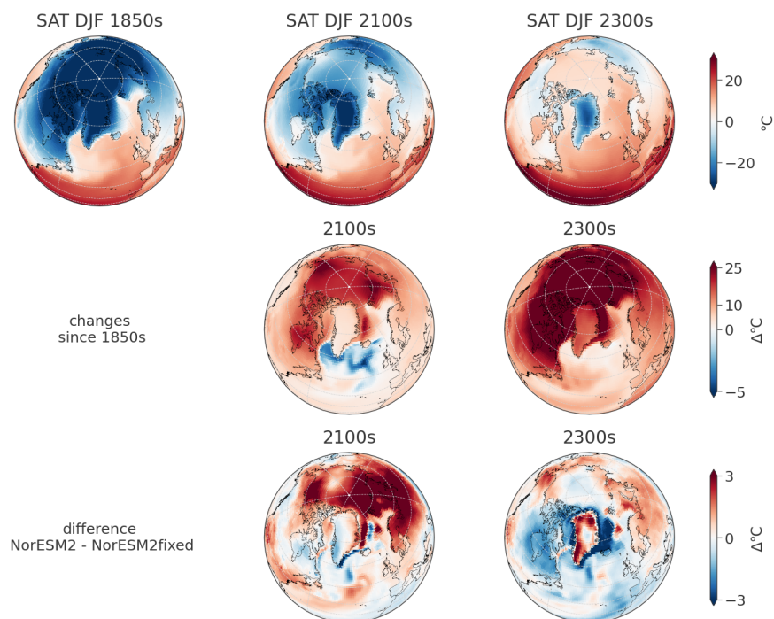
Figure A2. Arctic winter (DJF) surface air temperature. Absolute values 1850, 2100 and 2300 for NorESM2 (top row), changes since the start of the simulation for NorESM2 (second row) and as difference between NorESM2 and NorESM2fixed (third row). To cover differences of the initial climate state in NorESM2 and NorESM2fixed, the last row is calculated as double differences, meaning the difference of changes since the 1850s of the respective simulations.
