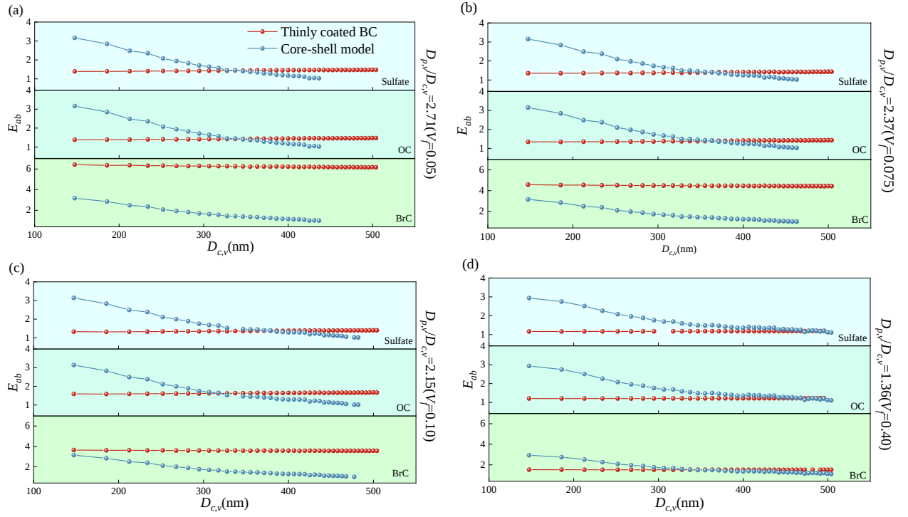
Figure 5. The absorption enhancement of BC thinly coated by different materials with D_f = 1.80 and the corresponding core-shell model. (a) The preset D_{p,v}/D_{c,v} is 2.71; (b) The preset D_{p,v}/D_{c,v} is 2.37; (c) The preset D_{p,v}/D_{c,v} is 2.15; (d) The preset D_{p,v}/D_{c,v} is 1.36.
