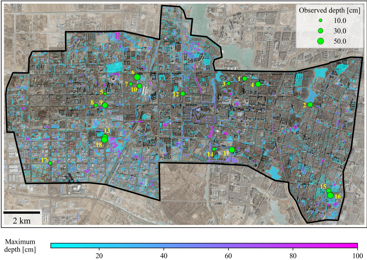
Figure 8. Maximum inundation depth map simulated by the FSR approach under the 20220711-July 2022 storm. Basemaps are derived from ESRI World Imagery (Credit: Esri, TomTom, Garmin, FAO, NOAA, USGS, © OpenStreetMap contributors, and the GIS User Community).
