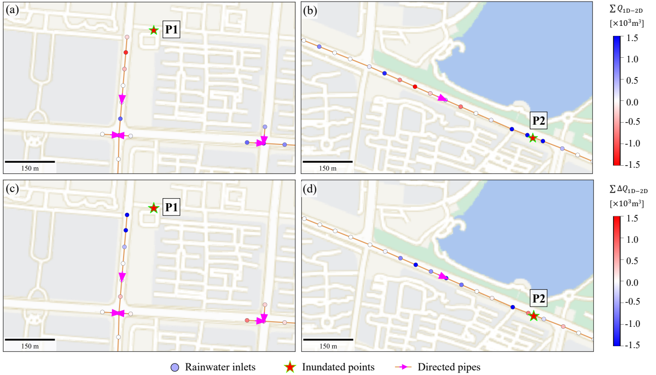
Figure 11. Comparison of accumulated discharges at rainwater inlets during the 20220714 July 2022 storm. (a)-(b) RSN simulated discharges. (c)-(d) Simulated discharge differences between RSN and FSN defined by RSN minus FSN. Basemaps are provided by Tianditu ( https://map.tianditu.gov.cn/ ).
