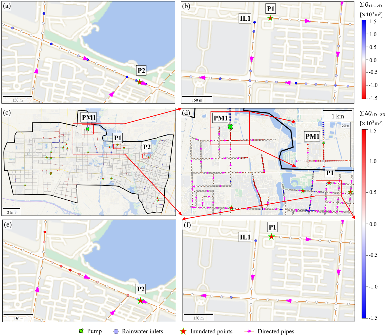
Figure 10. Comparison of accumulated discharges ( \sum Q_{1D-2D} ) at rainwater inlets during the 20220711-July 2022 storm where positive values indicate inflows. (a)-(b). FSN simulated discharges. (c-f) Simulated discharge differences ( \sum \Delta Q_{1D-2D} ) between FSN and FSR defined by FSN minus FSR. Basemaps are provided by Tianditu ( https://map.tianditu.gov.cn/ ).
