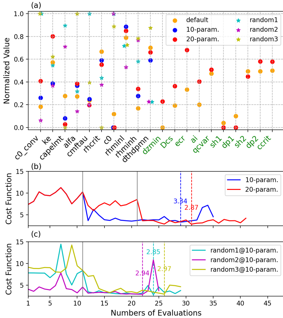
Figure 3. Normalized values of tuning parameters for the default and all five optimized cases (a); changes in the cost function values over iterations-numbers of evaluations for the two main optimized cases (b) and the three sensitivity experiment cases (c). The vertical solid lines indicate the 11 and 21 runs from the initial perturbation phase, while vertical dashed lines mark the iterations at which the cost function reach its minimum.
