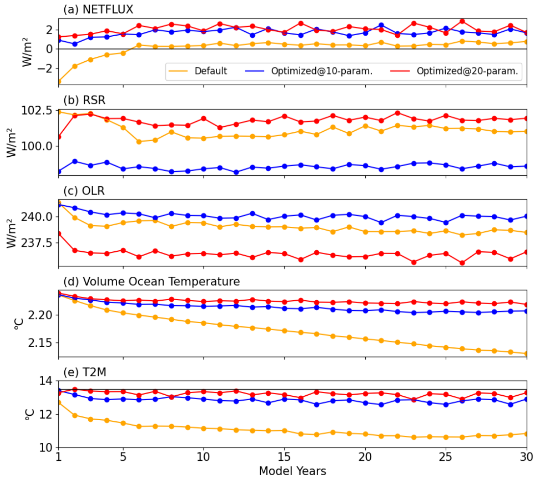
Figure 10. Results from the 30-year piControl simulation for NETFLUX (a), RSR (b) and OLR (c) radiation, mean volume-averaged ocean temperature (d), and T2M in the default (greenorange), 10-parameter (blue), and 20-parameter cases (red) cases.
