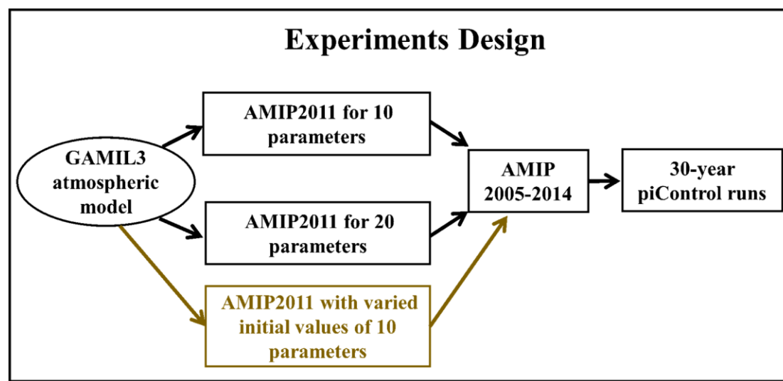
Figure 2. All experiments conducted in this study, including the AMIP2011 optimization runs for 10- and 20-parameter cases, the AMIP2005-2014 simulations using the optimized parameter sets, and the 30-year piControl simulations. Note that piControl simulations were not performed for the sensitivity experiments that varied the initial values of the 10 parameters (shown in brown).
