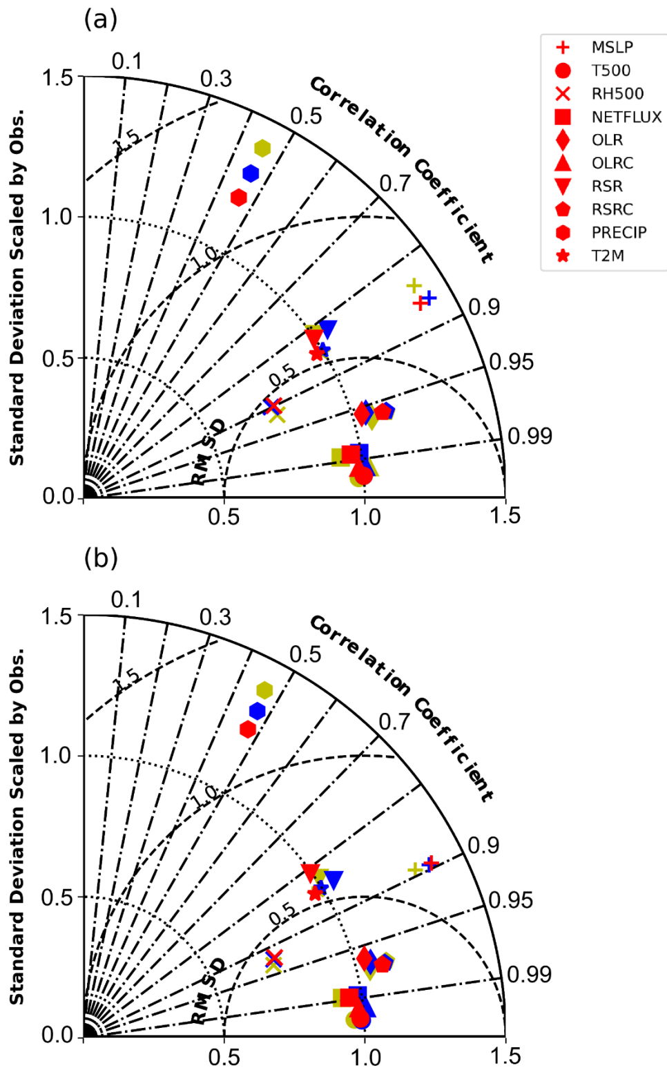
Figure 6. Taylor-diagram showing all variables for three cases in 2011 (a) and the AMIP2005-2014 simulations (b). Shown are default case (greenyellow), 10-parameter case (blue), and 20-parameter case (red).
