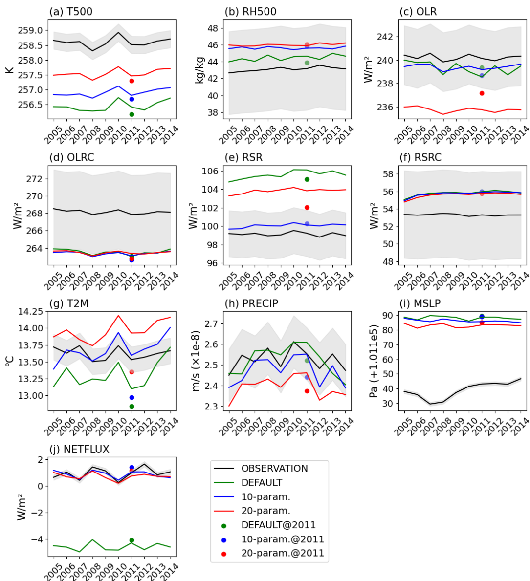
Figure 54. 1-year-AMIP2011 results (dots) and time series (lines) for three cases for: T500 (a), RH500 (b), OLR (c), OLRC (d), RSR (e), RSRC (f), T2M (g), Lprecip PRECIP (h), MSLP (i) and NETFLUX (j). The cases include the default case (green lines and dots), 10-parameter case (blue lines and dots), and 20-parameter case (red lines and dots). The black lines and shadings represent the observations and their associated uncertainties.
