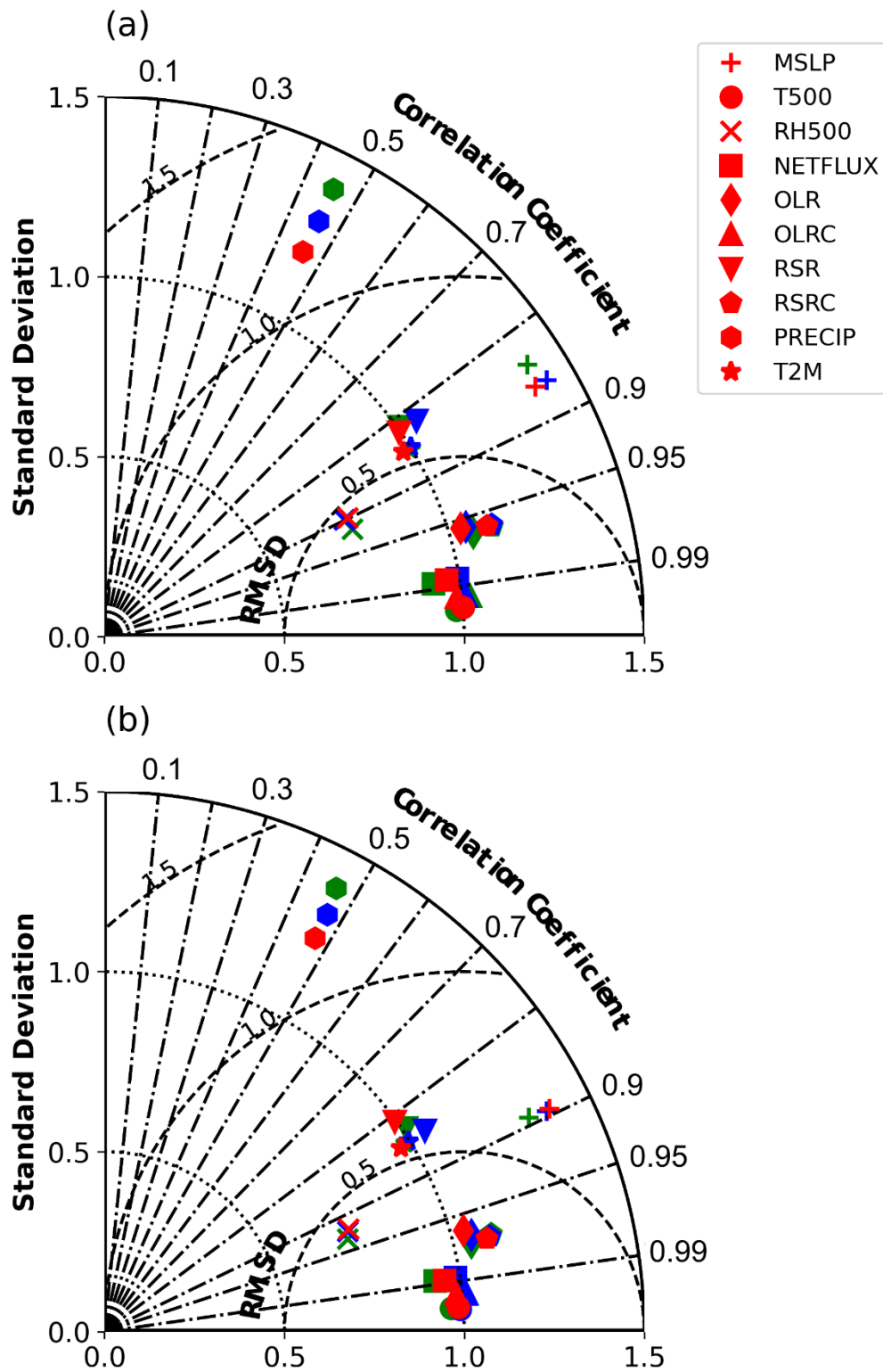
Figure 65. Taylor-diagram showing all variables for three cases in 2011 (a) and the 10-year AMIP2005-2014 simulations (b). Shown are default case (green), 10-parameter case (blue), and 20-parameter case (red).
