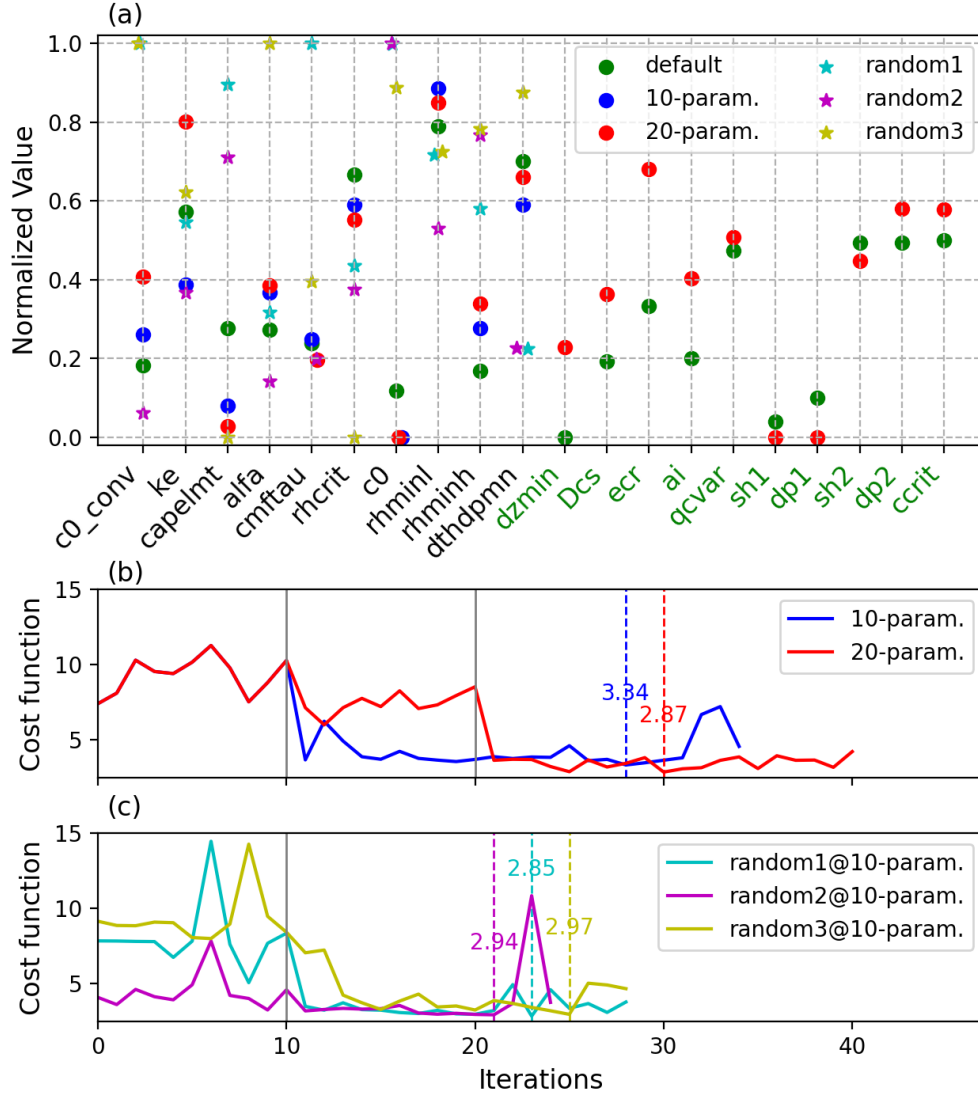
Figure 32. Normalized values of tuning parameters for the default and all five optimized cases (a), along with changes in the cost function values over iterations for the 10- and 20-parameter two main optimized cases (b) and the three sensitivity experiments cases (c). The vertical solid lines indicate the 11 and 21 runs from the initial perturbation phase, while vertical dashed lines mark the iterations at which the cost function reach its minimum.
