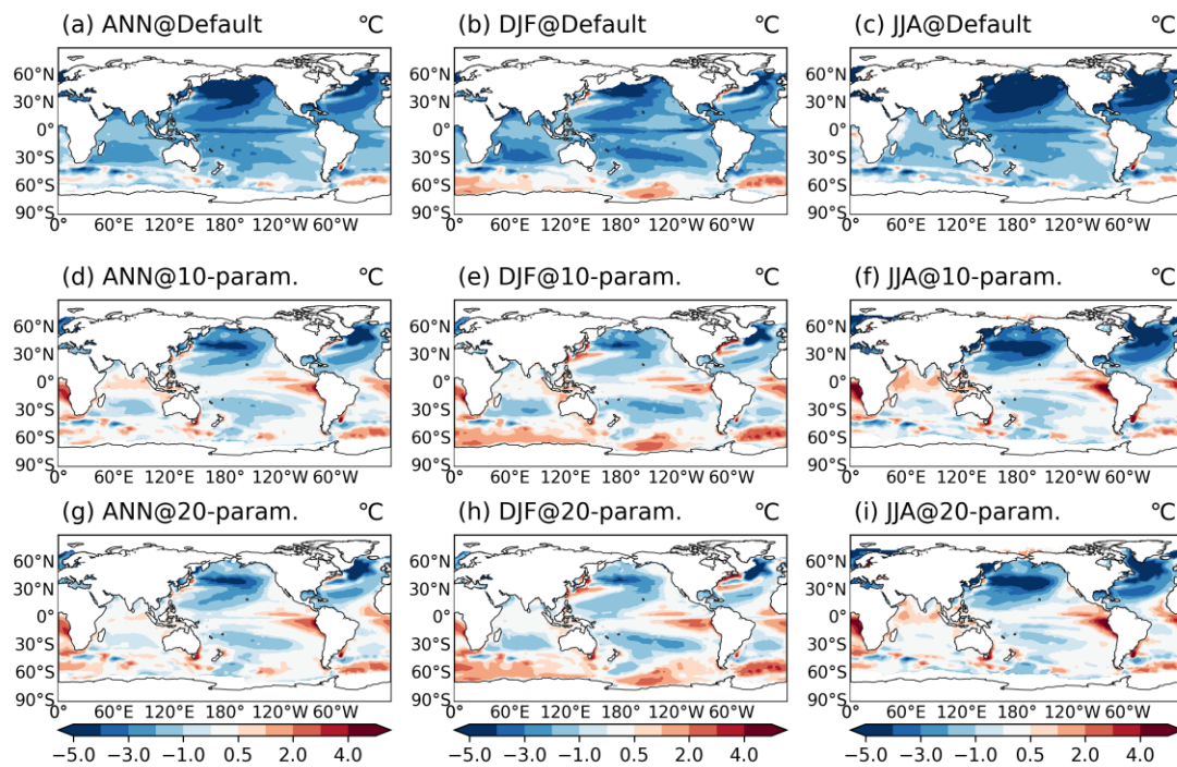
Figure 10. Sea surface temperature biases relative to observations (HadISST; Rayner et al., 2003) from the last 15 years of piControl simulations for the default case (a, b, c) and two optimized cases (d-i).
