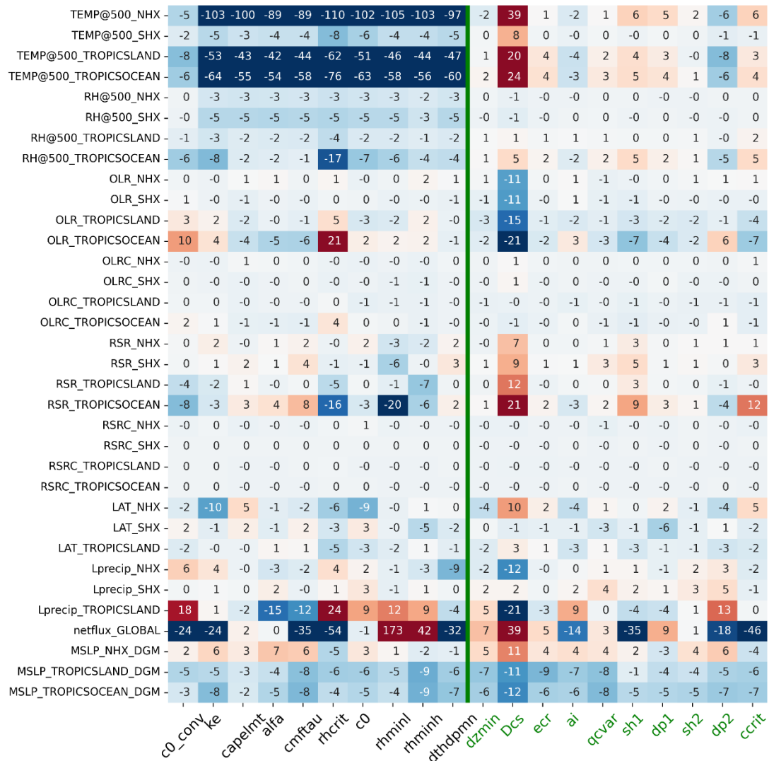
Figure 87. Normalized Jacobian for all 20 parameters, with values normalized by the total covariance metrics. The x-axis shows the parameter names, while the y-axis represents the variables. Black parameters are used in the 10-parameter case, and green ones are added in the 20-parameter case. Red and blue indicate positive and negative effects, respectively, with darker shades showing greater impact.
