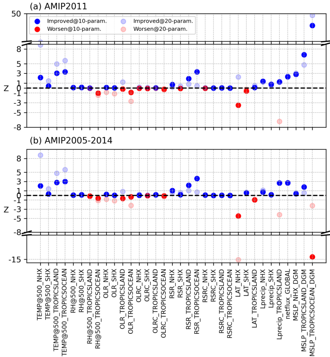
Figure 43. Z values for the 1-year AMIP2011 (a) and 10-year AMIP2005-2014 (b) AMIP simulations. Solid and hollow dots represent tuning with 10 and 20 parameters, respectively. Blue dots indicate improved performance, while red dots show deterioration. The black dashed line at Z = 0 separates improved from non-improved variables.
