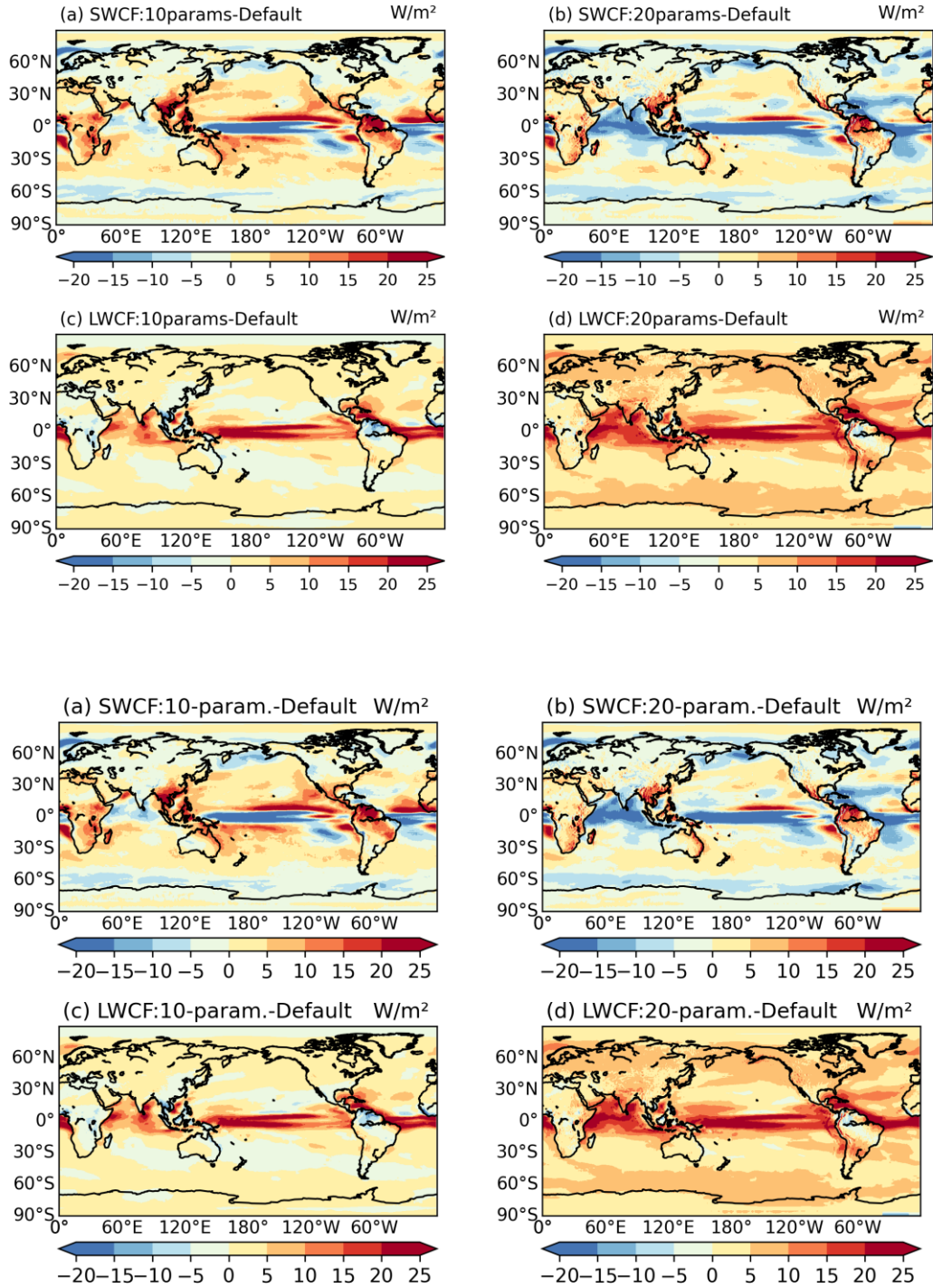
Figure 124. Distribution of shortwave (a, b) and longwave (c, d) cloud forcing differences between the two optimized cases and the default case.
