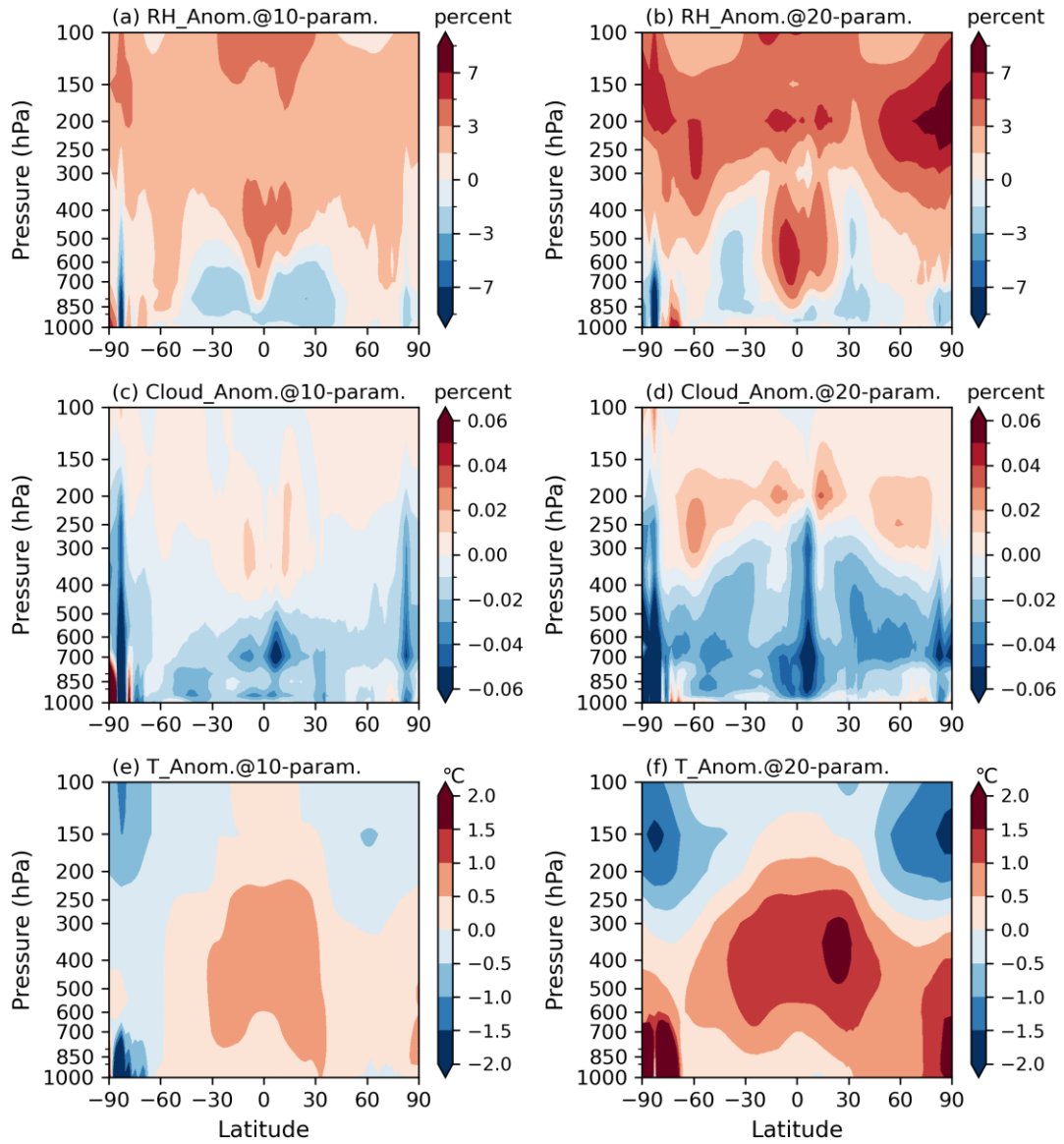
Figure 98. Latitude-pressure anomaly distributions relative to the default case for relative humidity (a, b), cloud fraction (c, d), and temperature (e, f) from 10-year-AMIP2005-2014 simulations: 10-parameter case (a, c, e) and 20-parameter case (b, d, f).
