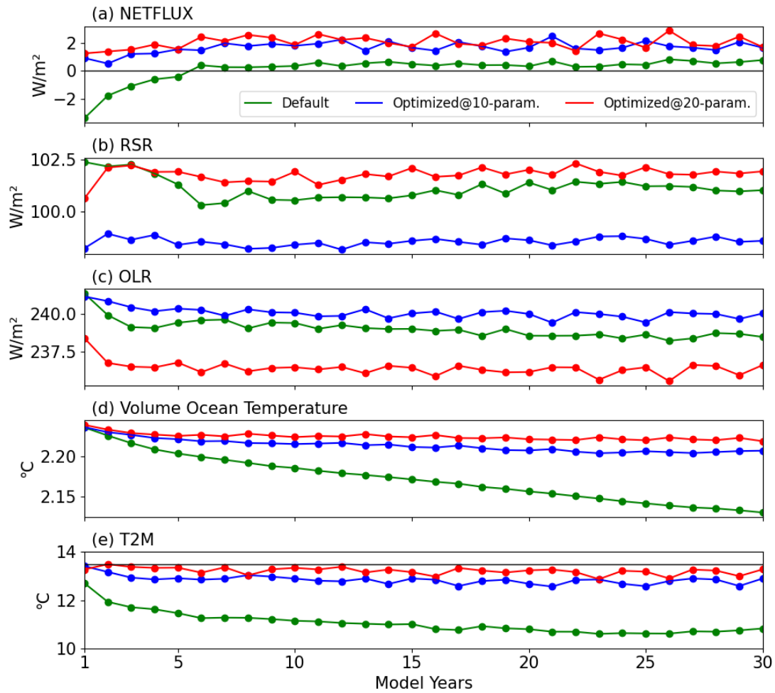
Figure 109. Results from the 30-year piControl simulation for NETFLUX (a), RSR (b) and OLR (c) radiation, mean volume-averaged ocean temperature (d), and T2M in the default (green), 10-parameter (blue), and 20-parameter cases (red) cases.
