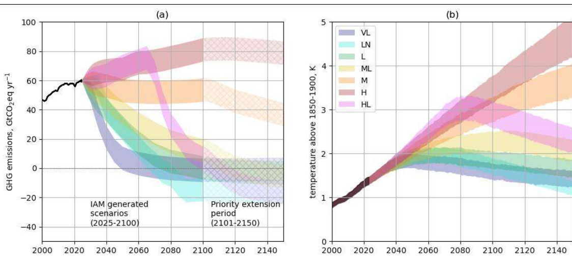
360 Figure 1: Proposed scenarios for CMIP7 ScenarioMIP, showing (a) GHG emissions pathways as a function of time for each of the proposed scenarios (based on GWP-100) and (b) the associated global average temperature outcomes using the probabilistic FaIR ensemble used in IPCC AR6 (41, 42). The shaded area for emissions shows \pm 8 GtCO 2 around the expected marker scenario value while for temperature outcomes, it shows the 33-67 percentile range of the distribution for the same expected marker scenario. Data for the historical period can be found here (43). Scenarios are (H) High , (HL) High-to-Low , (M) Medium , (ML) Medium-to-Low , (L) Low , (LN) Low-to-Negative and (VL) Very Low . The final emission trajectories will depend on the finalized IAM runs but are expected to be roughly consistent with the illustrations provided here. The final temperature outcomes will be known only at completion of Earth system models' experiments, and will, for this phase of ScenarioMIP, include also the effects of carbon cycle feedbacks. Models are requested to run the scenarios for the period 2025-2150; the textured regions for the 2100-2150 period (AD) indicate that these emissions and forcings are defined in the extension protocol. 365
