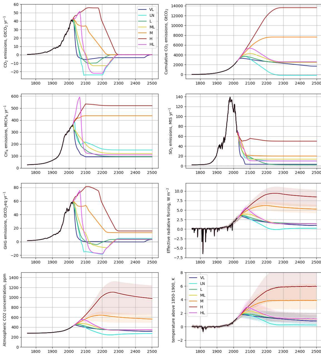
735 Figure 2: Extensions for ScenarioMIP in CMIP7. Top row shows CO 2 emissions and cumulative emissions. Second row shows methane and sulfur dioxide emissions. Third row shows GHG emissions (calculated using GWP100) and total radiative forcing. Fourth row shows atmospheric CO 2 concentrations and projected temperature outcomes. Simulations are conducted with a calibrated ensemble of the FaIR simple climate model (41, 42), where solid lines show the 50th percentile outcome and shaded regions show the 5-95 percentile range. Data for the historical period is based on (43). Scenarios are (H) High, (HL) High-to-Low, (M) Medium, (ML) Medium-to-Low, (L) Low, (LN) Low-to-Negative and (VL) Very Low. The final emission trajectories will depend on 740 the finalized IAM runs but are expected to be consistent with the illustrations provided here.
