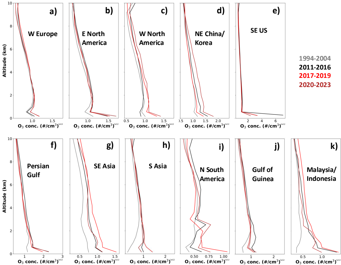
Figure 2: Ozone concentration profiles in the 11 regions listed in Tab. 1, averaged over the periods 1994-2004 (grey lines), 2011-2016 (black lines), 2017-2019 (red lines) and 2020-2023 (dark red lines).
