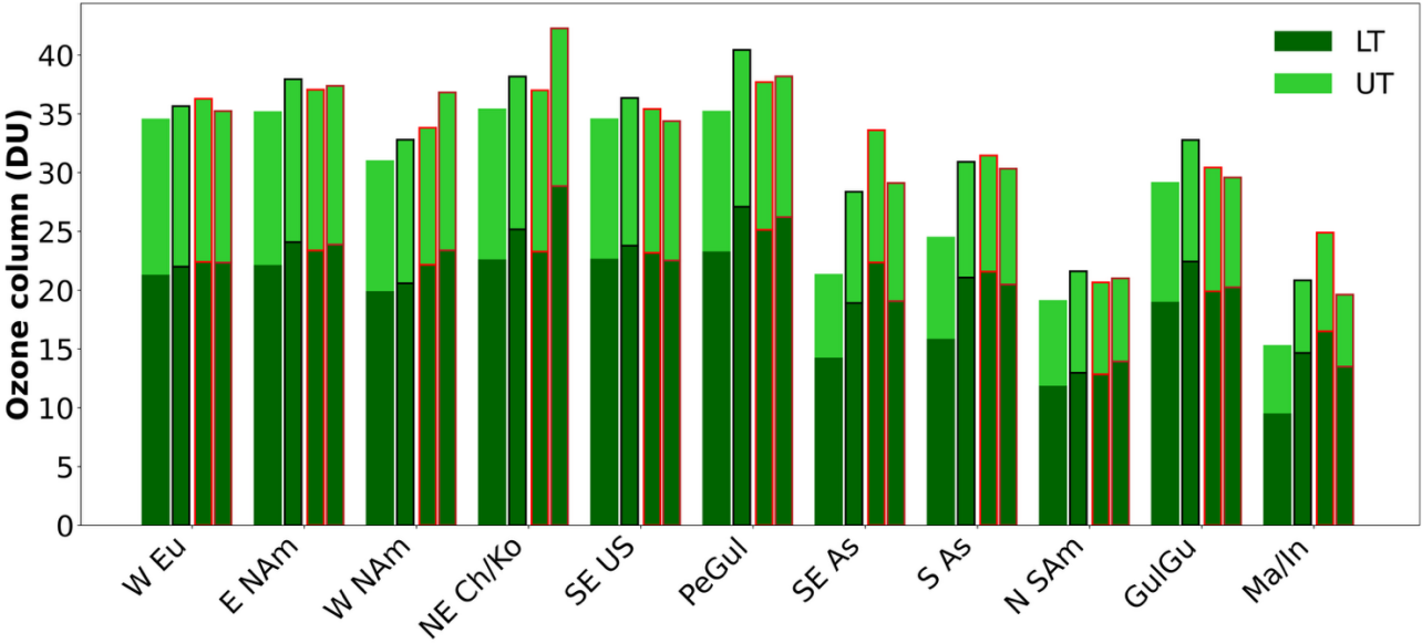
Figure 3: Average LT (dark green bars) and UT ozone columns (stacked light green bars) in the periods 1994-2004 (large bars on the left without borders), 2011-2016 (bars with black borders), 2017-2019 (bars with red borders) and 2020-2023 (bars with dark red border) for each of the 11 regions listed in Tab. 1.
