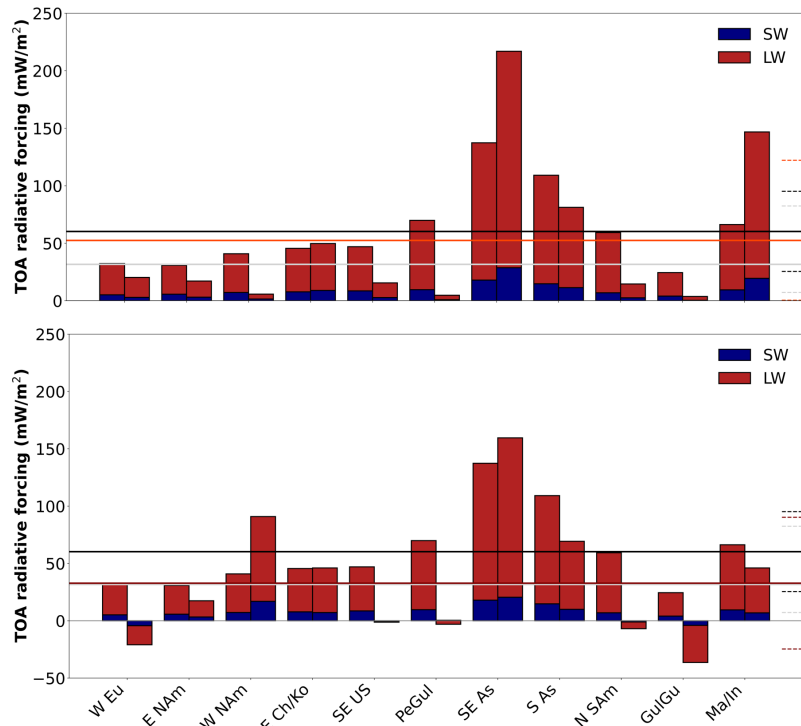
230 Figure 5: SW (blue bars) and LW (stacked red bars) decadal tropospheric ozone instantaneous RF, for each of the 11 regions listed in Tab. 1, for the periods 2011-2016 (bars on the left in panels a and b), 2017-2019 (bars on the right in panel a) and 2020-2023 (bars on the right in panel b), with respect to the period 1994-2004. Horizontal lines represent the overall 2011-2016 (solid black line in panels a and b), 2017-2019 (solid red line in panel a) and 2020-2023 (solid dark red line in panel b) averages, and the global average RF of Skeie et al. (2020) scaled to 14.5 years (solid grey line). Horizontal dotted lines represent the uncertainty range of respective solid lines. 235
