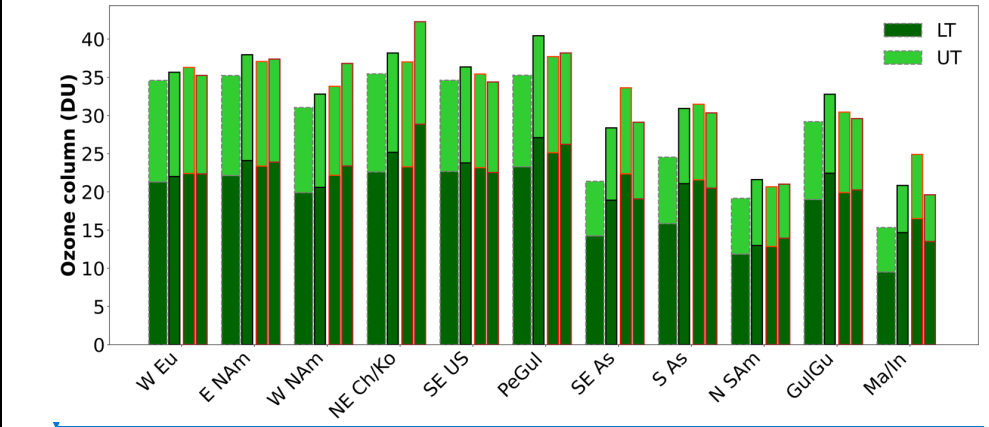
Figure 3: Average LT (dark green bars) and UT ozone columns (stacked light green bars) in the periods 1994-2004 (large bars on the left dashed grey borders), 2011-2016 (bars with black borders), 2017-2019 (bars with red borders) and 2020-2023 (bars with dark red border) for each of the 11 regions listed in Tab. 1.
