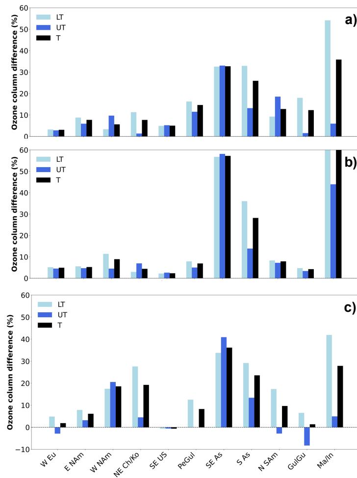
Figure 4: LT (sky blue bars), UT (blue bars) and total tropospheric ozone percent difference (black bars), for each of the 11 regions listed in Tab. 1 for the periods 2011-2016 (panel a), 2017-2019 (panel b) and 2020-2023 (panel c) with respect to the period 1994-2004.
