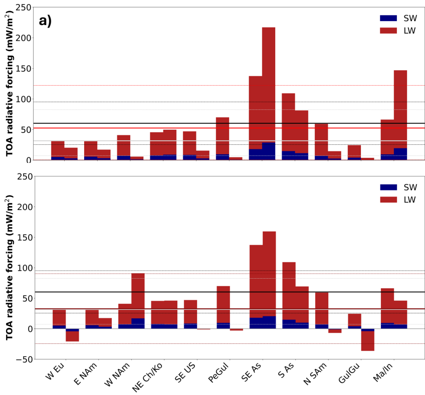
Figure 5: SW (blue bars) and LW (stacked red bars) decadal tropospheric ozone instantaneous RF, for each of the 11 regions listed in Tab. 1, for the periods 2011-2016 (bars on the left in panels a and b), 2017-2019 (bars on the right in panel a) and 2020-2023 (bars on the right in panel b), with respect to the period 1994-2004. Horizontal lines represent the overall 2011-2016 (solid black line in panels a and b), 2017-2019 (solid red line in panel a) and 2020-2023 (solid dark red line in panel b) averages, and the global average RF of Skeie et al. (2020) scaled to 14.5 years (solid grey line). Horizontal dotted lines represent the uncertainty range of respective solid lines.
