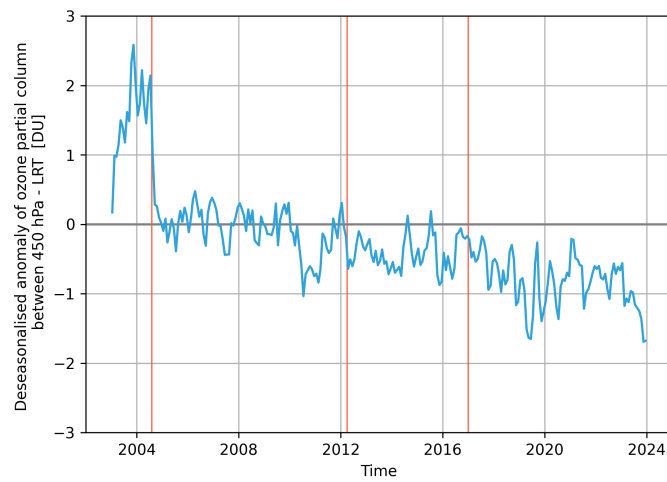
Figure 1. Difference (blue) between the derived climatology (2004-2016) and full reanalysis CAMS correction terms for going from the 450 hPa top level tropospheric column to the lapse-rate tropopause column. Vertical lines (red) indicate important changes in the CAMS assimilation system as detailed in Inness et al. (2019).
