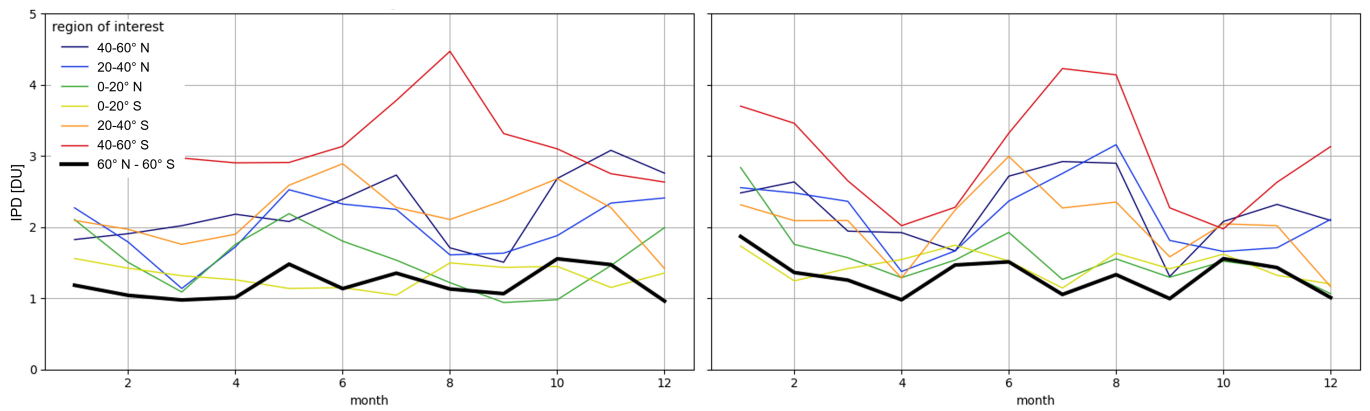
Figure 12. Zonal and near-global (60° N to 60° S) seasonal cycles of the IPD [DU] for the full time series of all sixteen satellite data records, both before (left) and after (right) harmonisation. Note that the latter is limited to the CAMSRA temporal domain (2003-2023).
