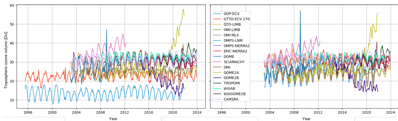
Figure 10. Near-global (60° N to 60° S) tropospheric ozone column time series for all sixteen satellite data records and CAMSRA, both before (left) and after (right) harmonisation. Note that the latter is limited to the CAMSRA temporal domain (2003-2023).
