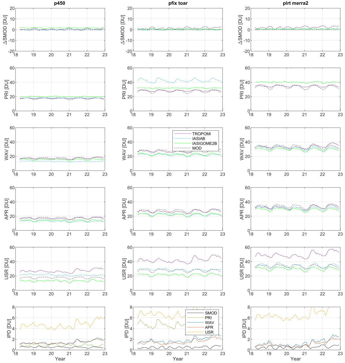
Figure 4. Same as Fig. 3 but for the overlapping period (May 2018 to December 2022) of TROPOMI (purple), IASI-AB (blue), and IASI+GOME-2B (green), restricted to their common spatiotemporal sampling. Note that the IASI-AB PRI data is just above 60 DU for the lapse-rate tropopause definition (third column).
