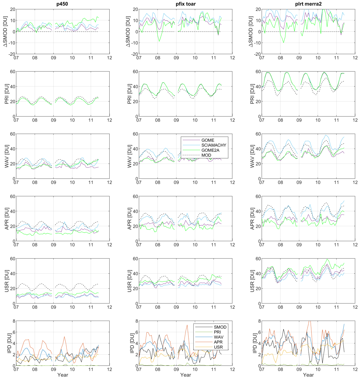
Figure 3. Evaluation of nadir ozone profile harmonisation for the overlapping period (January 2007 to June 2011) of GOME (purple), SCIAMACHY (blue), and GOME-2A (green), restricted to their common spatiotemporal sampling. The first row shows the difference between the CAMSRA model data (black dashed lines) before and after averaging kernel smoothing. The second to fifth rows contain global mean tropospheric ozone time series for the prior profile columns (PRI), weighted-averaged retrieved columns (WAV), harmonised columns using a-priori profile replacement (APR), and columns in their unit-sensitivity representation (USR), respectively, all in DU. The last row depicts the IPD [DU] for each of the rows above. The PRI dispersion here roughly equals zero as all three products result from essentially the same RAL algorithm and prior input. The three columns correspond to the three selected tropospheric top level definitions.
