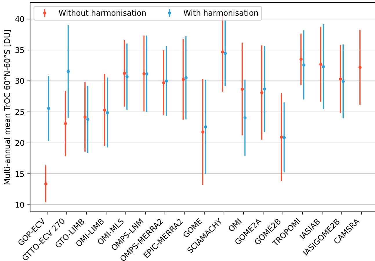
Figure 9. Near-global (60° N to 60° S) multi-annual mean tropospheric ozone columns (TrOC) and dispersions before (red) and after (blue) harmonisation for all sixteen satellite data products and CAMSRA, over their full time series. The GTTO-ECV dataset covers 20° N to 20° S and is not directly comparable to the near-global mean of the other datasets.
