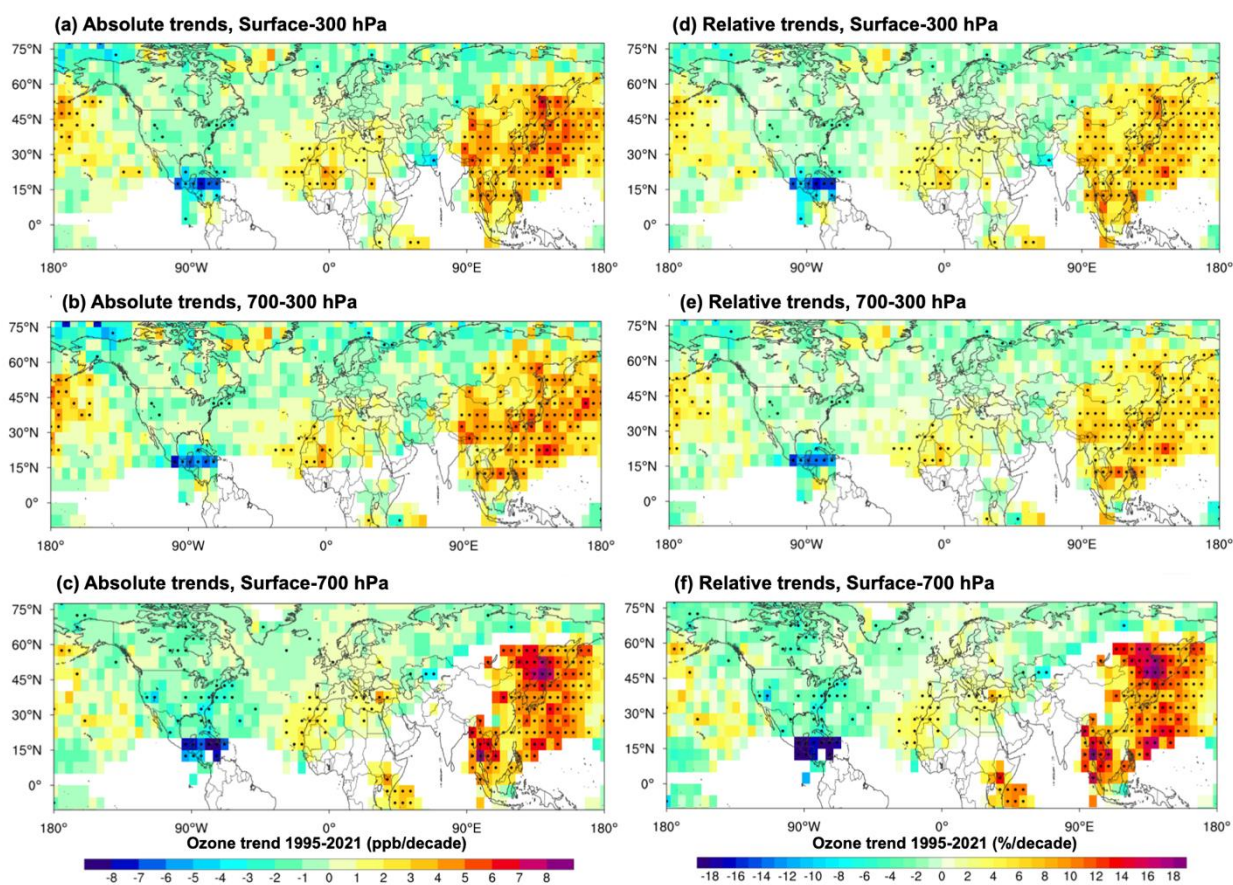
395 Figure 5: (a-c) TOST-based trends (in ppb/decade) of the mean ozone mixing ratios over the columns from the surface to 300 hPa, TrOC (a), from 700 to 300 hPa, FTOC (b) and from surface to 700 hPa, LTOC (c) in the Northern Hemisphere during 1995-2021. (d-f) The same as (a-c), but for relative trends (in %/decade). The statistics are based on QR median value of ozone mixing ratios in each grid cell over 1990-2021. Significant trends are shown by a black dot in the grid cell.
