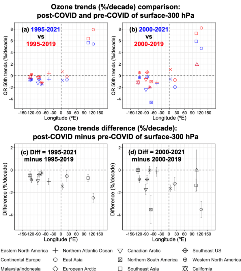
480 Figure 9: (a) TOST QR median trends (in %/decade) of the mean ozone mixing ratio from surface-300 hPa varying with longitude, for the periods 1995-2021 and 1995-2019. The shapes denote the different regions. (b) The same as (a), but for the periods 2000-2021 and 2000-2019. (c) The difference in QR median trends between the periods 1995-2021 and 1995-2019. Error bars represent the 95% confidence interval for the QR median trend difference. (d) The same as (c), but now between the periods of 2000-2021 and 2000-2019. A version of this figure for the absolute trends (in ppb/decade) is available in Fig. S4.
