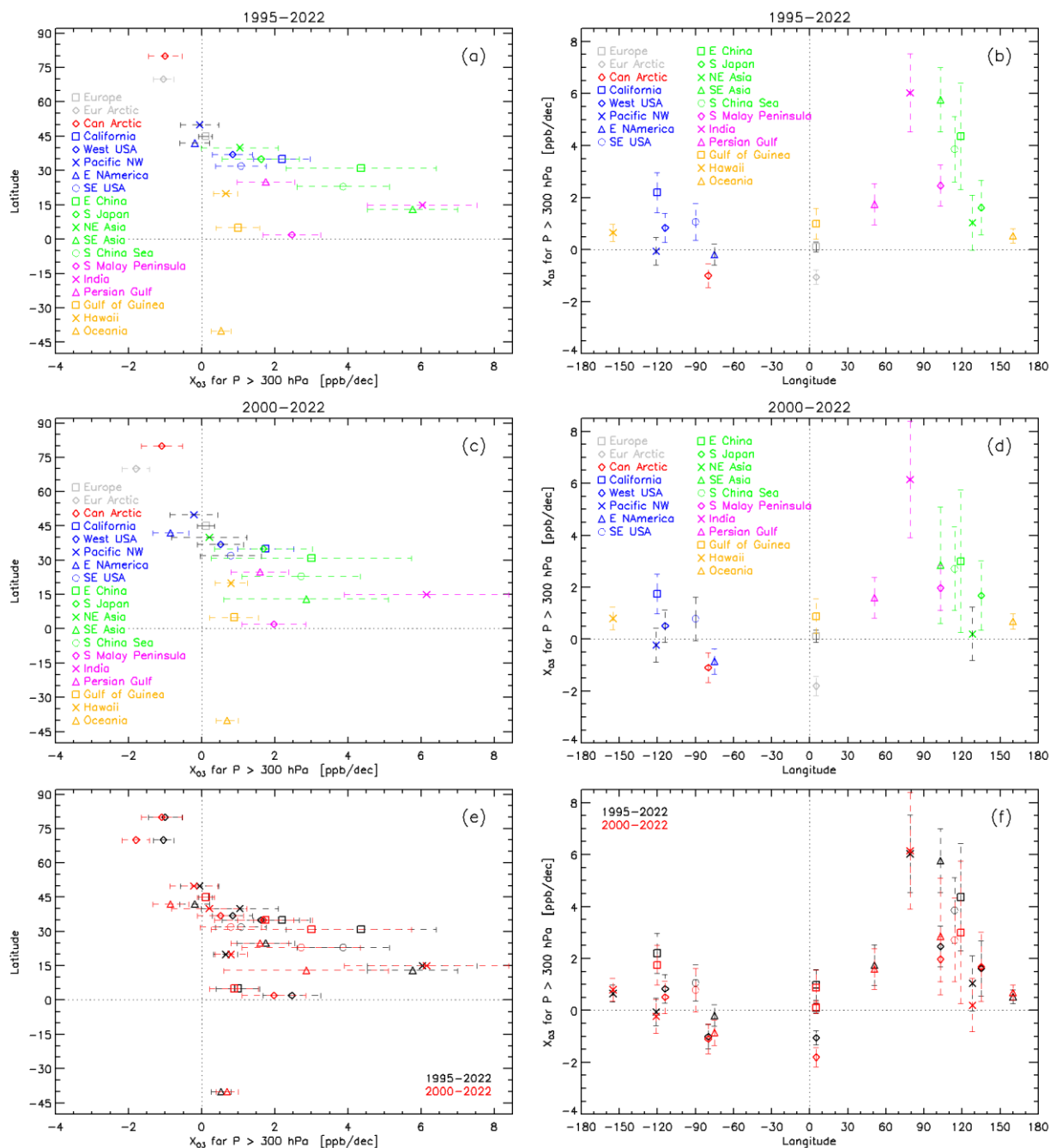
495 Figure 10: Upper panels: LMM TrOC synthesized 1995-2022 trends versus latitude (left) and longitude (right), calculated for the different regions, including only sites that have at least 30 monthly values. The regions are denoted by different symbols and colours for the trend values, and the error bars denote the 2-sigma uncertainties. If those 95% uncertainty ranges are in the same colour as the symbol of the trend value itself, the p-value of the trend is lower than 0.05; if shown in black, the p-value is higher than 0.05. Middle panels: same as in upper panels, but now for the 2000-2022 period. Lower panels: the LMM TrOC synthesized trends of the upper panels are shown now in black, and are compared with the LMM TrOC trends of the middle panels (in red).
