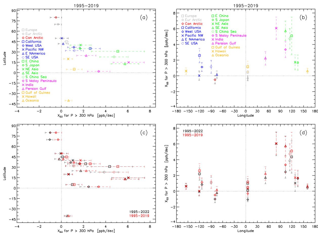
605 Figure 12: Upper panels: Same as in upper panels of Fig. 10, but now for the TrOC trends for the 1995-2019 time period, hence excluding the period where restrictions have been applied to cope with the COVID-19 spread. Lower panels: the synthesized trends of the upper panel are shown now in red, and are compared with the TrOC trends for the time period 1995-2022 (in black).
