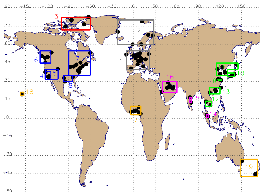
305 Figure 3: Map showing the 19 different regions and the individual HEGIFTOM ground-based sites (see Tables 1 and S1) that are used for the regional synthesized trends calculation using the linear mixed-effects modelling (LMM) approach.
