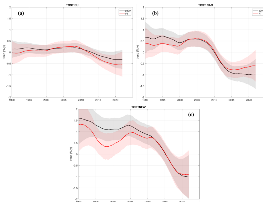
445 Figure 8: DLM trends (%/yr) for both the TrOC (black) and FTOC (red) for the TOST regional time series in Europe (a), North Atlantic Ocean (b), and Northeast Asia (c). Shaded areas represent the 2\sigma uncertainties.
