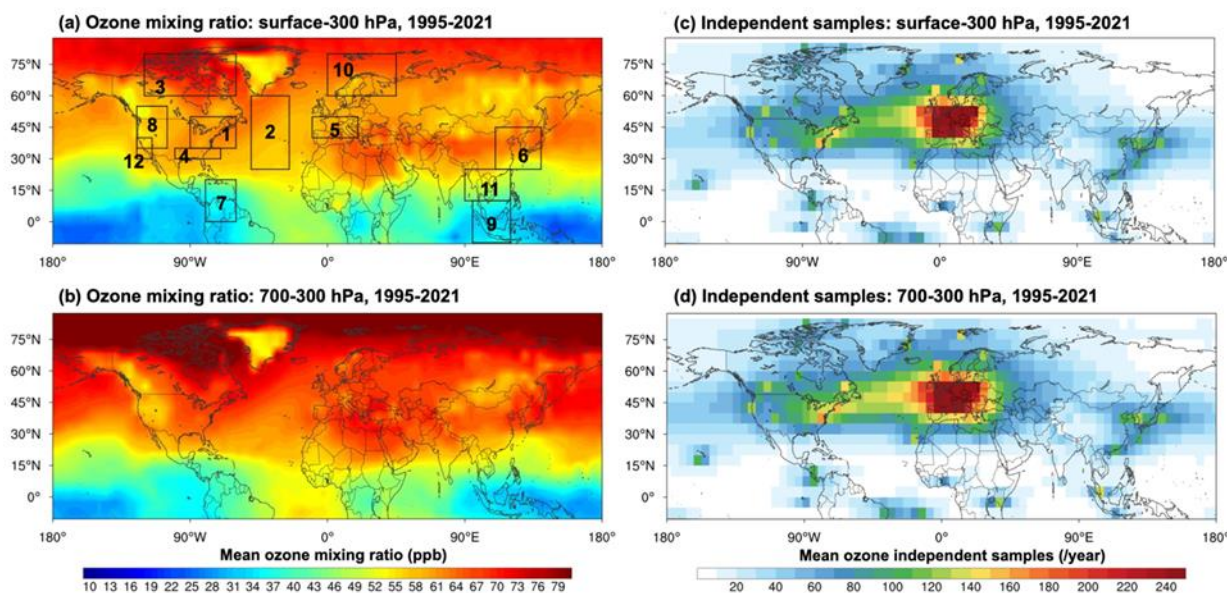
360 Figure 4: (a, b) TOST-based spatial distributions of the mean ozone mixing ratios over the columns from the surface to 300 hPa (a) and of 700 to 300 hPa (b) during 1995-2021. (c-d) The same as (a-b), but for the corresponding mean independent samples. The boxes and ID numbers in (a) denote 12 regions for trend analysis (see Table 3 for the extent of each region).
