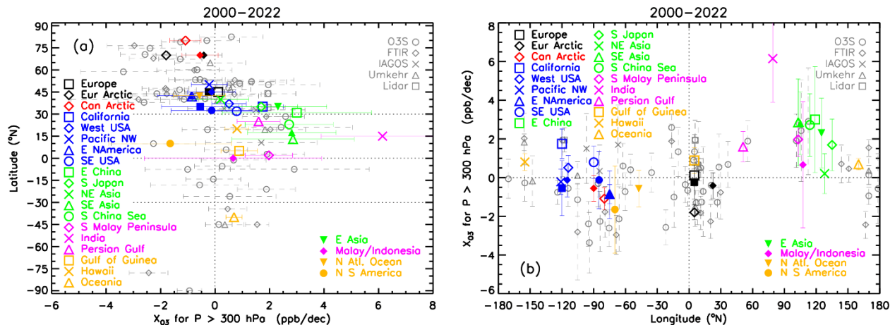
Figure 13: All 2000-2022 TrOC trends [ppb/dec] estimated from the homogenized ground-based and in-situ HEGIFTOM measurements. In grey: the individual site trend estimates from Van Malderen et al. (2025), with different symbols for the different techniques. Open colored symbols denote the LMM trend estimates for the different regions, marked with the different colours in the upper left legends in the plot. The closed symbols represent the TOST regional trend estimates, using the same colour coding for the common regions as for the LMM. Non-overlapping TOST regions are identified in the lower left legends in the plots.
