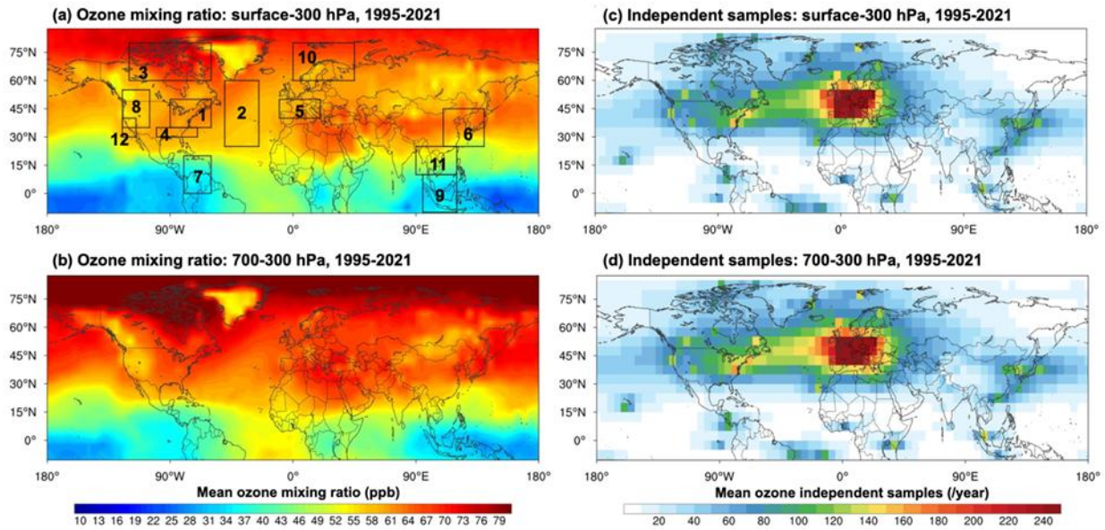
380 Figure 4: (a, b) TOST-based spatial distributions of the mean ozone mixing ratios over the columns from the surface to 300 hPa (a) and of 700 to 300 hPa (b) during 1995-2021. (c-d) The same as (a-b), but for the corresponding mean independent samples. The boxes and ID numbers in (a) denote 12 regions for trend analysis (see Table 3 for the extent of each region).
