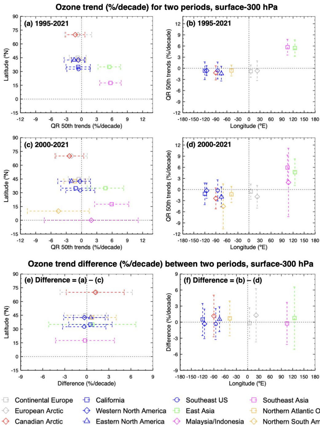
Figure 6: (a, b) TOST QR median trends (in %/decade) of the mean ozone mixing ratios from surface-300 hPa varying with latitude (left, a) and longitude (right, b), for the period of 1995-2021. Error bars represent the 95% confidence interval of the QR trend. Colors denote the regions. (c, d) The same as for (a, b), but for the period of 2000-2021. (e, f) The difference in the QR median trend between the periods of 1995-2021 and 2000-2021. Error bars represent the 95% confidence interval for the QR median trend difference.
