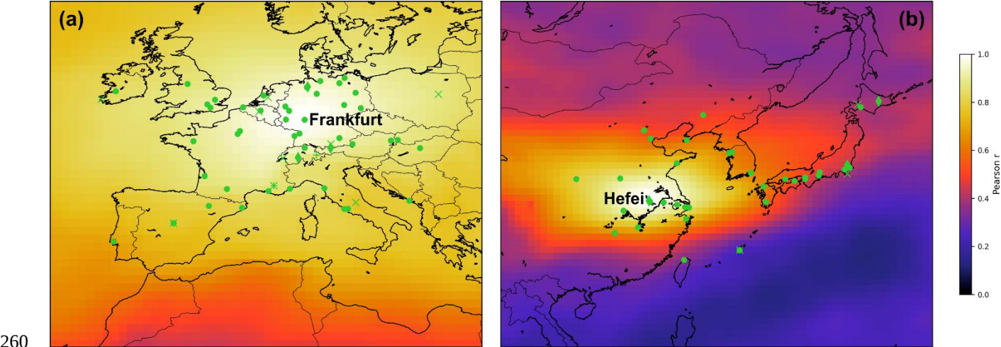
Figure 1: (a) Correlation map at the IAGOS FRA (Frankfurt) airport location, constructed by calculating the linear Pearson correlation coefficients between the CAMS TrOC monthly anomaly grid point at the IAGOS FRA airport location and the CAMS TrOC monthly anomaly grid points in the European domain. (b) Same as (a), but now for the FTOC at the FTIR Hefei location in
