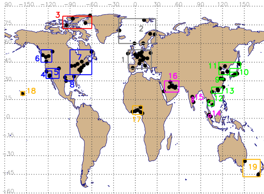
Figure 3: Map showing the 19 different regions (squares, numbered) and the individual HEGIFTOM ground-based sites (black dots) that are used for the regional synthesized trends calculation using the linear mixed-effects modelling (LMM) approach. An overview of those different regions and included HEGIFTOM sites is given in Tables 1 and S1.
