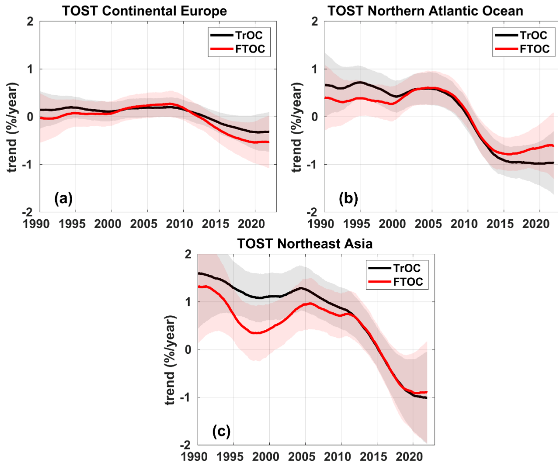
Figure 8: DLM trends (%/yr) for both the TrOC (black) and FTOC (red) for the TOST regional time series in Europe (a), North Atlantic Ocean (b), and Northeast Asia (c). Shaded areas represent the 2\sigma uncertainties.
