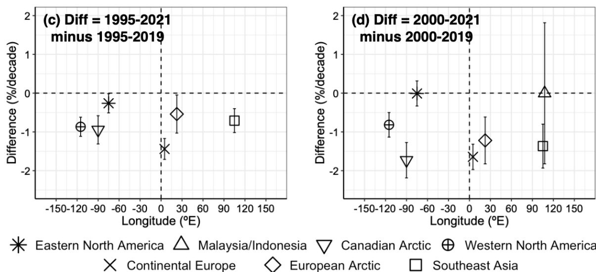
Figure 9: (a) TOST QR median trends (in %/decade) of the mean ozone mixing ratio from surface-300 hPa varying with longitude, for the periods 1995-2021 and 1995-2019. The shapes denote the different regions. (b) The same as (a), but for the periods 2000-2021 and 2000-2019. (c) The difference in QR median trends between the periods 1995-2021 and 1995-2019. Error bars represent the 95% confidence interval for the QR median trend difference. (d) The same as (c), but now between the periods of 2000-2021 and 2000-2019. A version of this figure for the absolute trends (in ppb/decade) is available in Fig. S4.
