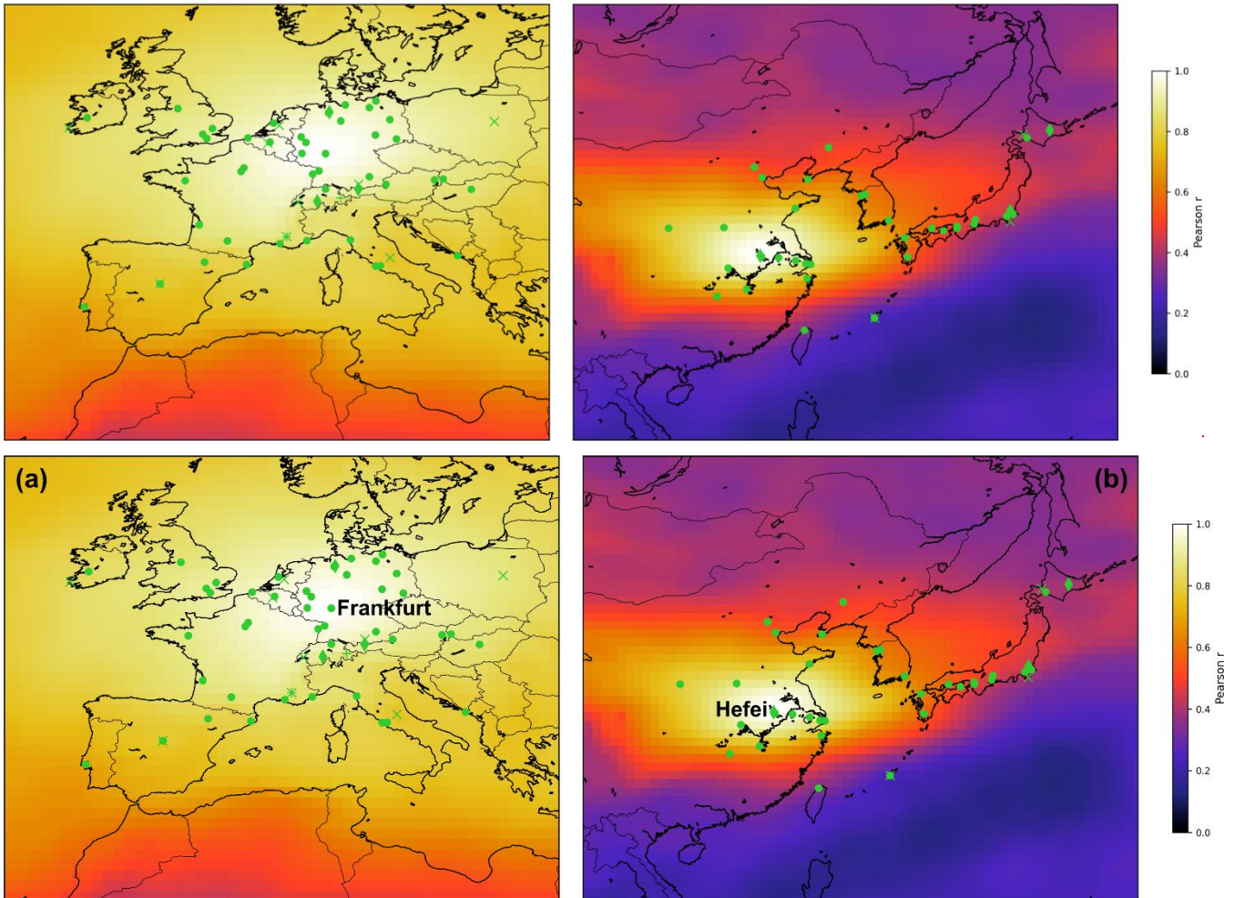
Figure 1: (a) Correlation map at the IAGOS FRA ( Frankfurt ) airport location, constructed by calculating the linear Pearson correlation coefficients between the CAMS TrOC monthly anomaly grid point at the IAGOS FRA airport location and the CAMS TrOC monthly anomaly grid points in the European domain. (b) Same as (a), but now for the FTOC at the FTIR Hefei location in East China. The different HEGIFTOM sites are marked with green symbols, with dots for IAGOS, \times for ozonesondes, diamonds for FTIR, plus for Umkehr, squares for L idar.
