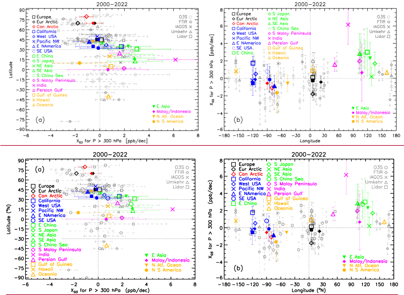
Figure 13: All 2000-2022 TrOC trends [ppb/dec] estimated from the homogenized ground-based and in-situ HEGIFTOM measurements. In grey: the individual site trend estimates from Van Malderen et al. (2025), with different symbols for the different techniques. Open colored symbols denote the LMM trend estimates for the different regions, marked with the different colours in the upper left legends in the plot. The closed symbols represent the TOST regional trend estimates, using the same colour coding for the common regions as for the LMM. Non-overlapping TOST regions are identified in the lower left legends in the plots.
