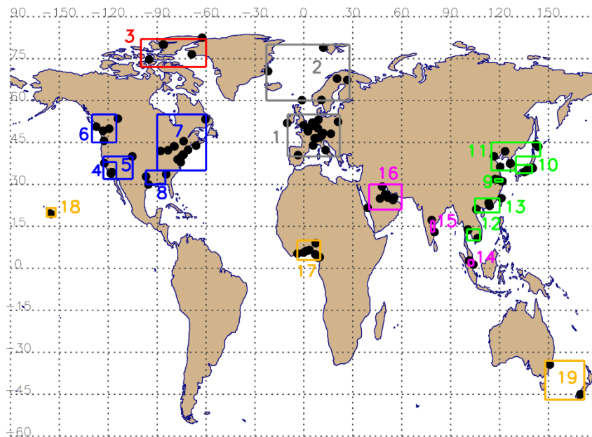
Figure 3: Map showing the 19 different regions ( squares, numbered ) and the individual HEGIFTOM ground-based sites ( black dots ) see Tables 1 and S1 that are used for the regional synthesized trends calculation using the linear mixed-effects modelling (LMM) approach. An overview of those different regions and included HEGIFTOM sites is given in Tables 1 and S1.
