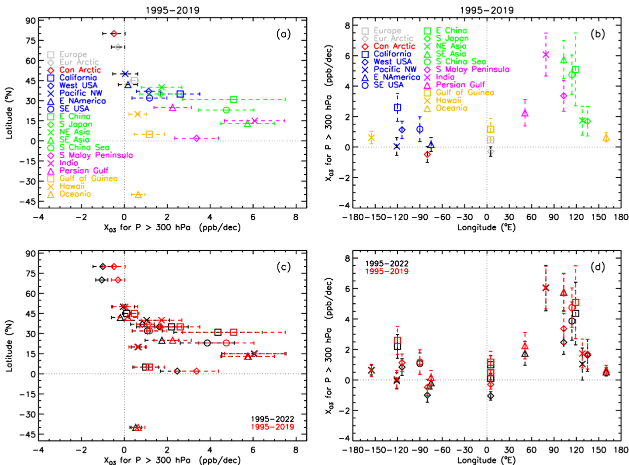
675 Figure 12: Upper panels: Same as in upper panels of Fig. 10, but now for the TrOC trends for the 1995-2019 time period, hence 680 excluding the period where restrictions have been applied to cope with the COVID-19 spread. Lower panels: the synthesized trends of the upper panel are shown now in red, and are compared with the TrOC trends for the time period 1995-2022 (in black).
