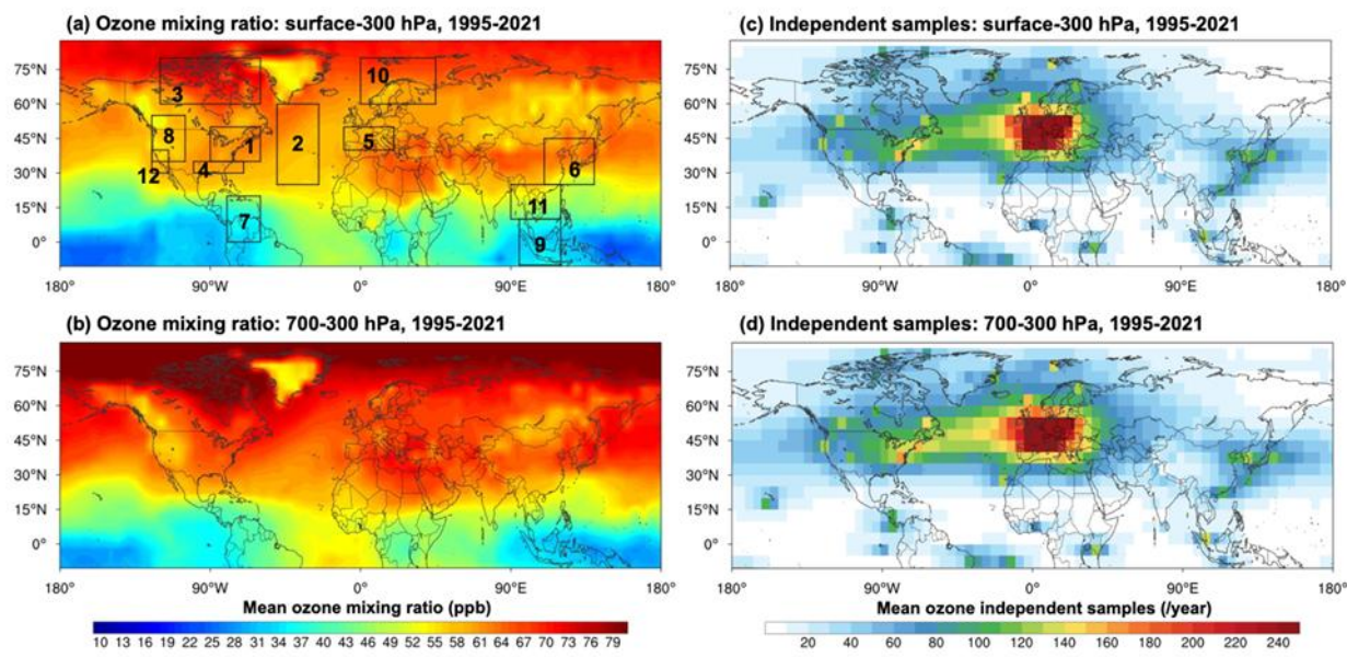
Figure 4: (a, b) TOST-based spatial distributions of the mean ozone mixing ratios over the columns from the surface to 300 hPa (a) and of 700 to 300 hPa (b) during 1995-2021. (c-d) The same as (a-b), but for the corresponding mean independent samples. The boxes and ID numbers in (a) denote 12 regions for trend analysis (see Table 3 for the extent of each region).
