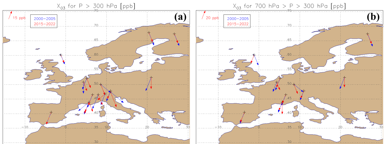
Figure S4: Close-up of Fig. 6 for Europe.
