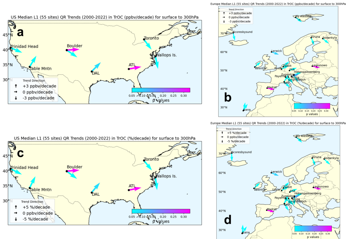
25 Figure S5. Close-up of trends at stations within highly-sampled regions: (a) US; (b) Europe. Multiple arrows correspond to multi-instrument sites, Boulder in (a), OHP and Izaña in (b). (c) Trend same as (a) except in %/decade with p-values; (d) same as (b) except in %/decade with p-values.
