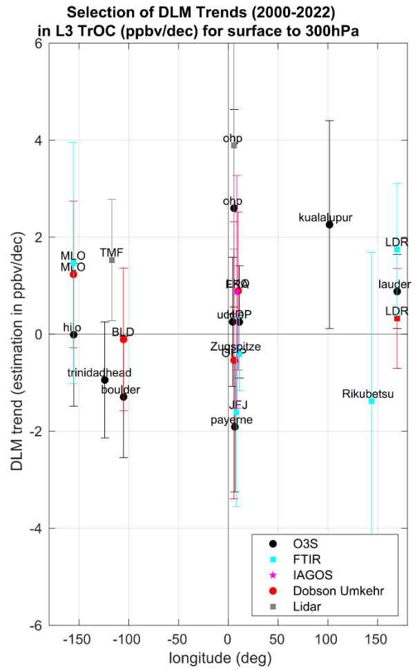
40 Figure S6: DLM trend estimates (ppbv/dec), based on the monthly mean time series for a subset of sites from our sample. DLM trend values are output in ppbv/year. In order to compare DLM trend values with QR and MLR decadal trend values, we need to give an estimate of the trend in ppbv/dec. DLM outputs a distribution of ozone change between the beginning and the end of the considered time period and the trend values in ppbv/dec are determined in ratio. The uncertainty on these values is determined by Monte-Carlo simulations. Assuming the distribution to be normal, we estimate the standard deviation of the trends values from the FWHM of the distribution.
