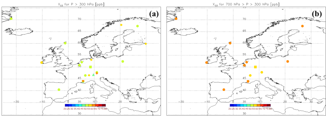
Figure S2: Close-up of Fig. 4: mean (a) TrOC (ppb, surface to 300 hPa), (b) FTOC (ppb, 700>p>to 300 hPa) at European HEGIFTOM sites with at least 120 monthly values in the 2000-2022 period. Circles denote ozonesondes, squares = IAGOS airports, diamonds=FTIR, upward triangles=Umkehr, downward triangles=lidar.
