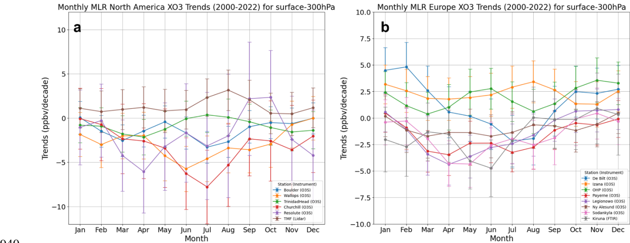
Figure A1: Monthly mean TrOC trends computed with MLR for sites with high confidence ( p<0.05 ) annual MLR trends (a) North America (b) Europe.
