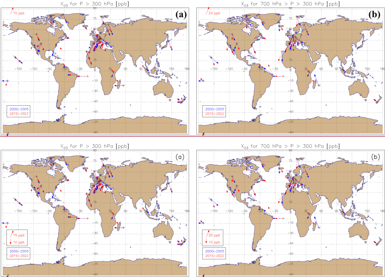
Figure 6: Illustration of the mean seasonal cycle for the TrOC (a) and FTOC (b) time series for two different periods: 2000-2005 (blue) and 2015-2022 (red). The amplitude of the seasonal cycle, defined as the difference between the maximum and minimum long-term monthly mean, is represented by the length of the arrow (with unit shown in the legend in the upper left of the plots). The phase of the seasonal cycle, defined here as the month with the maximum long-term monthly mean value, is denoted by the direction of the arrow as in a clock: 1h = phase or maximum long-term monthly mean in January, 2h = February, 3h = March, etc. A zoom over Europe of those figures are provided in the Supplementary material (Fig. S54).
