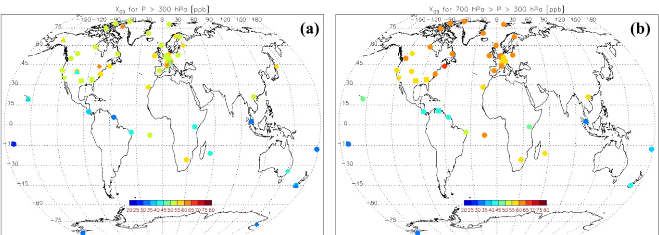
Figure 4: Mean (a) TrOC (ppb, surface to 300 hPa), (b) FTOC (ppb, 700 hPa to 300 hPa) at HEGIFTOM sites with at least 120 monthly values in the 2000-2022 period. Circles denote ozonesondes, squares = IAGOS airports, diamonds=FTIR, upward triangles=Umkehr, downward triangles=lidar. In the supplement, a Zoom over Europe of this figure is provided (Fig. S2), as well as the mean TrOC and FTOC distributions for DJF and JJA (Fig. S3).
