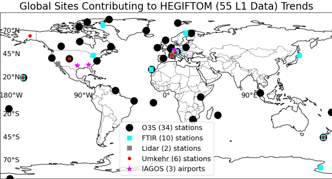
Figure 1: Partial map of sites for which ozone data have been homogenized and TrOC are available at the HEGIFTOM archive: https://hegiftom.meteo.be/datasets/tropospheric-ozone-columns-trocs . Five types of instruments are archived, color-coded as in key. Details on instrumentation, sample characteristics and locations appear in Table 1. Colors are superimposed at sites with data from more than one instrument (Table 1). Map shows 55 sites for which trends are computed according to the criteria (1) all datasets must start within 2000-2002 and end within 2019-2022 (see TOAR-II statistical guidelines, Chang et al., 2023), and (2) more than 120 monthly mean values.
