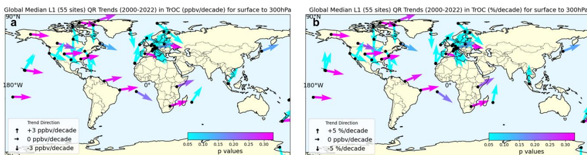
625 Figure 10: Geographical distribution of TrOC trends. (a) Trends for TrOC (in ppbv O 3 /dec) over period 2000-2022 based on QR analyses with HEGIFTOM L1 data. Arrows give magnitude of median 50%-ile trend value; note maximum limits are within \pm 3 ppbv. Confidence level indicated with p-value denoted by color scale, where p < 0.05 is considered high certainty and p > 0.3 very low certainty. For multiple arrows at sites with more than one instrument, refer to Table 1 for instrument key. (b) same as (a) except trends in %/dec and maximum range is within \pm 5 %/dec.
