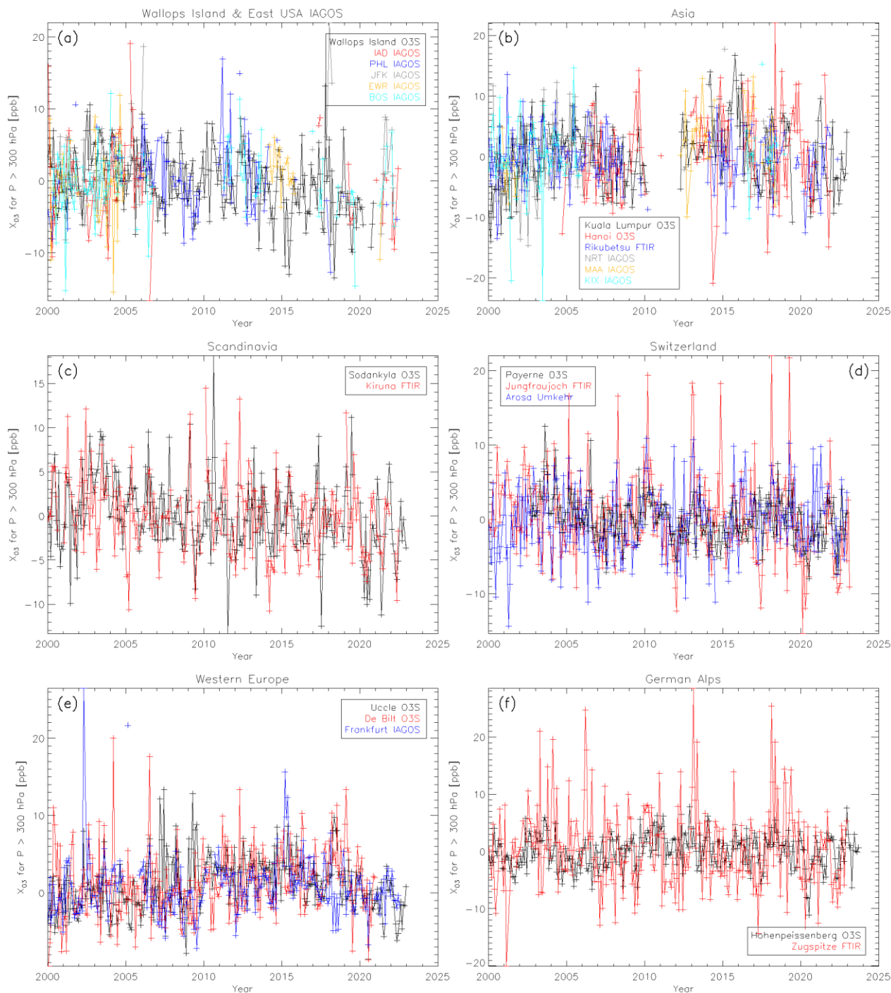
Figure 15: -Time-series for TrOC monthly anomalies, 2000-2022, for regional and nearby instrument clusters illustrated in Fig. 3. (a) eastern US, (b) Japan and southeast Asian sites and airports, (c) two nearby Scandinavian monitoring stations (d) 3 nearby Swiss stations, (e) 3 nearby western Europe ozonesonde stations and airport, (f) 2 nearby alpine German stations. For the eastern US and Asian sites, we do not present trend estimates. Monthly anomalies with time gaps more than 4 months are not connected with lines.
