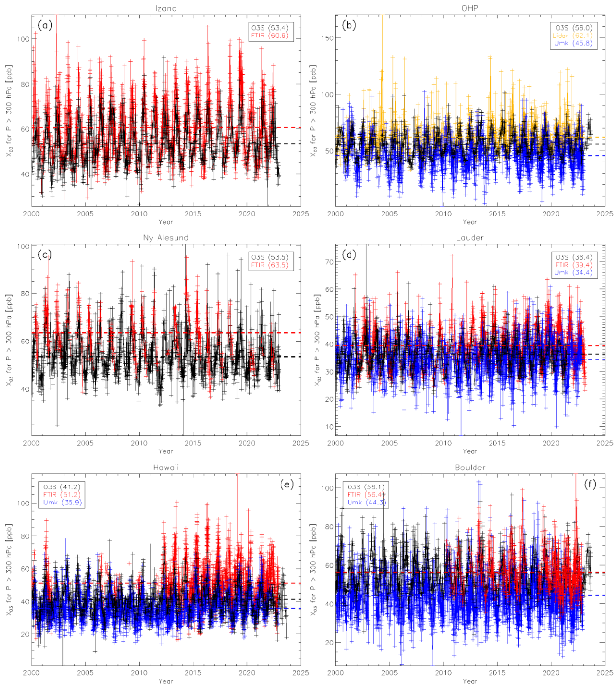
380 Figure 2: TrOC daily mean (L2) time series, 2000-2022, for collocated instruments as archived in the HEGIFTOM database. Dashed lines are the long-term mean values over 23-yr period. (a) Izaña, (b) OHP, (c) Ny Ålesund, (d) Lauder, (e) Mauna Loa and Hilo, Hawaii, (f) Boulder. Note that the FTIR time series in Boulder and Ny Ålesund do not fulfil our criteria used for trend detection here. Measurements with time gaps more than 4 months are not connected with lines.
