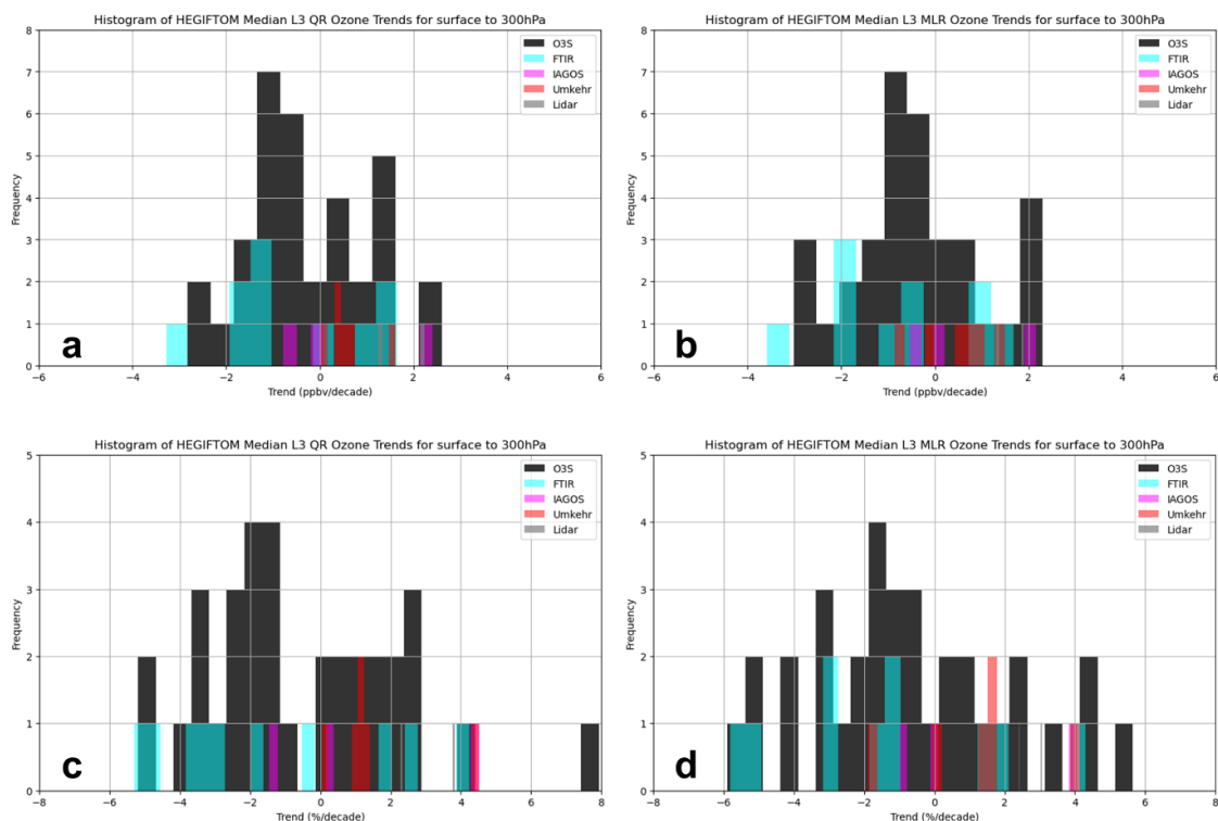
620 Figure 9: Histogram of median TrOC trends for 2000-2022 determined for 55 HEGIFTOM L3 data with color coding for each instrument type. (a) computed with QR analyses in ppbv/dec and %/dec in (c); (b) same as (a) for MLR analyses and (d) same as (c) for MLR analyses.
