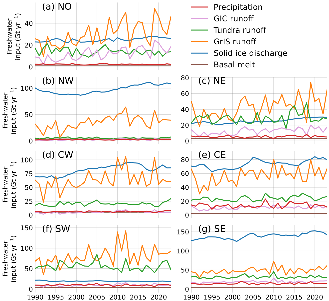
Figure 4. Time series of annual freshwater input per region between 1990-2023. Data sets used are indicated in bold in Table 1.
