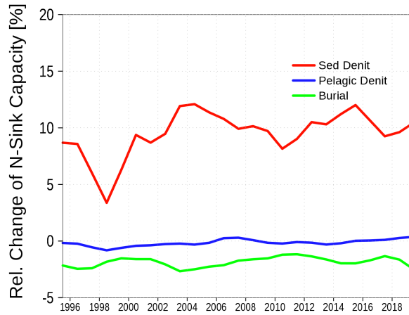
Figure 7. Change in relative nitrogen retention capacity between control run and 50% load reduction run.
