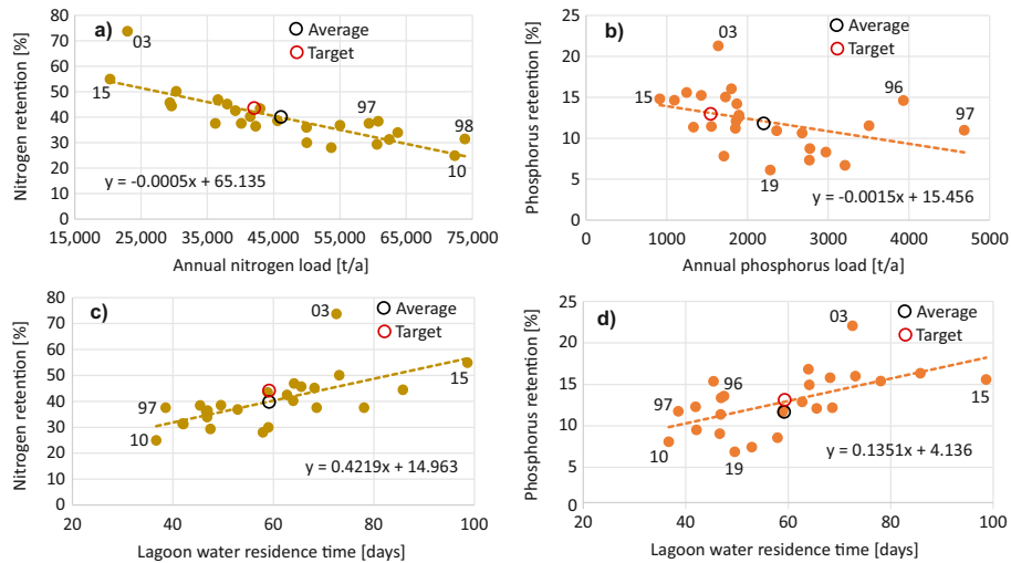
Figure 8. Relationship between annual riverine nitrogen and phosphorus loads and the nutrient retention in the Oder lagoon. c,d) Relationship between average annual water residence time and the nitrogen and phosphorus retention in the Oder lagoon. Residence time has been estimated following Vollenweider (1976); Monsen et al. (2002) by volume over runoff.
