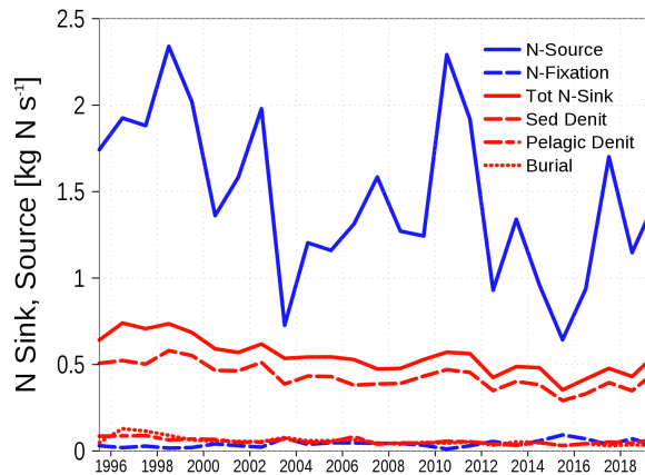
Figure 6. Nitrogen sources (blue) and sinks (red) in the Oder Lagoon. N-Sources are riverine loads and atmospheric deposition while N-Fixation is shown as a separate source (blue, dashed line). Tot N-Sink is the total sink of nitrogen; Red dashed and dotted lines are the contributing processes.
