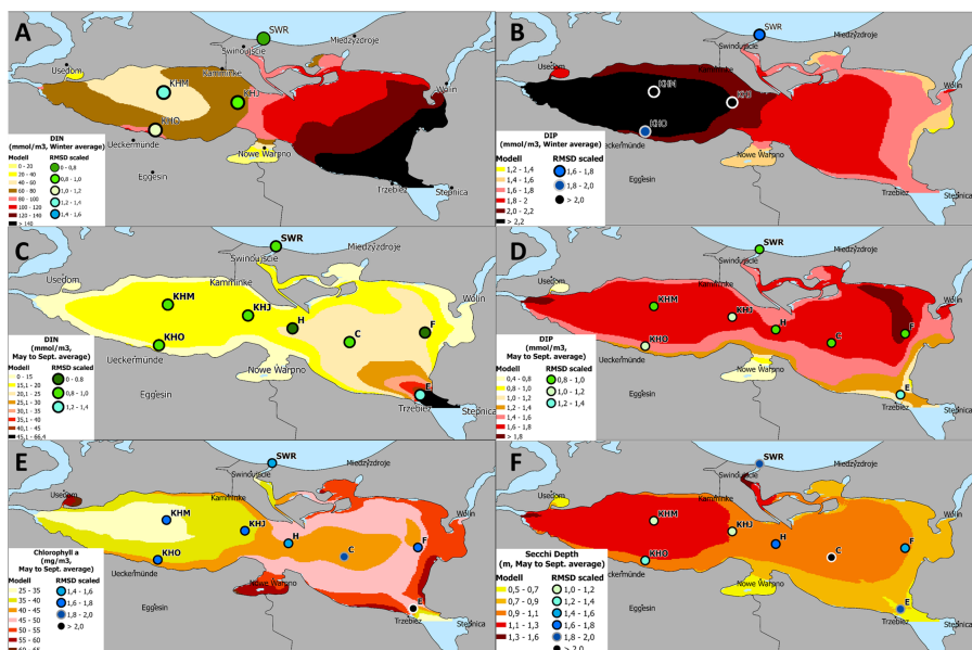
Figure A8. Near surface concentrations of dissolved inorganic nitrogen A: Winter average, C: May to September average; dissolved inorganic phosphorus B: Winter average, D: May to September average; Chlorophyll-a E: May to September average, and Secchi depth F: May to September average. All parameters are averaged from 2010 to 2019. The model results are color-coded and circles indicate the normalized RMSD for each monitoring station and parameter. The map was created using the software ESRI ArcGIS Pro (Version 3.3.2; https://pro.arcgis.com ).
