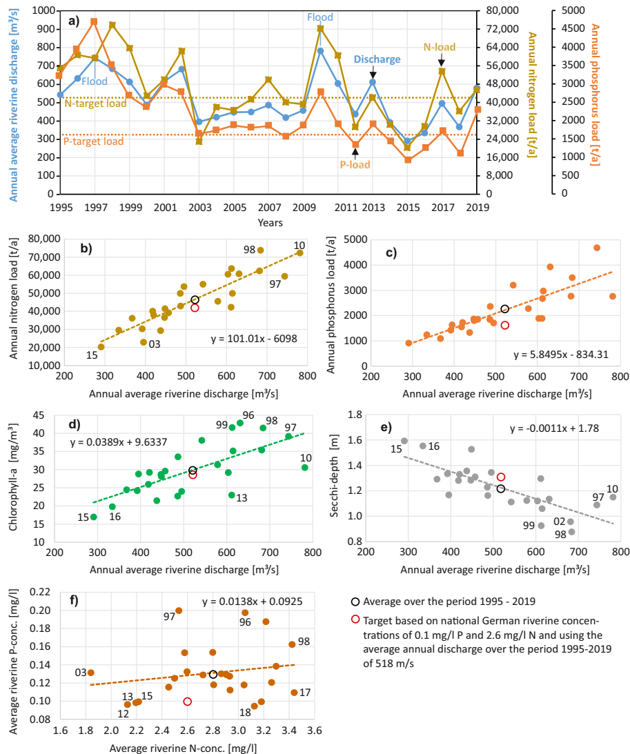
Figure 9. Average annual water discharge and annual loads of total nitrogen and total phosphorus to the Oder (Szczecin) Lagoon during a 25 years period (1995–2019), always including the rivers Oder/Odra, Uecker and Zarow. Relationship between riverine water discharge annual riverine nitrogen loads (b), annual riverine phosphorus loads (c), annual average phytoplankton biomass (chlorophyll-concentrations) (d) and annual average water transparency (Secchi depth) (e) in the Oder Lagoon (spatially integrated). (f) Relationship between riverine phosphorus and nitrogen concentrations.
