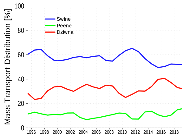
Figure A5. The relative contribution of the three outlet channels of the Oder Lagoon to the net water exchange with the Baltic Sea.
