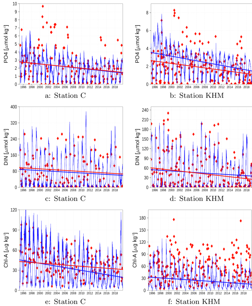
Figure A6. Surface concentration of phosphate, DIN, and chlorophyll at station C (a,c,e) and station KHM (b,d,f) (see Fig. 1). Red diamonds: Observations; Blue line: Model simulation. Straight lines show the trend if significant.
