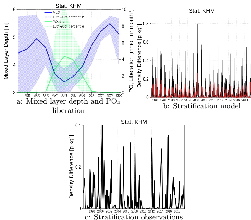
Figure A7. Climatology of model mixed layer depth and PO 4 liberation (a), stratification in model simulation (b), and in observations (c). Blue color in (a) are the mixed layer depth and green color the PO 4 liberation. The shaded area is the range between 10th and 90th percentile. The red line in (b) is from monthly mean and the black line from two-day mean model data. For (c), monthly mean observations are used. All data are from station KHM (see Fig. 1).
