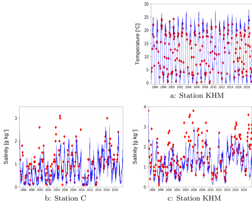
Figure A4. Surface temperature and salinity at station KHM (a,c) and salinity at station C (b) (see Fig. 1). Red diamonds: Observations; Blue line: Model simulation.
