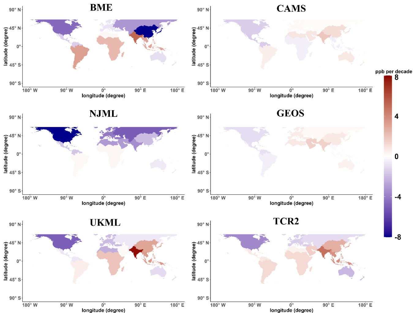
Figure 6: Population weighted ozone (OSDMA8) trends per decade for six datasets, calculated over the 2006-2016 period analyzed for each dataset. The different regions are defined in Table S7. Population weighted yearly trend of six datasets over priority regions (NAM, EUR, SAS, EAS, SEA, SAF, MDE) from 2006 to 2016 with 95% confidence intervals and p-values is shown in Table S9.
