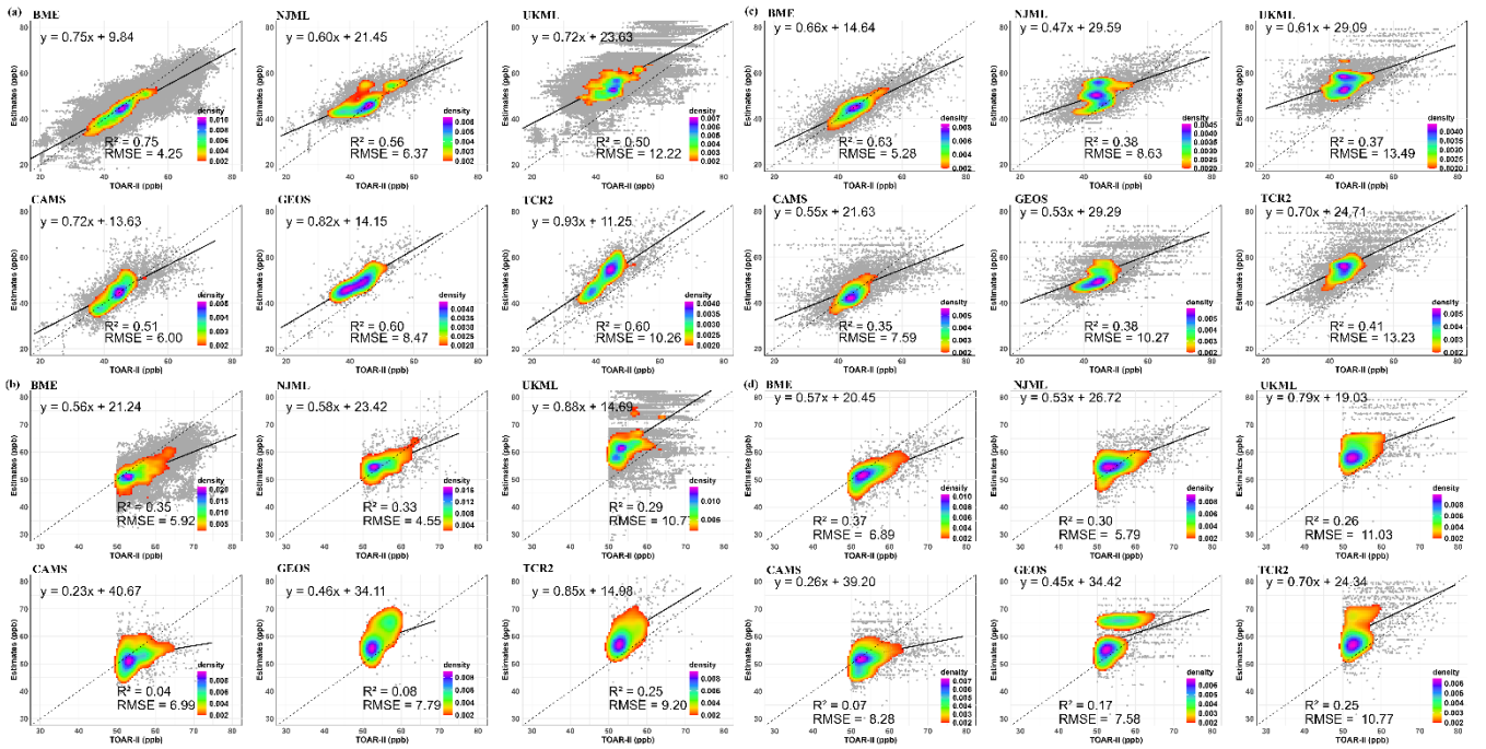
Figure 1: Performance evaluations of six datasets with TOAR-II observations in 2016 for OSDMA8. The observation-prediction evaluations are presented with densities estimated by a Gaussian kernel function. The coefficient of determination ( R^2 ) and root mean squared error (RMSE) are shown for four scenarios: (a) A grid-to-grid evaluation at the native resolution of each dataset using re-gridded TOAR-II observations, (b) A grid-to-grid evaluation, same as (a), but only for grid cells with observations above 50 ppb, (c) A grid-to-point evaluation using all TOAR-II sites, (d) A grid-to-point evaluation, same as (c), but only for sites with observations above 50 ppb. The dashed line marks where TOAR-II observations equal estimates ( y=x line), and the solid black line represents the best-fit line. Performance evaluations for each year are shown in Fig. S7 and Fig. S8.
