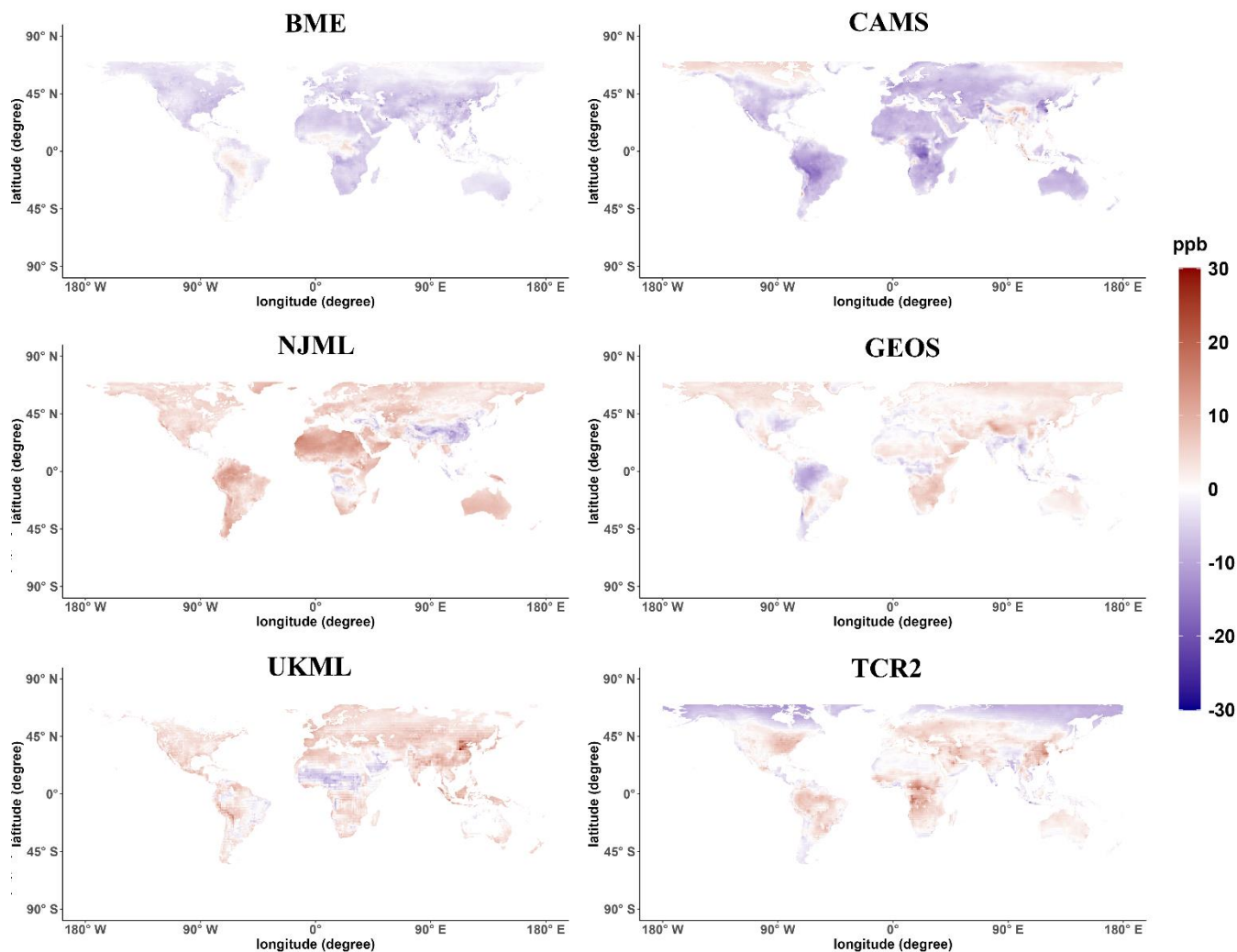
685 Figure 8: The difference of OSDMA8 in each grid cell between the 11-year (2006-2016) mean of each of six datasets and the ensemble mean (Fig. 3). Positive values indicate that the average estimate of the dataset is higher than the ensemble mean. Negative values indicate that the average estimate of the dataset is lower than the ensemble mean of the six datasets. Difference maps for each year are shown in Fig. S7.
