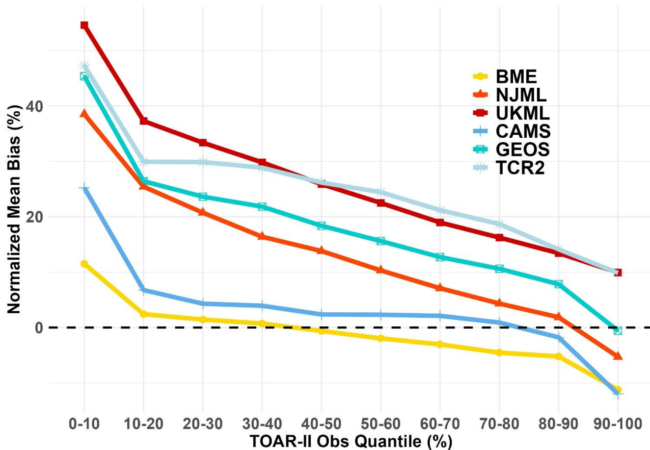
Figure 2: Normalized mean bias of six databases against TOAR-II observations (OSDMA8) at different quantiles in 2016, calculated based on the grid-to-point scenario. 0%: 13.46 ppb; 10%: 36.75 ppb; 20%: 39.80 ppb; 30%: 41.89 ppb; 40%: 43.57 ppb; 50%: 45.06 ppb; 60%: 46.82 ppb; 70%: 48.93 ppb; 80%: 52.18 ppb; 90%: 57.21 ppb; 100%: 86.25 ppb. Normalized mean bias for each year against TOAR-II observations are shown in Fig. S5. Different quantiles of TOAR-II observations for other years are shown in Table S11.
