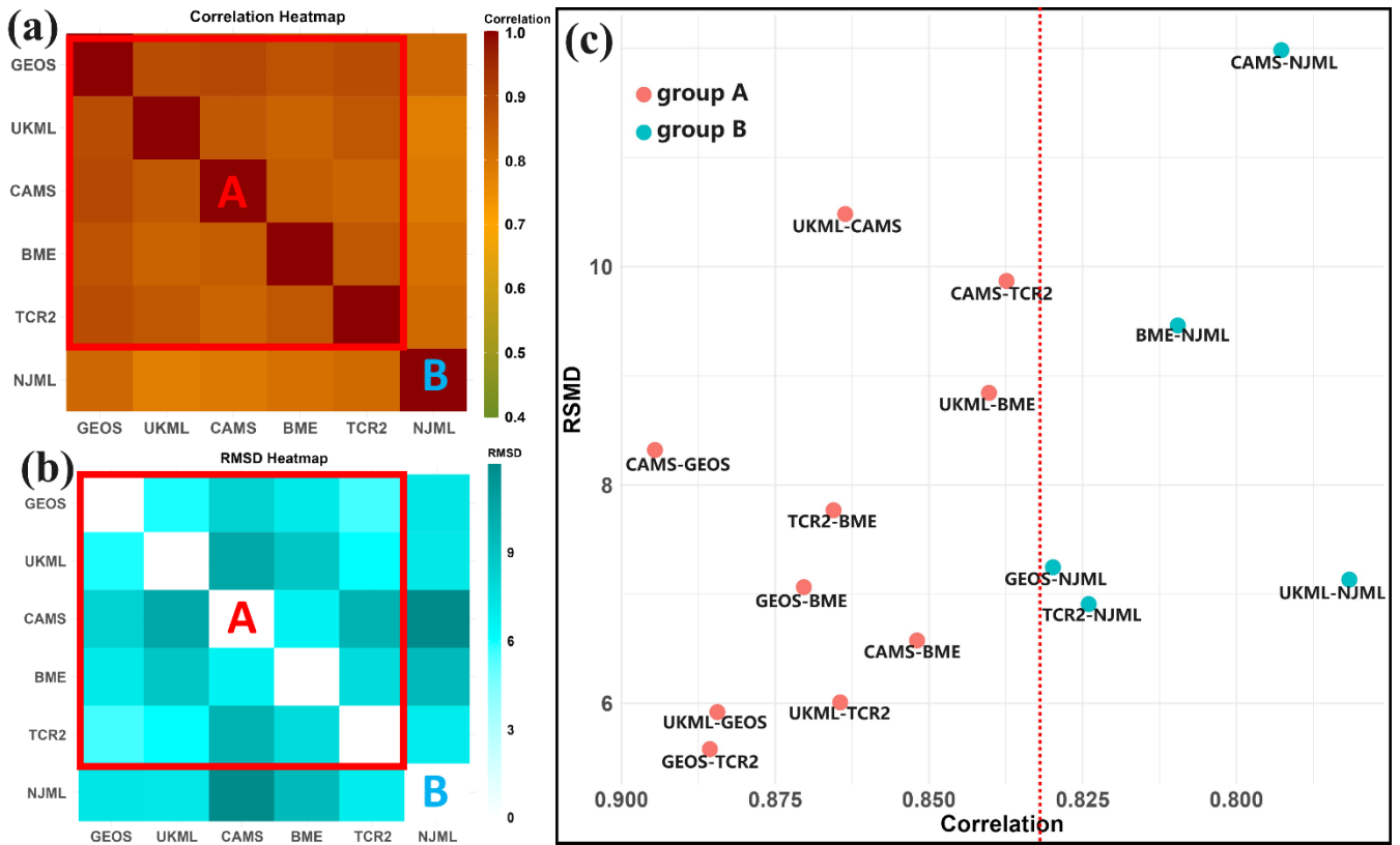
690 Figure 9: Heatmaps of similarity among the six datasets, including (a) heatmaps of average of pairwise correlation (Pearson R) between each dataset from 2006 to 2016. (b) heatmaps of average of pairwise Root mean square difference (RMSD) between each dataset from 2006 to 2016. Group A designates five datasets with strong similarity, while Group B is composed of one dataset with lower similarity with the rest. (c) Scatterplot of correlation and RMSD between each pair of datasets. The datasets with greatest similarity are in the lower left of panel c, and comparisons with the Group B dataset have lower correlation.
