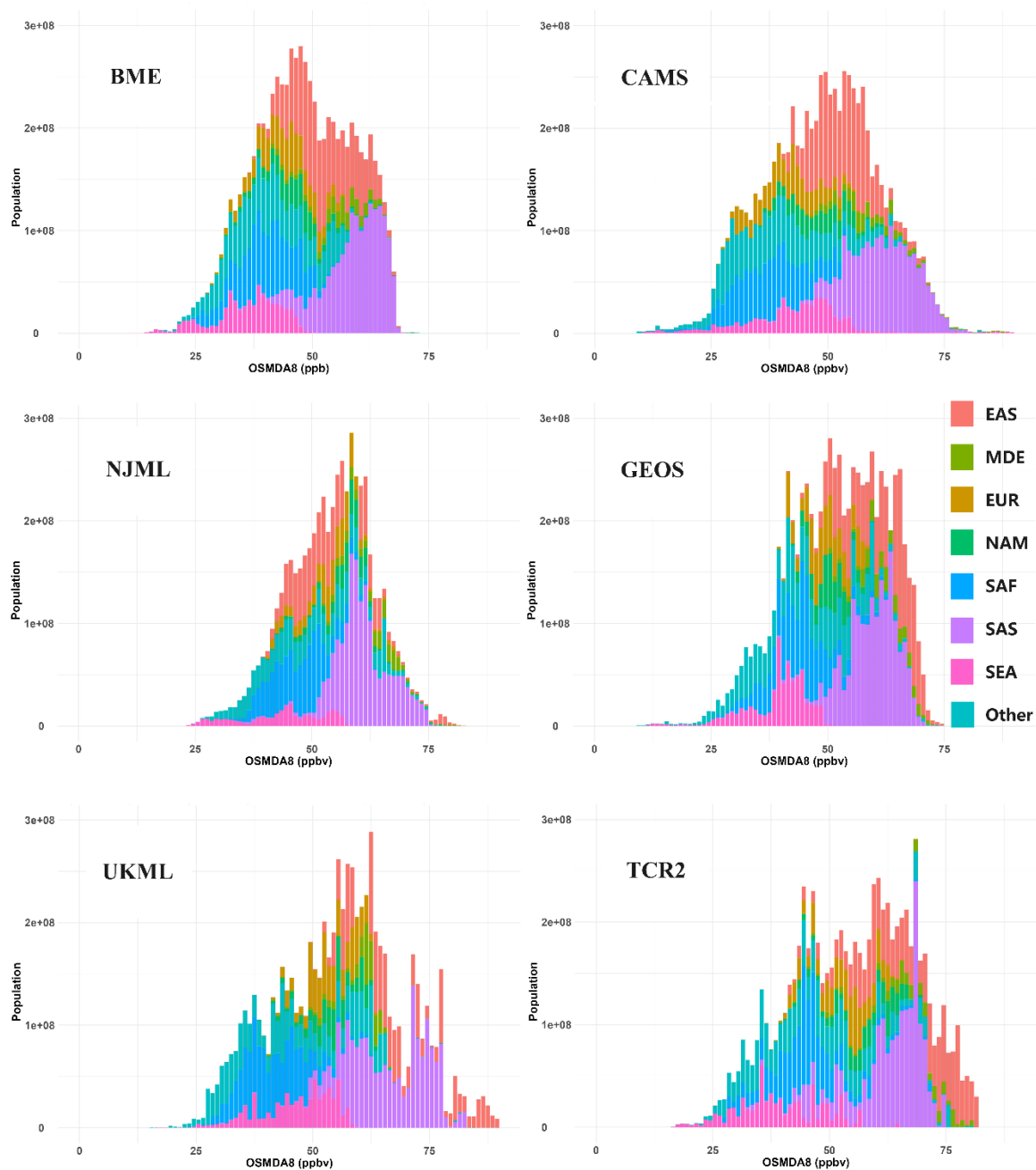
Figure 10: Population exposed to 11-year average ozone (OSMDA8) from 2006 to 2016 in different regions. The horizontal axis represents ozone concentrations, and the vertical axis represents population size. The definitions of different regions are included in Table S7. The Lower and Upper Bound of population exposure, which represent the 95% prediction interval for the estimate, are presented in Figure S12.
