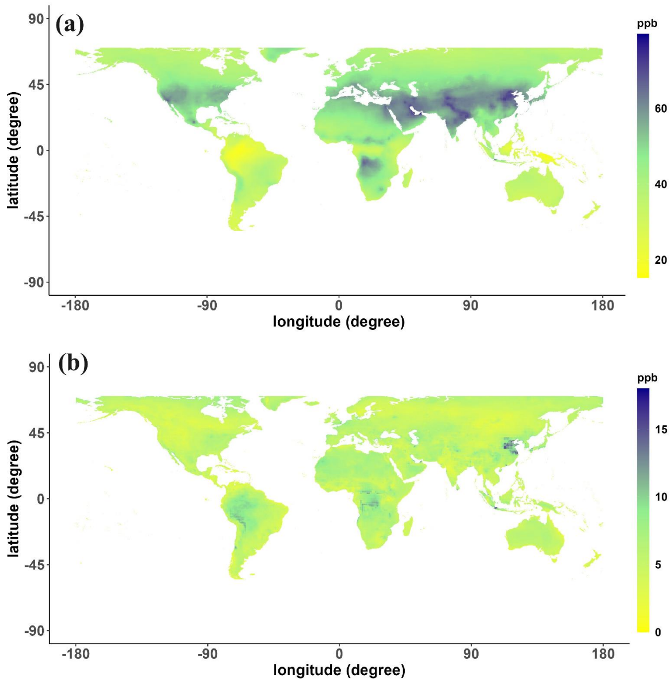
Figure 7: For six datasets from 2006 to 2016, (a) the 11-year ensemble mean, and (b) the average of annual standard deviations. Ozone data are reported as OSDMA8. The mean and standard deviation for each year are shown in Figures S5 and S6.
