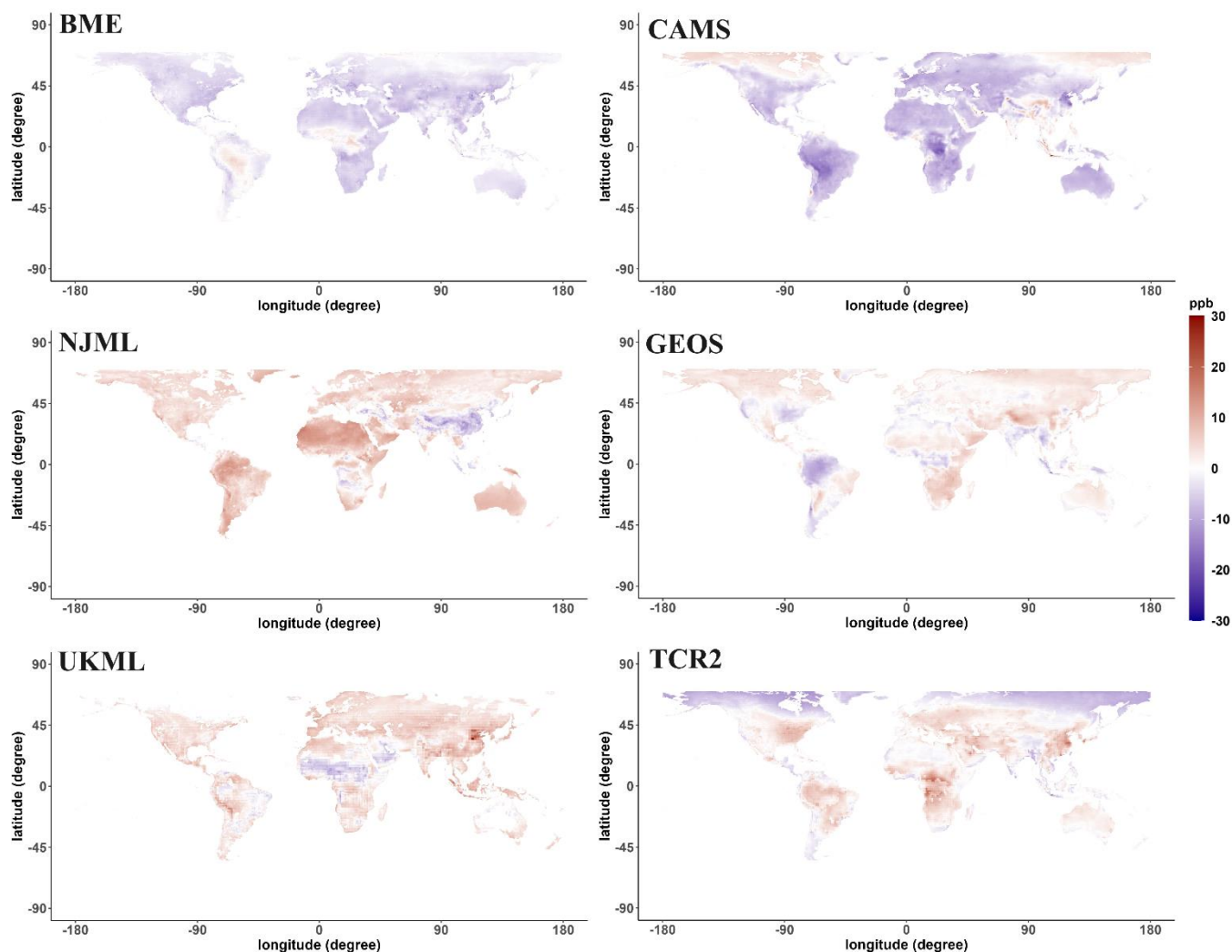
685 Figure 8: The difference of OSDMA8 in each grid cell between the 11-year (2006-2016) mean of each of six datasets and the ensemble mean (Figure 3). Positive values indicate that the average estimate of the dataset is higher than the ensemble mean. Negative values indicate that the average estimate of the dataset is lower than the ensemble mean of the six datasets. Difference maps for each year are shown in Fig. S7.
