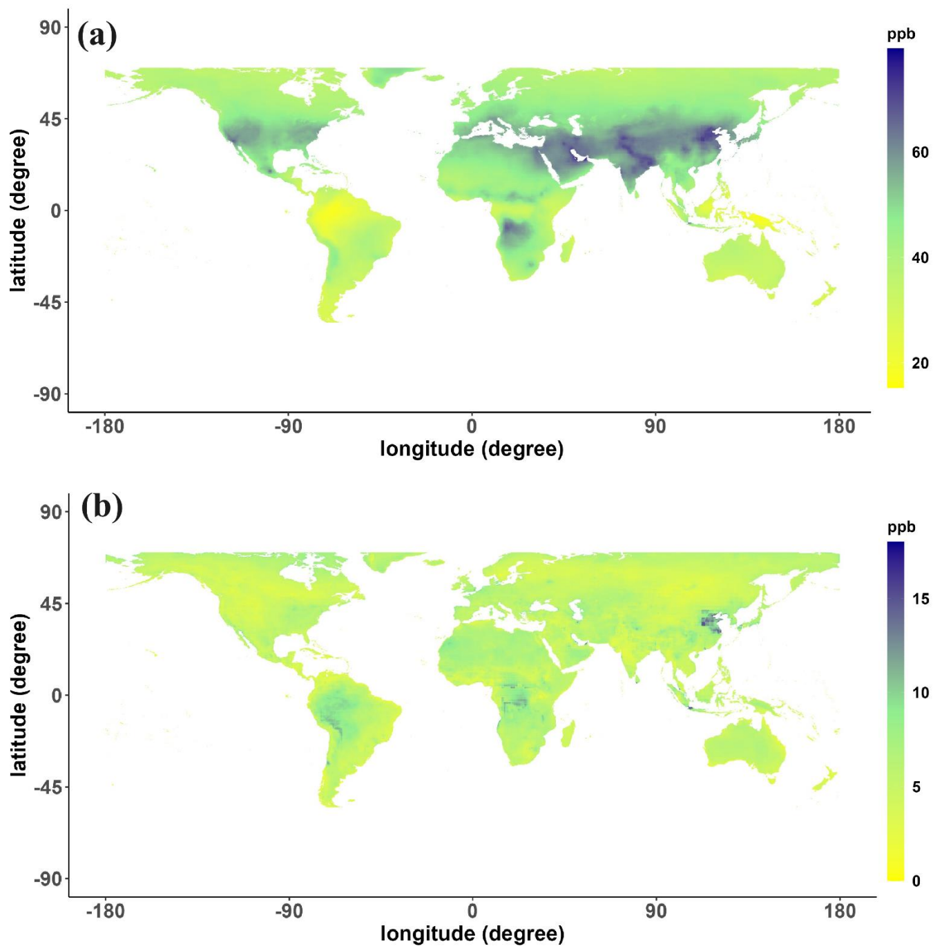
610 Figure 3: For six datasets from 2006 to 2016, (a) the 11-year ensemble mean, and (b) the average of annual standard deviations. Ozone data are reported as OSMDA8 OSDMA8 . The mean and standard deviation for each year are shown in Figures S5 and S6.
