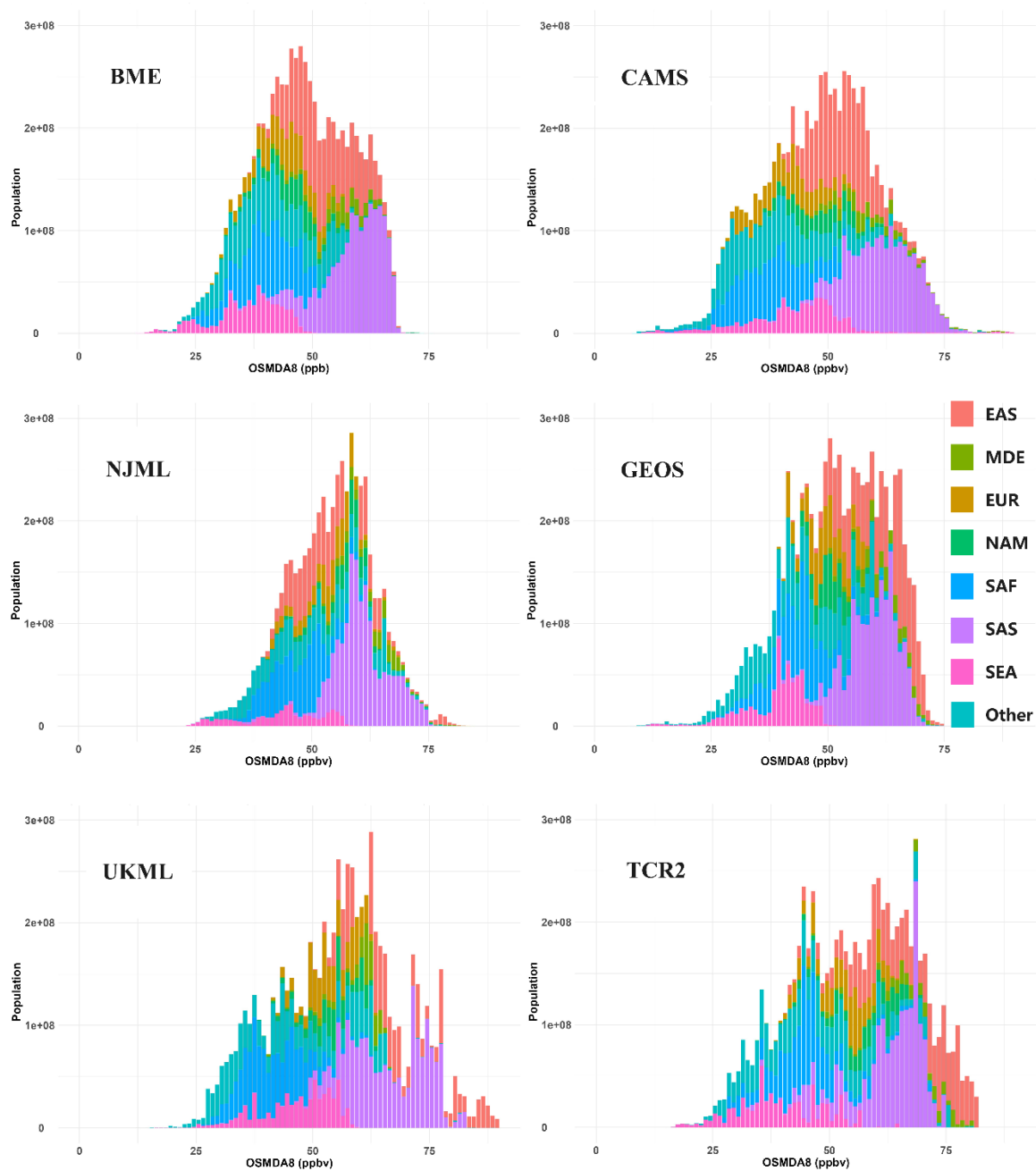
625 Figure 6: Population exposed to 11-year average ozone (OSMDA8OSMDA8) from 2006 to 2016 in different regions. The horizontal axis represents ozone concentrations, and the vertical axis represents population size. Concentrations and population for each year are presented in Figure S10. The definitions of different regions are included in Table S7.
