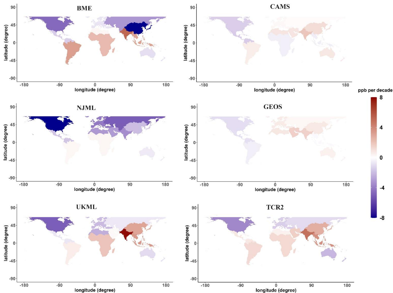
Figure 2: Population weighted ozone ( OSMDA8 OSDMA8) trends per decade for six datasets, calculated over the full 2006-2016 period analyzed for each dataset. The different regions are defined in Table S7. Population weighted yearly trend of six datasets over priority regions (NAM, EUR, SAS, EAS, SEA, SAF, MDE) from 2006 to 2016 with 95% confidence intervals and p-values is shown in Table S11. Population weighted ozone ( OSMDA8 OSDMA8) trends per decade for six datasets from 2006 to 2016 over the full period is shown in Figure S4.
