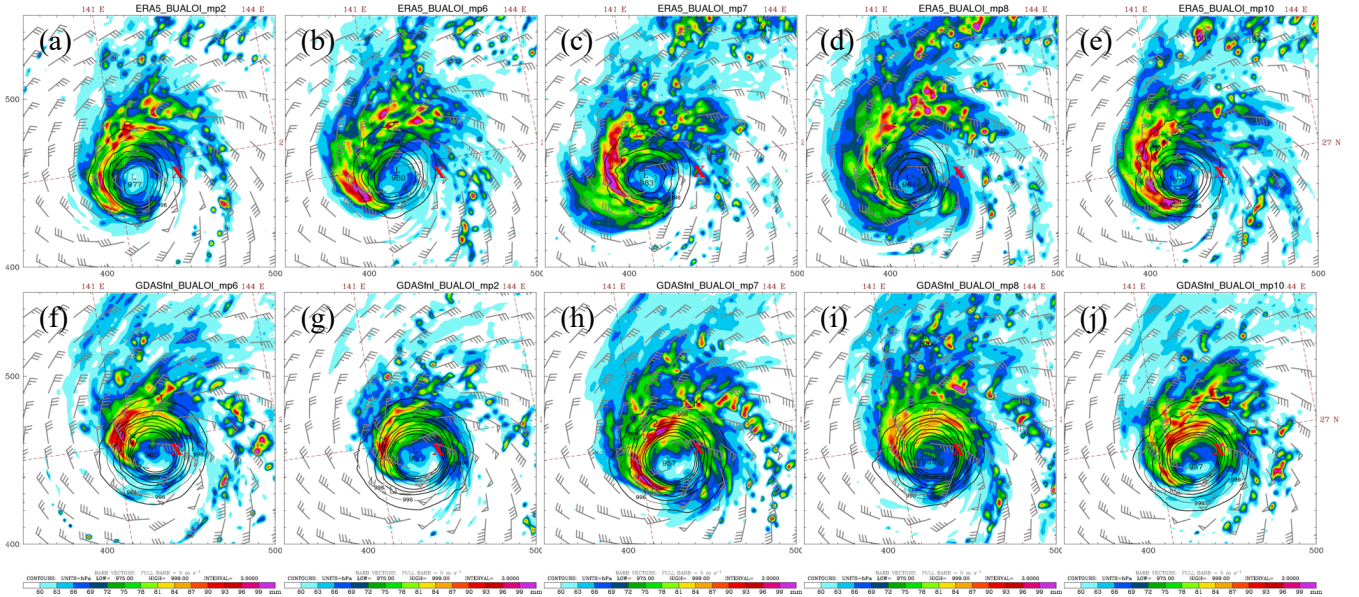
Figure 3. Panels (a)–(e) are similar to Figure 2a for total precipitable water (in color), sea level pressure (in contour), and wind vectors with the initial condition from ERA5, but for WRF 18-hour forecast with different microphysics schemes: (a) Purdue Lin scheme, (b) WSM 6-class graupel scheme, (c) Goddard 4-ice scheme, (d) Thompson graupel scheme, and (e) Morrison 2-moment scheme. Panels (f)–(j) are the same as (a)–(e), but for the initial conditions from NCEP FNL. The red cross sign in each panel, at 26.8°N and 142.1°E indicates the observed location of Typhoon Bualoi from the JTWC's best track.
