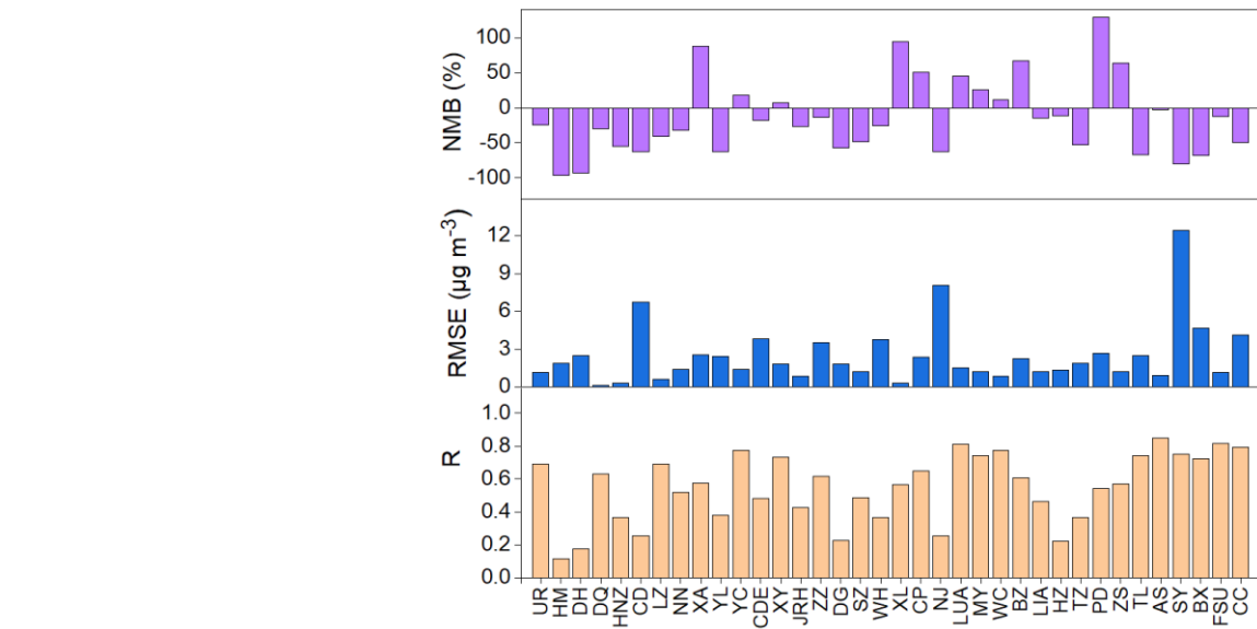
245 Figure 2. Comparisons of simulated versus observed daily mean BC concentrations at each site.
