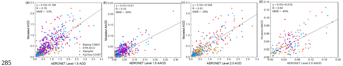
Figure 5. Comparison of simulated mean daily AOD (a, c) and AAOD (b, d) at 440nm with AERONET Level 1.5 (a, b) and 2.0 (c, d). Colored circles are the AERONET sites.
