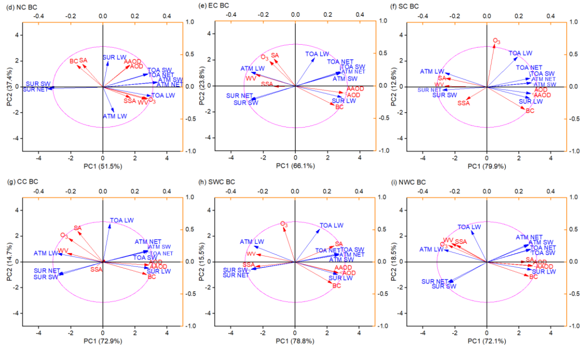
Figure 8. Principal component analysis biplots for BC DRFs and the influencing factors over seven regions in China (a), entire China (b), Northeast China (NEC, c), North China (NC, d), East China (EC, e), South China (SC, f), Central China (CC, g), Southwest China (SWC, h), and Northwest China (NWC, i). Blue and red arrows represent BC DRFs and their influencing factors, respectively. SA and WV are surface albedo and water vapor, respectively.
