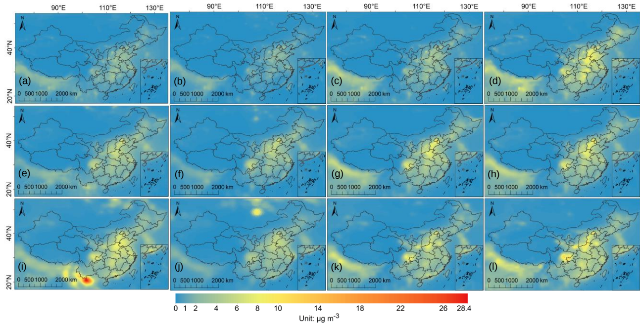
250 Figure 3. Spatial distribution of BC concentrations over China. Seasonal BC concentrations obtained from the GEOS-Chem simulation (a-d), MERRA-2 (e-h), and CAMS (i-l) in spring (a, e, and i), summer (b, f, and j), fall (c, g, k) and winter (d, h, l).
