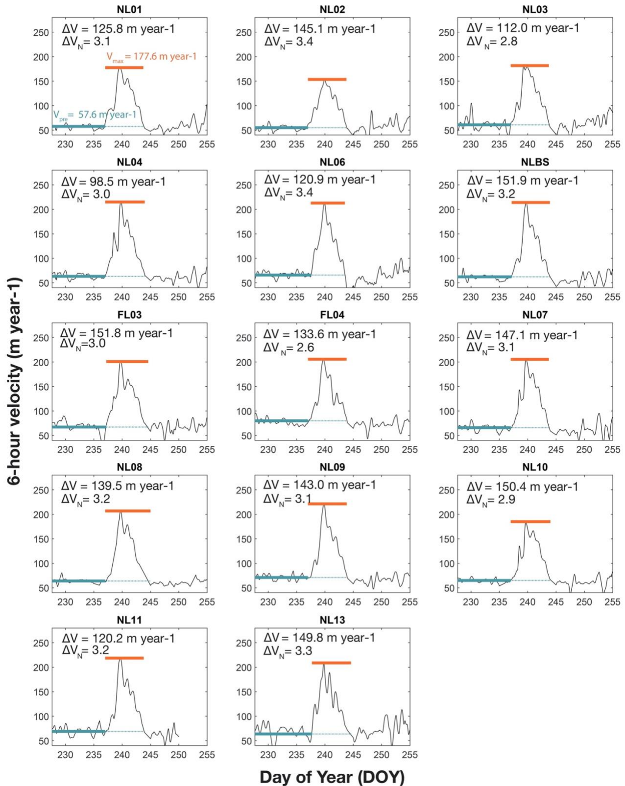
755 Figure 4. Velocity time series at all stations for the 2011/238 late-season speed-up event. Green lines show the pre-event time period and average velocity ( V_{pre} ). Orange lines show the maximum velocity ( V_{max} ) throughout the event. Speed-up magnitudes of \Delta V ( V_{max} - V_{pre} ) and \Delta V_N ( V_{max}/V_{pre} ) are given in upper left corner of each panel.
