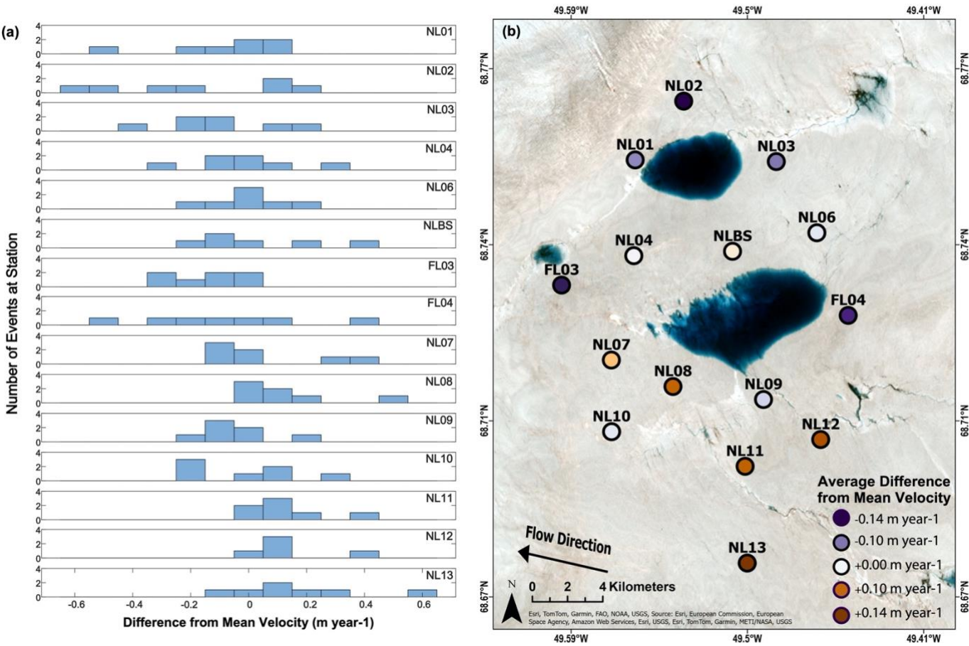
Figure 12. (a) Deviation of \Delta V (m/yr) from the array mean ( \overline{\Delta V}_{array} ) at each station for each of the 7 transient speed-up events in 2011. (b) Average speed-up at each GPS sensor location for all events. Circles represent individual station locations: red colors show greater than \overline{\Delta V}_{array} and blue colors show lesser than \overline{\Delta V}_{array} . Note the similarity in the spatial pattern of speed-up compared to the 2012/180 neighboring lake drainage event.
