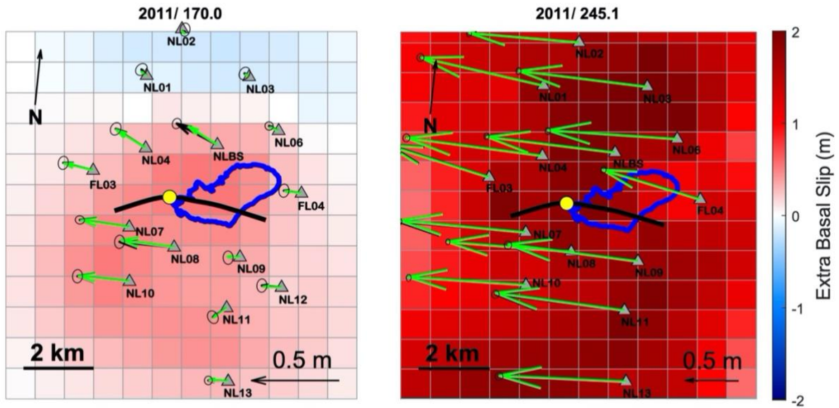
745 Figure 2. Maximum event basal slip for (a) 2011/169 lake drainage on DOY 170.0, and (b) 2011/238 on DOY 245.1. Moulin location is denoted with yellow dot, hydro-fracture crack is shown by thick black line, and North Lake basin is outlined in blue. GPS sensor locations are shown by black triangles with the black arrows representing the GPS displacement and green arrows show NIF displacement. Dark red colors (+) indicate greater basal slip than background and blue colors indicate (-) less than background values.
