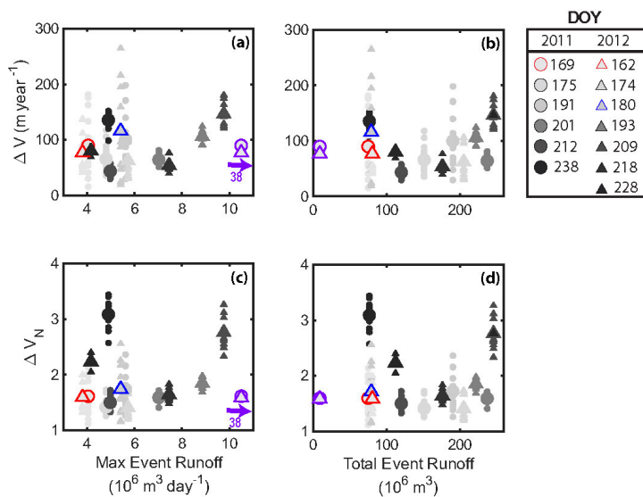
Figure 6. Velocity response \Delta V and \Delta V_N as a function of the maximum event runoff at the nearest RACMO grid cell (panels a,c), and total event runoff (panels b,d) integrated over the 6 local RACMO grid cells (Fig. S3a). Circles show events in 2011; triangles show events in 2012. Small symbols show \Delta V and \Delta V_N for each individual GPS station; larger symbols show \overline{\Delta V} and \overline{\Delta V_N} across all stations for each event. Colors darken chronologically with the lightest grey colors indicating events early in the melt season and the darkest black colors representing events late in the melt season. Note the lack of a trend in any of the panels. The red-outlined symbols highlight the lake drainage events. The blue-outlined symbols highlight the 2012/180 nearby lake drainage event. The purple-outlined symbols show \Delta V and \Delta V_N for the lake drainage events using “effective runoff.” In panels (a,c), the maximum “effective runoff” significantly exceeded the maximum runoff from RACMO (effective runoff value annotated); however the total lake volume is small compared to the integrated event runoff (b,d).
