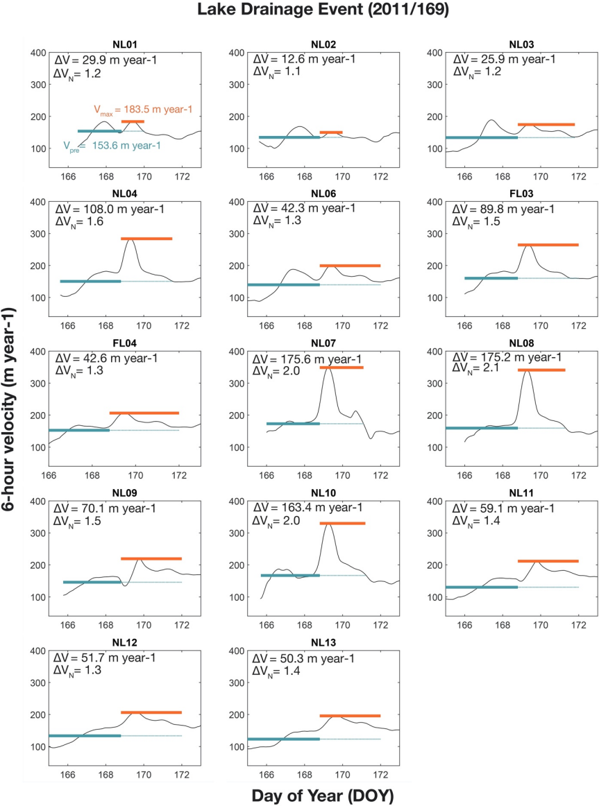
Figure 5. Velocity time series at all stations for the 2011/169 lake drainage event. Green lines show the pre-event time period and average velocity ( V_{pre} ). Orange lines show the maximum velocity ( V_{max} ) throughout the event. Speed-up magnitudes of \Delta V ( V_{max} - V_{pre} ) and \Delta V_N ( V_{max}/V_{pre} ) are given in the upper left corner of each panel.
