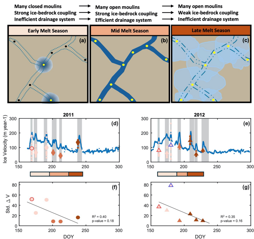
920 Figure 9. Conceptual model for subglacial conditions and ice response to melt input during (a) early-season lake drainage events, (b) mid melt season, and (c) late melt season. Yellow solid circles represent open moulins and black solid circles represent closed moulins. Lighter blue colors indicate lesser volumes of meltwater at the bed (a, c). Dark blue colors indicate greater volumes of meltwater at the bed (a–b). The circles and triangles show the \Delta V (m/yr) of each speed-up in (d) 2011 and (e) 2012, respectively. Individual symbols in panels (c) and (d) represent GPS sensors, and the larger symbols are the array-average for each speed-up event. The red-outlined symbols are lake drainages and the blue-outlined symbol is a local lake drainage. The blue line shows the 24-hour average velocity across the GPS array. Light red colors indicate early-season events, medium red colors indicate middle season melt events, and dark red colors indicate late-season melt events (d–g). The circles and triangles show the average standard deviation of \Delta V of each speed-up event in (f) 2011 and (g) 2012, respectively. 925
