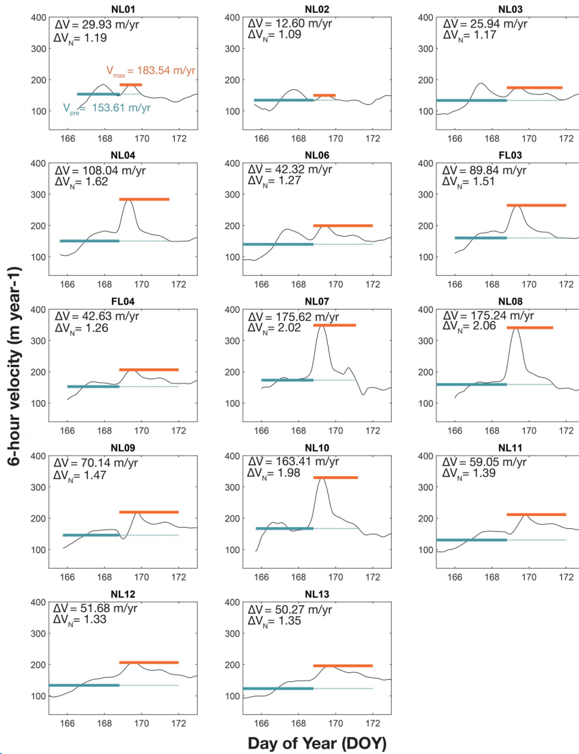
Figure 5. Velocity time series at all stations for the 2011/169 lake drainage event. Green lines show the pre-event time period and average velocity ( V_{\text{pre}} ). Orange lines show the maximum velocity ( V_{\text{max}} ) throughout the event. Speed-up magnitudes of \Delta V ( V_{\text{max}} - V_{\text{pre}} ) and \Delta V_N ( V_{\text{max}}/V_{\text{pre}} ) are given in the upper left corner of each panel.
