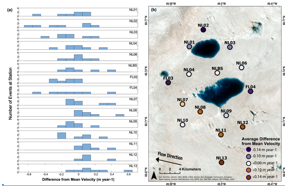
Figure 12. (a) Deviation of \Delta V (m/yr) from the array mean ( \Delta V_{array} ) at each station for each of the 7 transient speed-up events in 2011. (b) Average speed-up at each GPS sensor location for all events. Circles represent individual station locations: red colors show greater than \Delta V_{array} and blue colors show lesser than \Delta V_{array} . Note the similarity in the spatial pattern of speed-up compared to the 2012/180 neighboring lake drainage event.
