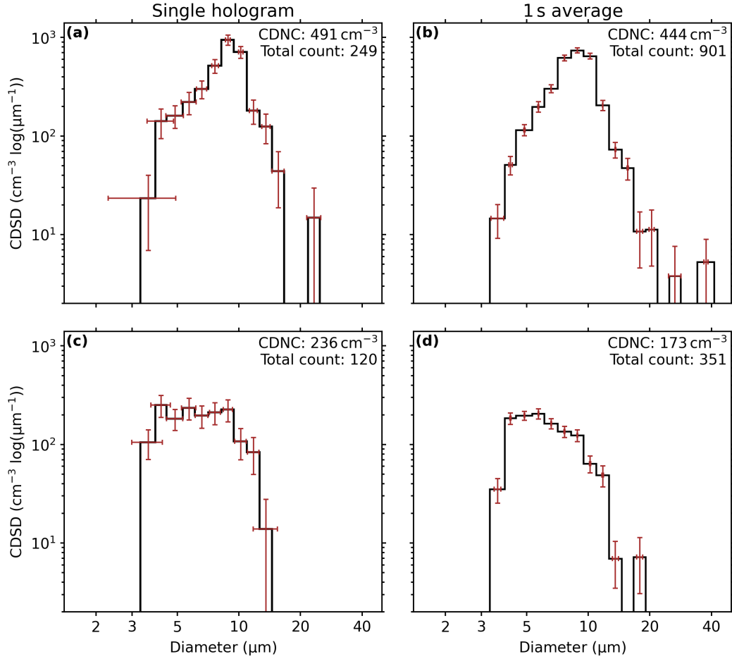
Figure C1. Exemplary cloud droplet size distributions (CDSs) measured with SmHOLIMO in black with associated diameter and counting uncertainties (red error bars). (a) and (c) show CDSs retrieved from single holograms recorded at 08:09:59.736 UTC and 08:39:59.955 UTC, respectively. (b) and (d) show CDSs averaged over 1-second intervals, recorded between 08:09:59 - 08:10:00 UTC and 08:39:59 - 08:40:00 UTC, respectively. Diameter uncertainties are calculated as \Delta d = d_s \cdot \sqrt{N}^{-1} with d_s = 1.85 \mu\text{m} the error of a single droplet measurement of pixel pitch and N being the number of droplets in each size bin. Counting uncertainties are derived from counting statistics as \sqrt{N} . The CDNC and respective total number of droplets are indicated in the upper right corner of each panel.
