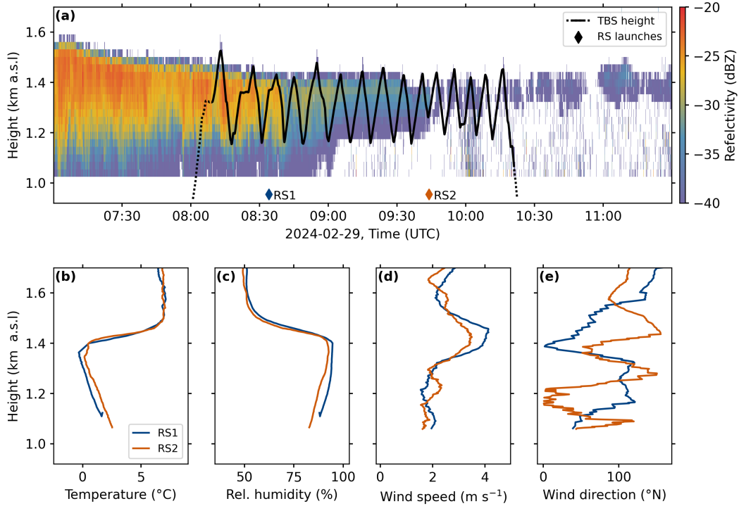
Figure 4. Meteorological conditions during the cloud measurements on 29 February 2024. (a): A height-time-indicator (HTI) reflectivity measurements in dBZ of a vertically pointing W-band Doppler cloud radar of a dissipating low stratus between 7:00 and 11:30 UTC. The time and height of the 30 vertical profiles (dotted and solid black line) of the tethered balloon system (TBS) are shown. The dotted black sections indicate times when no in situ measurements were taken. The launch times of two radiosondes (RS1, 08:34 UTC, blue diamond; RS2, 09:46 UTC, orange diamond) are shown at the bottom. The meteorological variables of RS1 (blue) and RS2 (orange) are shown as vertical profiles in (b) temperature, (c) relative humidity, (d) wind speed, and (e) wind direction.
