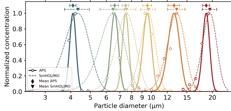
Figure 3. Normalized APS and SmHOLIMO size distributions with a brightness threshold of 0.5 for six size algorithm validation experiments with different droplet diameters (colors) ranging from of \approx 4 \mu\text{m} to \approx 19 \mu\text{m} . The APS means (diamond) and standard deviations (solid bars) are retrieved from Gaussian functions (solid lines) that are fitted to the APS measurements (circles). The SmHOLIMO means (triangles) and standard deviations (dotted bars) are retrieved directly from the distribution of the single particle data and the Gaussian functions (dashed lines) are derived from them.
