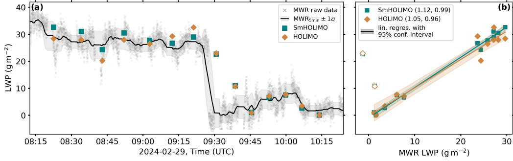
Figure 7. (a): Time series of the liquid water path (LWP) in \text{g m}^{-2} observed with the Microwave Radiometer (MWR, gray crosses, raw data points) with a 5 min moving average (solid black) and the respective standard deviation (gray shading) together with the LWP derived from ascending profiles for SmHOLIMO (blue squares) and HOLIMO (orange diamonds). (b): Correlation plot of SmHOLIMO (blue) and HOLIMO (orange) LWP versus MWR LWP. Also shown are linear regressions (solid lines) with respective slopes and Pearson r^2 values in parentheses (slope, r^2 ) and 95 % confidence intervals (shading). The unfilled data points obtained between 09:30 and 09:45 UTC were excluded from the linear regression due to a strong spatial inhomogeneity in the air mass.
