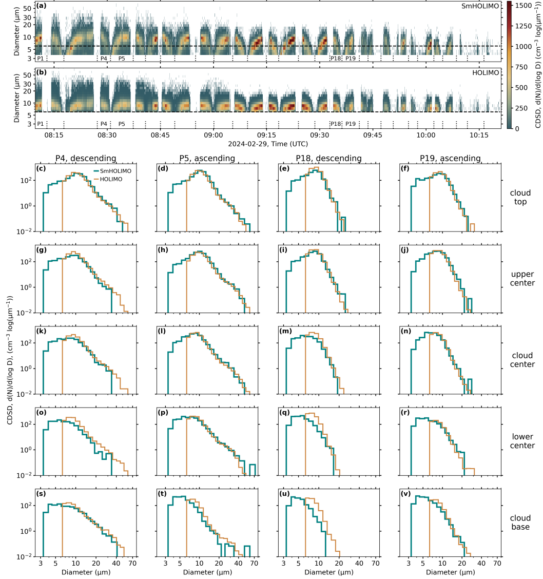
Figure 5. Cloud droplet size distributions (CDSs) measured with SmHOLIMO (a) and HOLIMO (b) over time during the 30 profiles. The black dotted vertical lines at the bottom indicate the start and end of each profile. Exemplary profile numbers are shown for profiles P1, P4, P5, P18, and P19, with odd numbers representing ascending profiles and even numbers representing descending profiles (see Table B1). The resolution limit of HOLIMO, of 6\ \mu\text{m} (dashed black line), is shown for easier comparison. Figures (c - v) show averaged CDSs for different cloud sections with cloud top in row 1 (c - f), upper center in row 2 (g - j), cloud center in row 3 (k - n), lower center in row 4 (o - r) and cloud base in row 5 (s - v). The cloud sections are determined for each profile individually by dividing the observed total cloud thickness (constrained by \text{LWC} > 0.01\text{g m}^{-3} ) into five equally sized parts. Shown are profiles P4, descending, column 1, (c - s); P5, ascending, column 2, (d - t); P18, descending, column 3, (e - u); and P19, ascending, column 4, (f - v).
