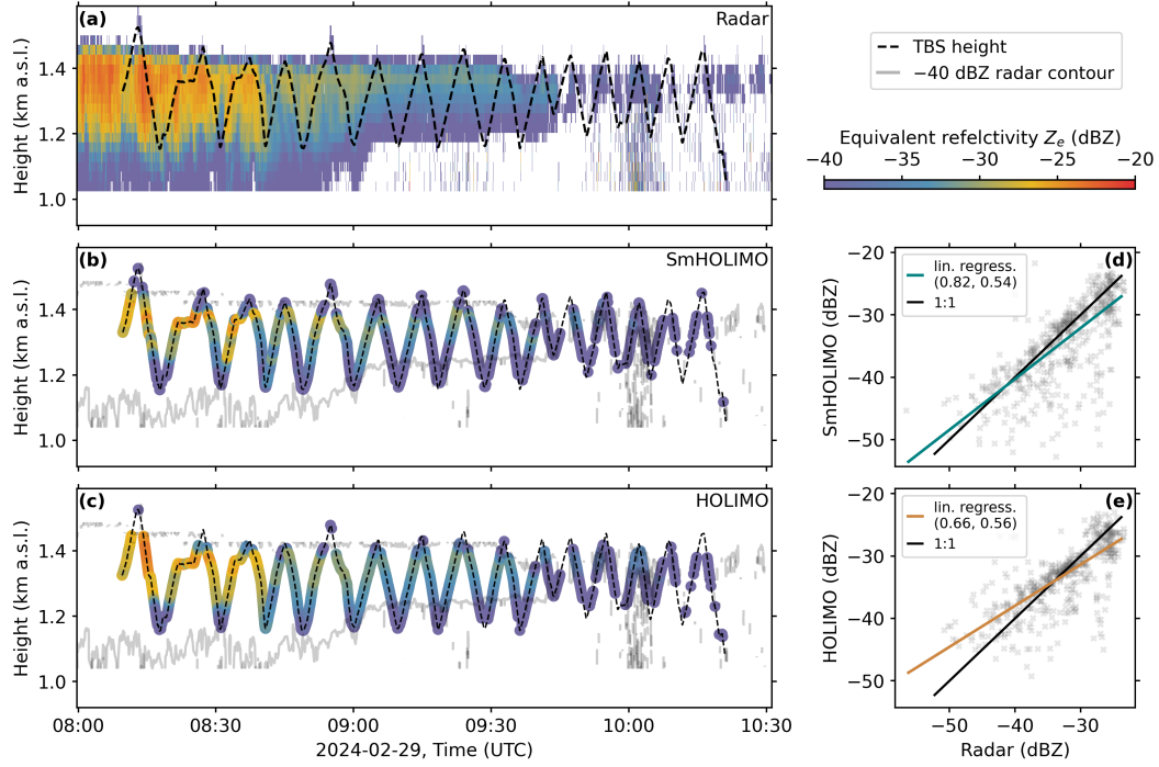
Figure 8. (a): Measured height-time-indicator (HTI) equivalent reflectivities Z_e in dBZ from a vertically pointing W-band Doppler cloud radar. Calculated Z_e in dBZ over the TBS flight track for SmHOLIMO in (b) and HOLIMO in (c) together with the -40 dBZ contour line (gray lines) from the radar Z_e measured in (a). Calculated reflectivities are shown only for values > -60 dBZ (lower limit of cloud radar). A moving average over 20 s is applied to the calculated Z_e in (b) and (c). Correlation plots of the calculated Z_e vs. the radar Z_e (gray crosses) are shown in (d) for SmHOLIMO and (e) for HOLIMO. Also shown are the one-to-one lines (solid black) and linear regressions (solid blue, (d), solid orange (e)) with slopes and Pearson r^2 values in parentheses (slope, r^2 ).
