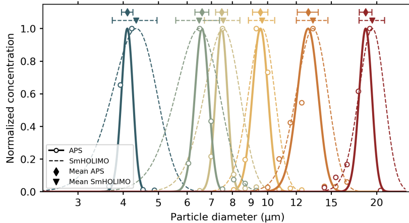
Figure 3. Normalized APS and SmHOLIMO size distributions with a brightness threshold of 0.5 for six size calibration algorithm validation experiments with different droplet diameters (colors) ranging from of \approx 4 \mu\text{m} to \approx 19 \mu\text{m} . The APS means (diamond) and standard deviations (solid bars) are retrieved from Gaussian functions (solid lines) that are fitted to the APS measurements (circles). The SmHOLIMO means (triangles) and standard deviations (dotted bars) are retrieved directly from the distribution of the single particle data and the Gaussian functions (dashed lines) are derived from them.
