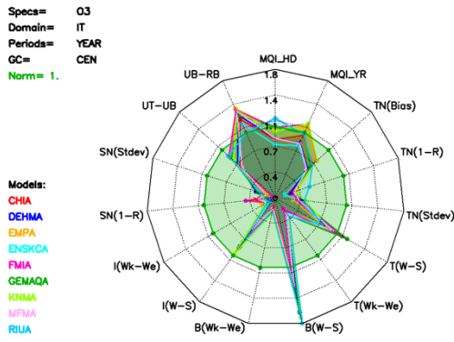
Figure 12. Radar plots of the calculated air quality model indicators for 8-hour maximum O 3 values for different countries: (a) Spain, (b) France, (c) Germany, (d) Poland and (e) Italy. Indicators are: MQI Hourly (MQI_HD), MQI Year (MQI_YR), Bias, 1-R (Time), Standard deviation (Time), gradients for Winter-Summer, Week-Weekend, Day-Night for Traffic, Industry, Background (T, I, B), 1-R Spatial, Standard Deviation spatial, Yearly Urban-Traffic vs Urban-Background (Year UT-UB), Yearly Urban-Background vs Rural-Background (Year UB-RB).
