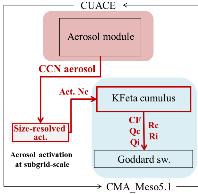
245 Figure 3: The diagram of subgrid-scale aerosol–cloud–radiation interaction in the CMA_Meso5.1/CUACE model.
