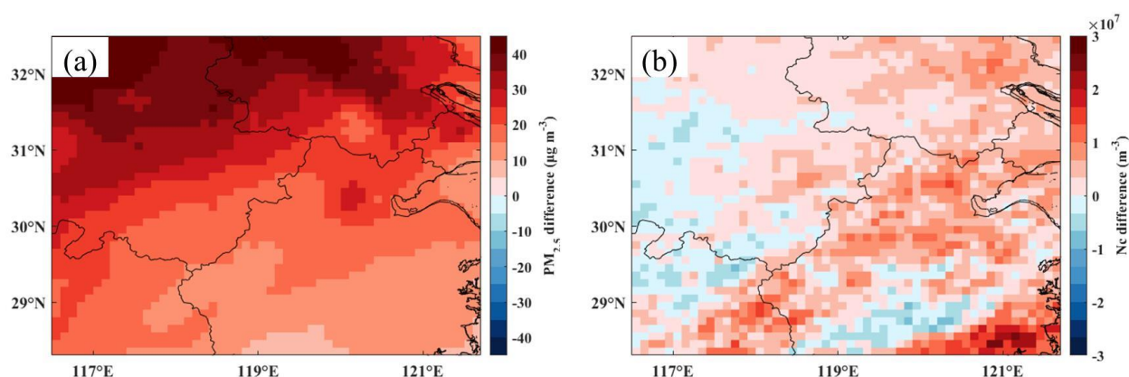
520 Figure 16: The spatial distribution of the difference between the ACI sub -DC and CACI sub -DC experiment for the time average (a) PM 2.5 mass concentration and (b) subgrid-scale cloud droplets number concentration (mean values in 1-6 km) from 26 to 29 June 2016.
