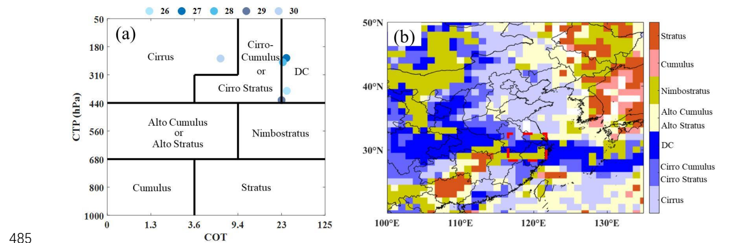
Figure 13: (a) Cloud types over YRD from 26 to 30 June 2016 based on the International Satellite Cloud Climatology Project (ISCCP) cloud classification algorithm (Hahn et al., 2001). (b) The spatial distribution of cloud types in central and eastern China on 28 June 2016. The red dashed rectangle is the location of the YRD region.
