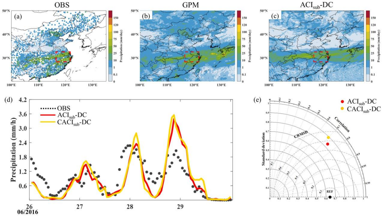
Figure 15: The spatial distribution of time average 24 hours cumulative precipitation from 26 to 29 June 2016 in the (a) observations, (b) GPM, and (c) ACI_{sub-DC} experiment. The (d) time variation and (e) Taylor diagram of observed and simulated regional average hourly precipitation in YRD from 26 to 29 June. In the Taylor diagram, the REF is the observation, the vertical coordinate is the standard deviation (STD), the distance between the simulations and REF is the centered root mean square deviation (CRMSD), and the position of the azimuth is the correlation coefficient ( R ).
