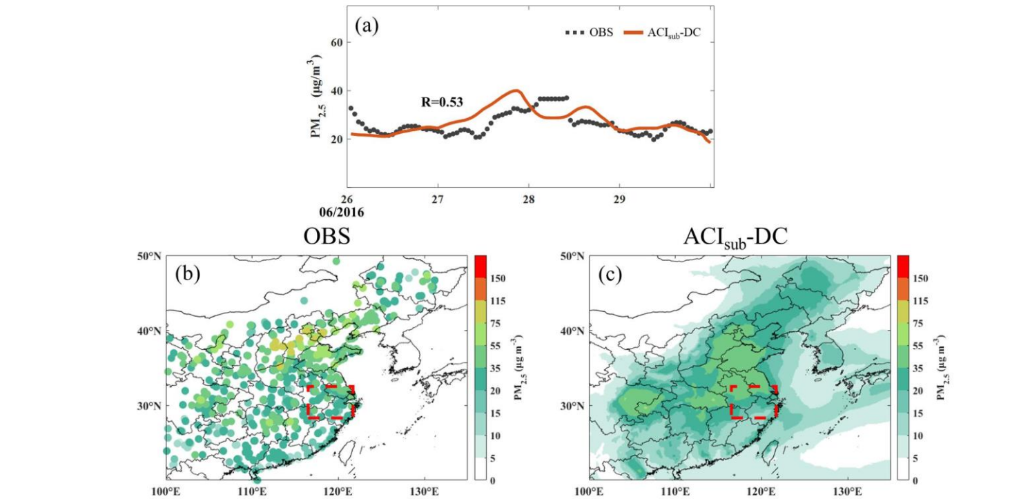
Figure 14. (a) The temporal variation of regional average PM_{2.5} mass concentration in YRD. The (b) spatial distribution of observed and (c) simulated by the ACI_{sub-DC} experiment time average PM_{2.5} mass concentration from 26 to 29 June 2016
