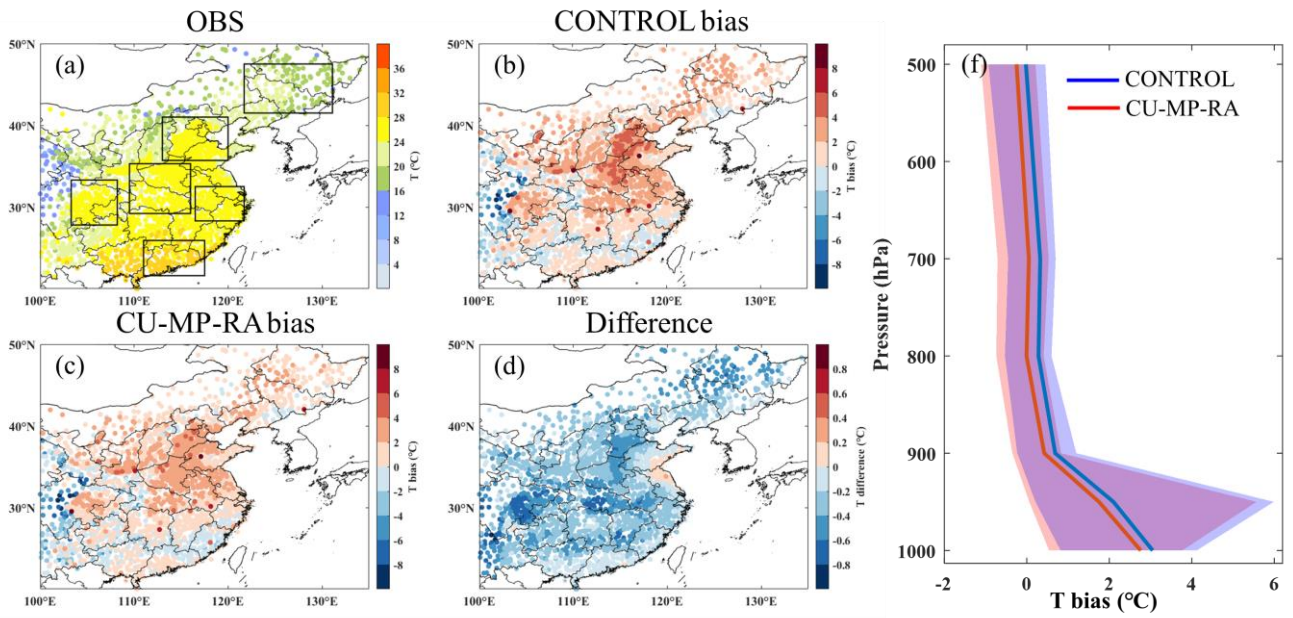
Figure 8: The spatial distribution of time average T2m and the vertical profiles of MB of temperature in June 2016. (a) The observations. (b) The MB of T2m in the NO-ACI sub CONTROL experiment. (c) The MB of T2m in the ACI sub CU-MP-RA experiment. (d) The difference of T2m between the ACI sub CU-MP-RA and NO-ACI sub CONTROL experiment. (f) The vertical profiles of MB of temperature in the NO-ACI sub CONTROL and ACI sub CU-MP-RA experiment. In the (f), the shadings are the spread of MB of temperature in six regions, and the solid lines are their average results.
