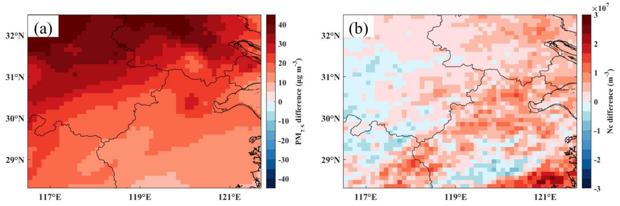
Figure 16: The spatial distribution of the difference between the ACI_{sub-DC} and CACI_{sub-DC} experiment for the time average (a) PM_{2.5} mass concentration and (b) subgrid-scale cloud droplets number concentration (mean values in 1-6 km) from 26 to 29 June 2016.
