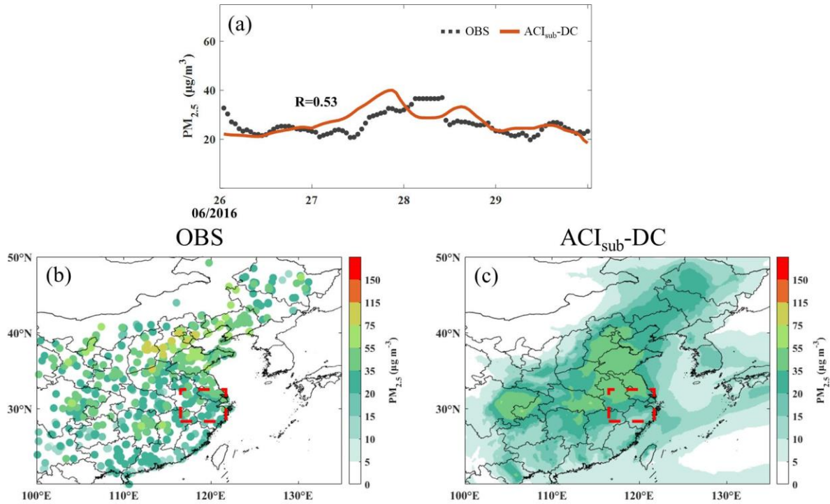
Figure 14. (a) The temporal variation of regional average \text{PM}_{2.5} mass concentration in YRD. The (b) spatial distribution of observed and (c) simulated by the ACI sub -DC experiment time average \text{PM}_{2.5} mass concentration from 26 to 29 June 2016
