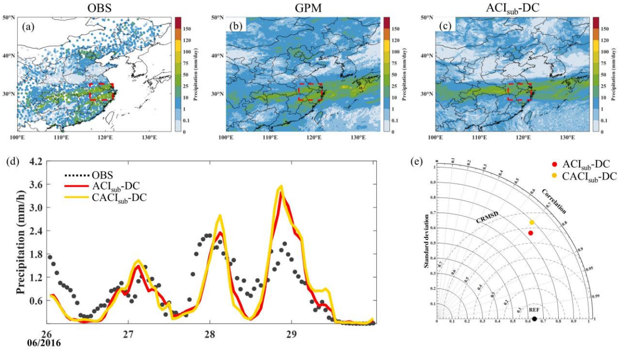
Figure 15: The spatial distribution of time average 24 hours cumulative precipitation from 26 to 29 June 2016 in the (a) observations, (b) GPM, and (c) ACI sub -DC experiment. The (d) time variation and (e) Taylor diagram of observed and simulated regional average hourly precipitation in YRD from 26 to 29 June. In the Taylor diagram, the REF is the observation, the vertical coordinate is the standard deviation (STD), the distance between the simulations and REF is the centered root mean square deviation (CRMSD), and the position of the azimuth is the correlation coefficient (R).
