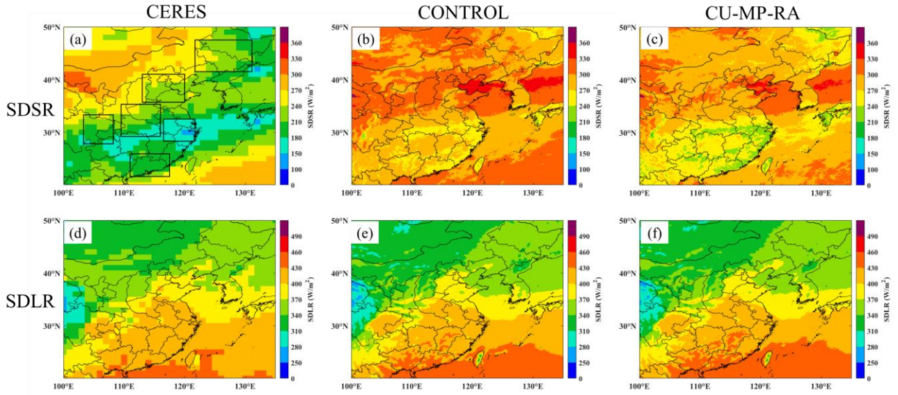
Figure 6: The spatial distribution of time average (a-c) SDSR, (d-f) SDLR in June 2016. The left, middle, and right column is the CERES, NO-ACI sub CONTROL , and ACI sub CU-MP-RA experiment, respectively.
