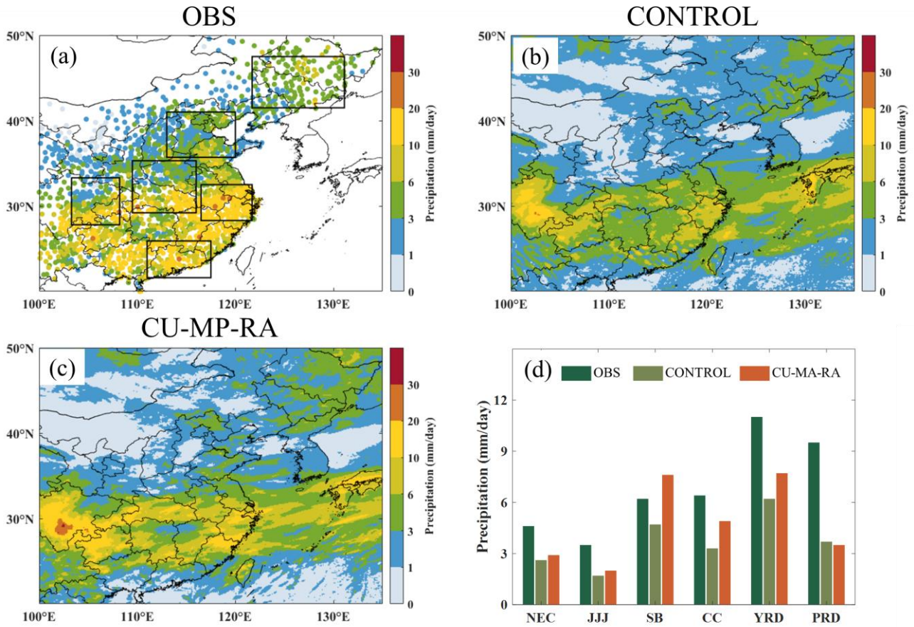
Figure 12: The spatial distribution of time average 24 hours cumulative precipitation in June 2016 from the (a) observations, (b) NO-ACI sub CONTROL experiment, and (c) ACI sub CU-MP-RA experiment. (d) The comparison of time average 24 hours cumulative precipitation in different regions.
