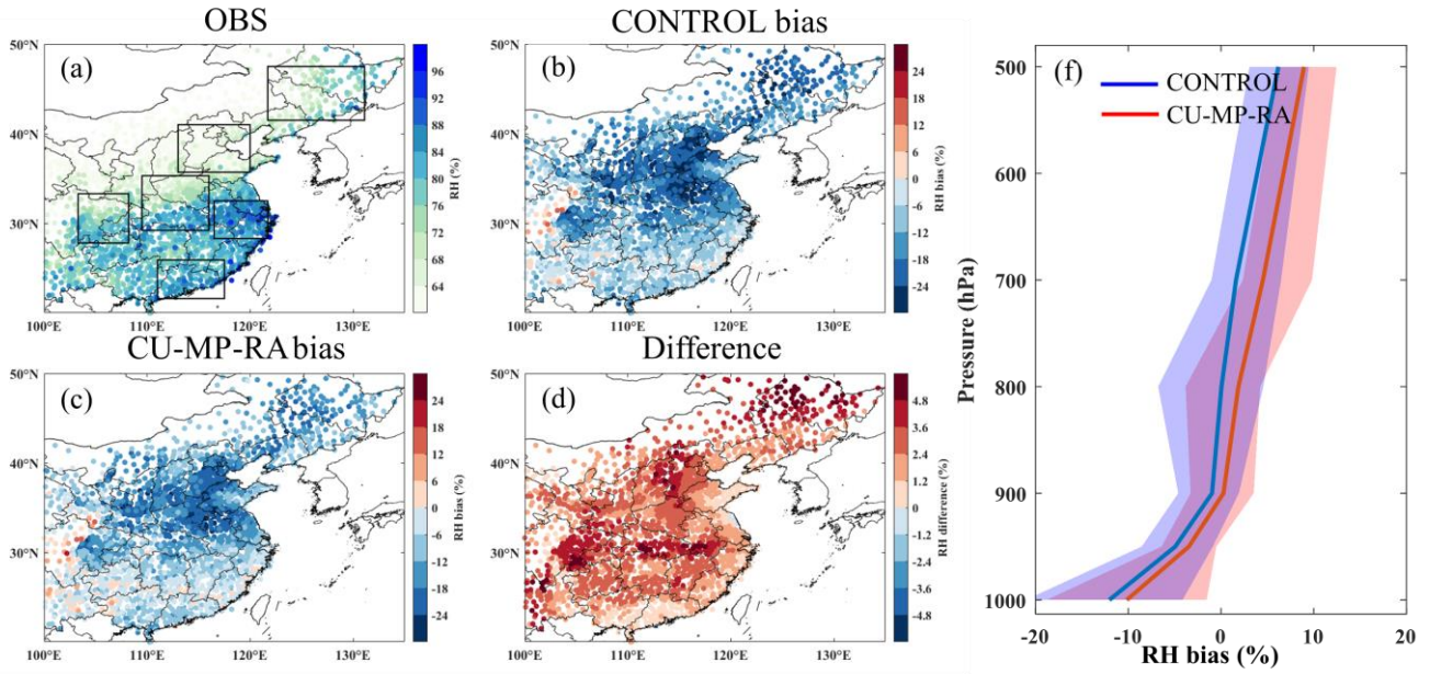
Figure 9: The spatial distribution of time average RH2m and the vertical profiles of MB of RH in June 2016. (a) The observations. (b) The MB of RH2m in the NO-ACI sub CONTROL experiment. (c) The MB of RH2m in the ACI sub CU-MP-RA experiment. (d) The difference of RH2m between the ACI sub CU-MP-RA and NO-ACI sub CONTROL experiment. (f) The vertical profiles of MB of RH in the NO-ACI sub CONTROL and ACI sub CU-MP-RA experiment. In the (f), the shadings are the spread of MB of RH in six regions, and the solid lines are their average results.
