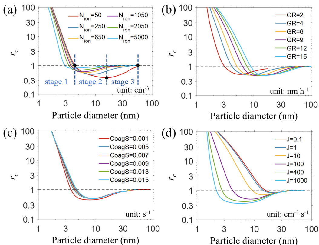
Figure 4. r_c as a function of particle diameter at different IIN conditions: (a) GR = 4 \text{ nm h}^{-1} , CoagS = 0.005 \text{ s}^{-1} , J = 100 \text{ cm}^{-3} \text{ s}^{-1} , (b) N_{ion} = 250 \text{ cm}^{-3} , CoagS = 0.005 \text{ s}^{-1} , J = 100 \text{ cm}^{-3} \text{ s}^{-1} , (c) N_{ion} = 250 \text{ cm}^{-3} , GR = 4 \text{ nm h}^{-1} , J = 100 \text{ cm}^{-3} \text{ s}^{-1} , (d) N_{ion} = 250 \text{ cm}^{-3} , CoagS = 0.005 \text{ s}^{-1} , GR = 4 \text{ nm h}^{-1} . The nucleation rate J is the sum of the formation rates of the positive and negative particles.
