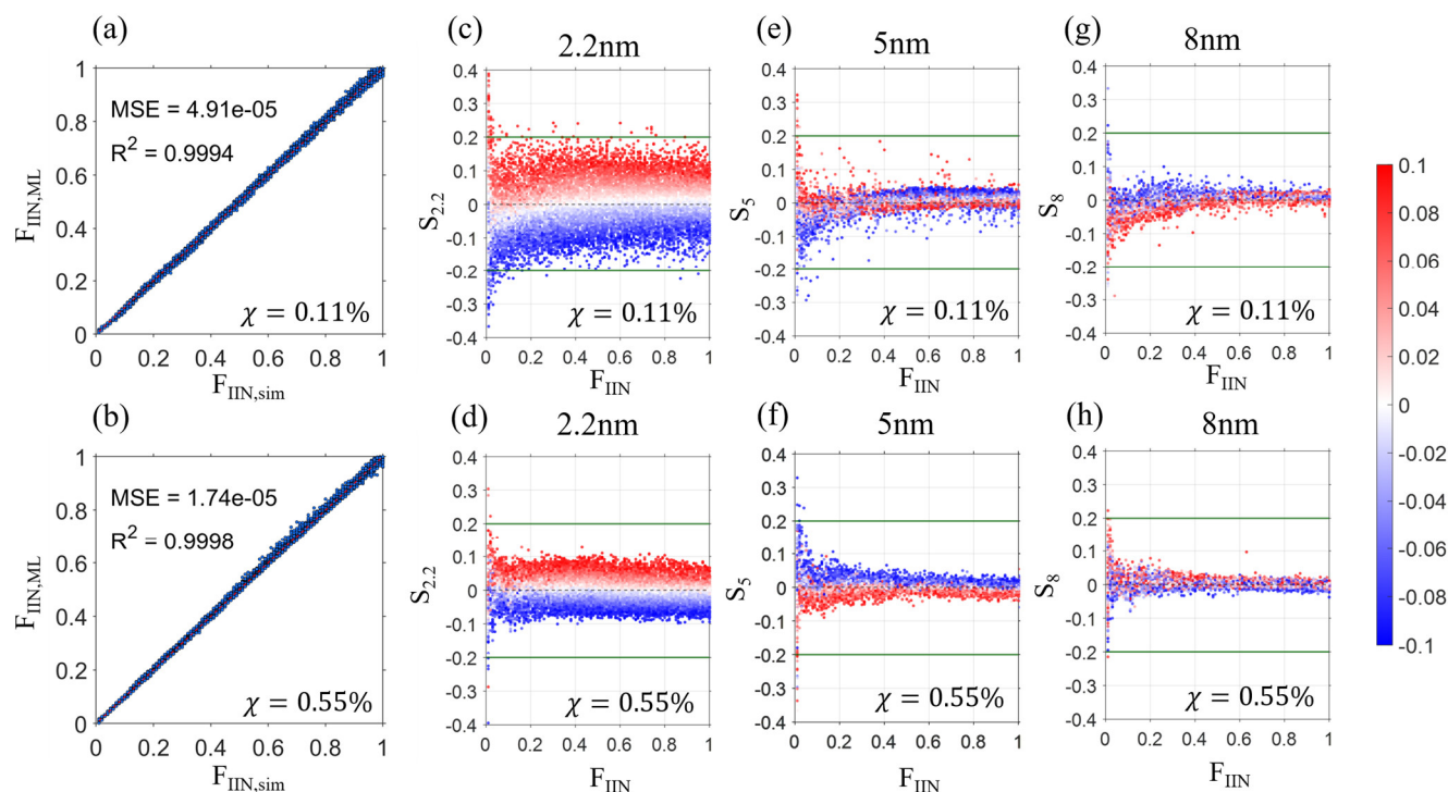
430 Figure 6. (a-b) Comparison between the predicted F_{\text{IIN}} by ResBWD and the true F_{\text{IIN}} used in CDMS-ion simulation. The upper and lower panels correspond to \chi values of 0.11% and 0.55%, respectively. (c-h) Sensitivity of F_{\text{IIN}} to noises of inputs including r_{c,2.2} , r_{c,5} , and r_{c,8} . The sensitivity is defined as S_x = \frac{F_{\text{IIN}}^{\text{noise}} - F_{\text{IIN}}}{F_{\text{IIN}}} , with the subscript x denoting the size at which r_c is varied. The green reference lines indicate S_x values of \pm 0.2 .
