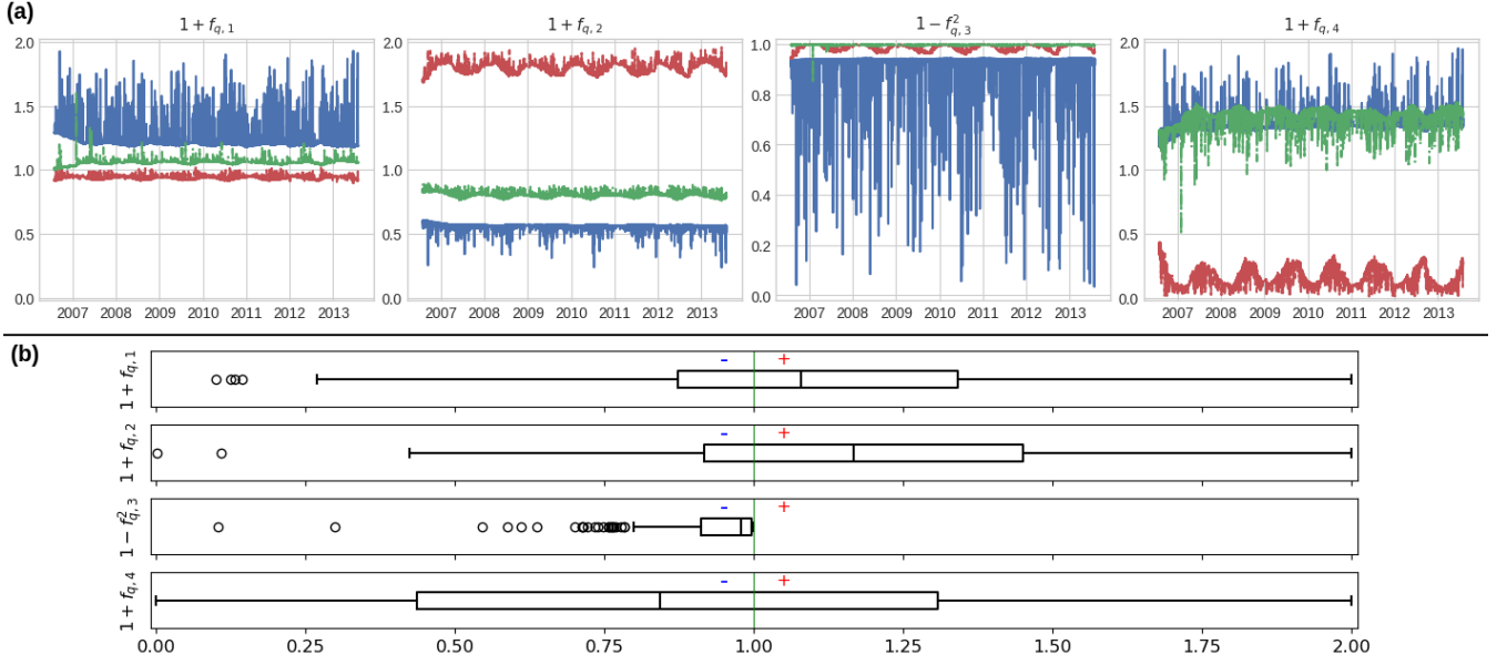
Figure B2. (a) Spatially averaged flux correction time series \overline{g(\mathbf{f}_q(t))}^{x \in \Omega_j} for the same three catchments selected in Figure 9a. These are obtained through local calibrations of spatially distributed parameters with the hybrid model structure (GRNN.D). (b) Boxplot of spatio-temporal average flux corrections \overline{g(\mathbf{f}_q)}^{x \in \Omega_j} , where each boxplot represents 235 catchment-specific spatio-temporal averages.
