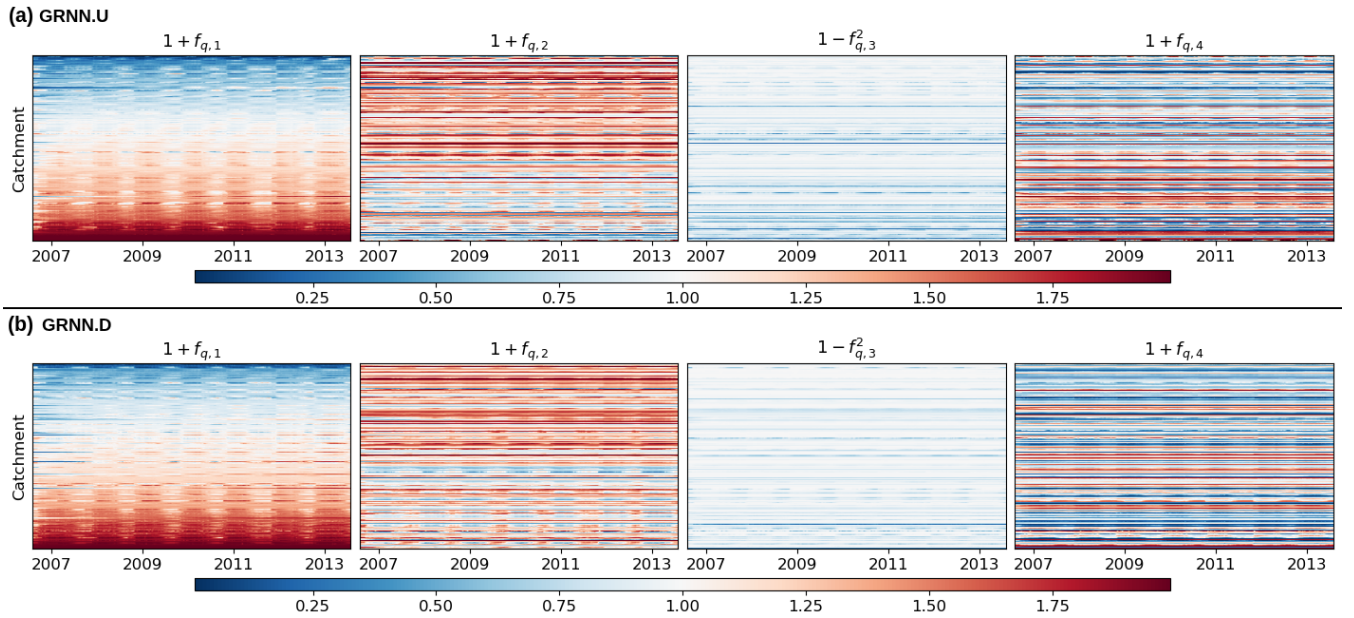
Figure B4. Heatmap of spatially averaged flux correction time series \overline{g(f_q(t))}^{x \in \Omega_j} , where j = 1..N_g , for the N_g = 235 catchments. These are obtained through local calibrations of (a) spatially uniform parameters with the hybrid model structure (GRNN.U), and (b) spatially distributed parameters with the hybrid model structure (GRNN.D).
