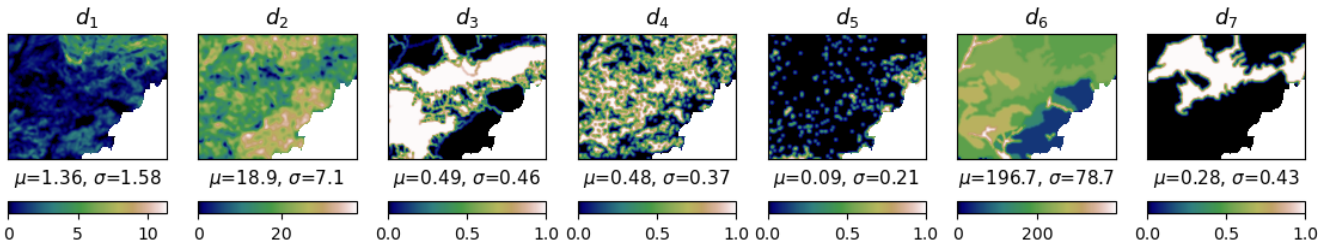
Figure A1. Maps of seven physical descriptors in the MedEst area at a resolution of 0.01^\circ in the WGS 84 projection, where \mu and \sigma represent the spatial average and standard deviation for each descriptor.
