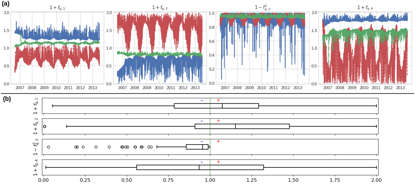
Figure 9. (a) Spatially averaged flux correction time series \overline{g(\mathbf{f}_q(t))}^{x \in \Omega_j} for three randomly selected catchments from the set of 235. These are obtained through local calibrations of spatially uniform parameters with the hybrid model structure (GRNN.U). (b) Boxplot of spatio-temporal average flux corrections \overline{g(\mathbf{f}_q)}^{x \in \Omega_j^t} , where each boxplot represents 235 catchment-specific spatio-temporal averages.
