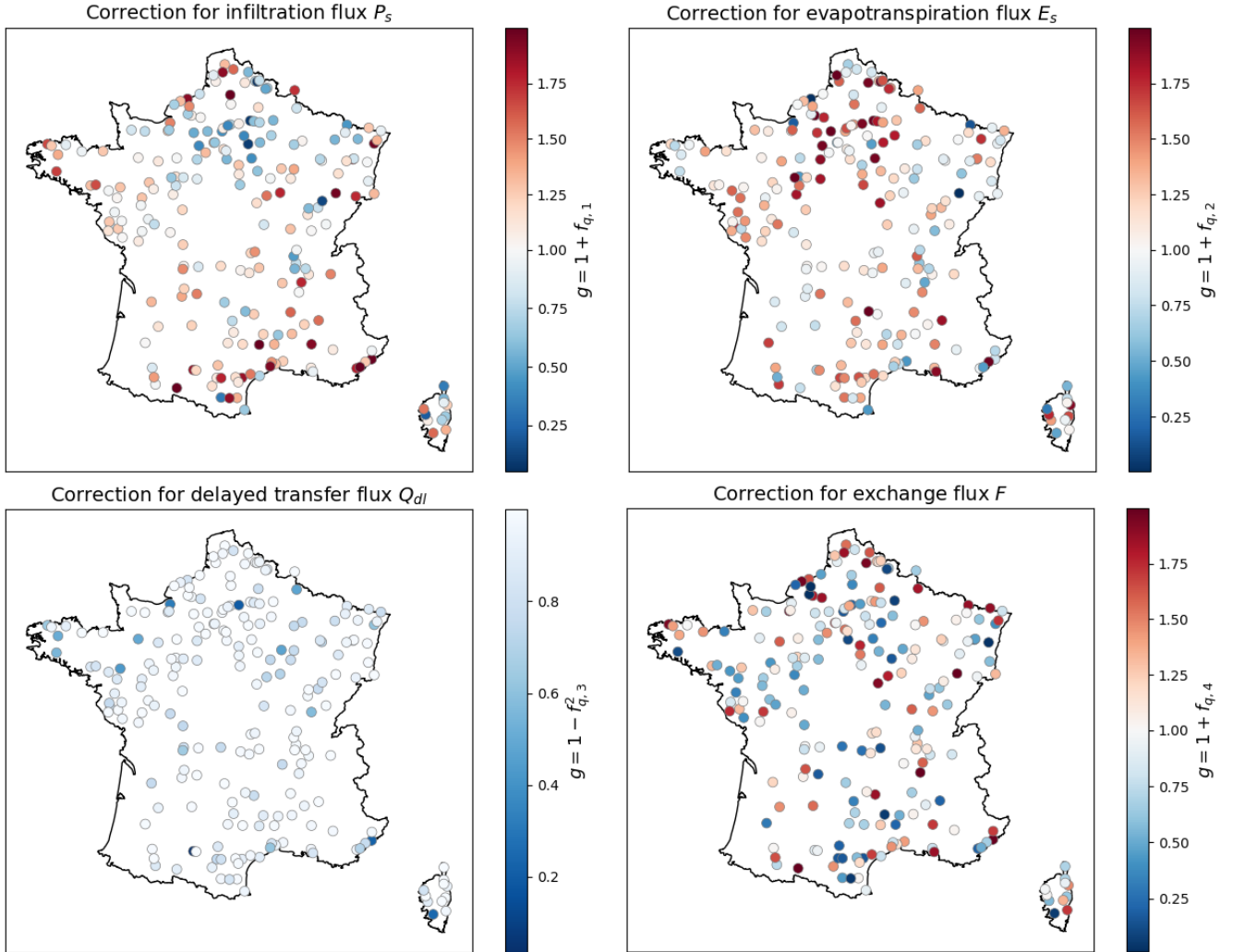
Figure 8. Maps of spatio-temporal average flux corrections \overline{g(\mathbf{f}_q)}^{x \in \Omega_j, t} , where j = 1..N_g , for the N_g = 235 catchments, obtained through local calibrations of spatially uniform parameters with the hybrid model structure (GRNN.U). The function g(\cdot) represents the transformation applied to the neural network output \mathbf{f}_q , which may differ depending on the specific flux being corrected. Red indicates corrections that tend to increase the current flux, while blue indicates corrections that reduce it, with white representing minimal or no effective correction.
