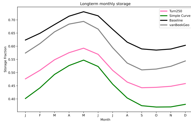
Figure A5. Depicts the longterm monthly average of the storage fractions for the three model in our analysis: Baseline (black), vanBeekGeo (grey) and Turn250 (pink) as well as the simplified release curve denoted as Simple Curve (green).
