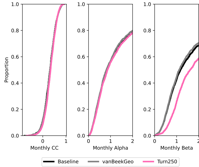
Figure A7. Shows the cumulative distribution functions of the KGE components, alpha, beta and R between the three models: Baseline (black), vanBeekGeo (grey) and Turn250 (pink) evaluated against point observations in GloLakes.
