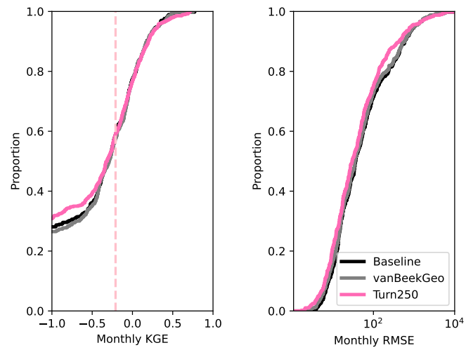
Figure A8. Depicts the KGE and RMSE CDFs for the storage evaluation with point location in GloLakes across the United States. The simulated models are depicted in black for Baseline, grey for the vanBeekGeo and pink for Turn250. The dashed pink line denotes the boundary above which the KGE values show significance.
