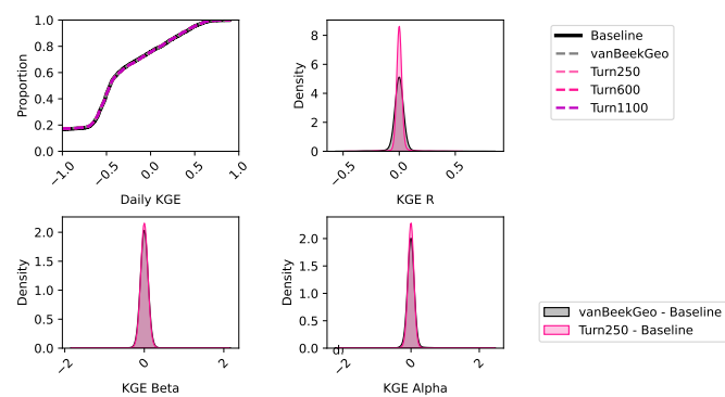
Figure A14. Show the KGE, and KGE components of the models we used in our analysis for Figure 5 in the manuscript without any zoom.
