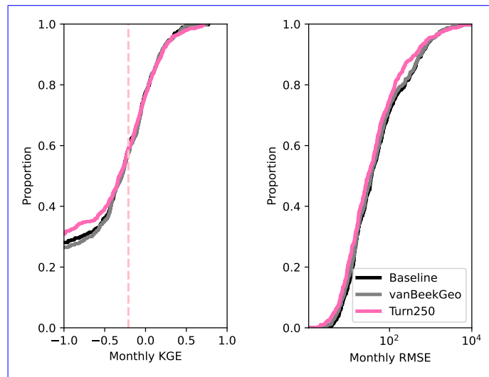
Figure A9. Depicts the KGE and RMSE CDFs for the storage evaluation with point location in GloLakes across the United States. The simulated models are depicted in black for Baseline, grey for the vanBeekGeo and pink for Turn250. The dashed pink line denotes the boundary above which the KGE values show significance.
