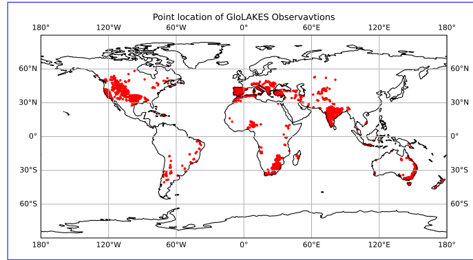
Figure A11. Point location map of all GeoDAR locations that are used in our analysis.
