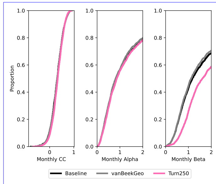
Figure A8. Shows the cumulative distribution functions of the KGE components, alpha, beta and R between the three models: Baseline (black), vanBeekGeo (grey) and Turn250 (pink) evaluated against point observations in GloLakes.
