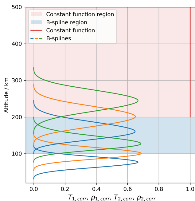
Figure 10. parametrization of the first and second order corrections with altitude. The parametrization contains three free parameters (two B-spline coefficients and one value for the constant function above 200 km altitude). Both the first and second order corrections for the temperature and the atomic oxygen concentration profiles utilise this parametrization, however with their own set of parameters.
