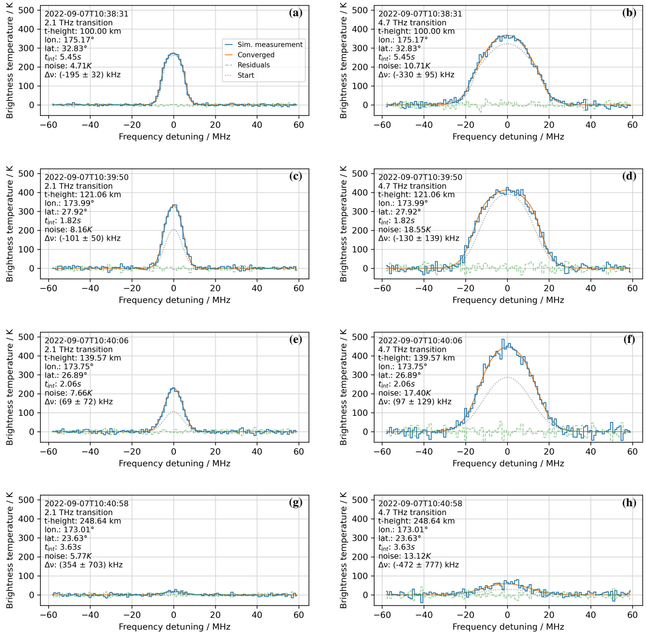
Figure 13. Examples of spectra from scan 14,15,16. In blue are the original simulated mission spectra. In orange are the spectra corresponding to the retrieved profiles and in grey are the spectra corresponding to the start profiles of the retrieval (see Figure 11). The tangential height, the time, the location of the satellite upon simulation, the integration time, and the simulated spectral noise (RMS) are annotated in the plots. The retrieved Doppler shifts ( \Delta\nu ) and the 1\sigma uncertainties are also annotated. (a, b) 2.1 THz and 4.7 THz spectra at tangential height 100 km. (c, d) 2.1 THz and 4.7 THz spectra at tangential height 121 km. (e, f) 2.1 THz and 4.7 THz spectra at tangential height 140 km. (g, h) 2.1 THz and 4.7 THz spectra at tangential height 249 km. The frequency axes corresponds to the rest frequencies of the atomic oxygen transitions (see Table 3).
