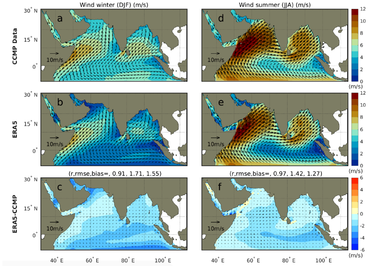
Figure R1. Surface wind (10m) during (a-c) winter (December-February) and (d-f) summer (June-August) monsoons. (a,d) CCMP satellite data, (b,e) ERA5 data product and (c,f) differences between ERA5 and CCMP. Correlation coefficients r , root-mean squared error (rmse) and bias between ERA5 and CCMP seasonal means are indicated. Wind data is from CCMP satellite (see details in Table 2). ERA5 results are averaged over the 1980-2020 period.
