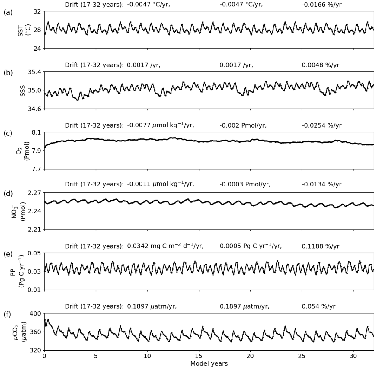
Figure R3. Time series of domain-mean model variables during the 32-year spin-up forced by repeated atmospheric and open boundary conditions looping over 1980–1987. Panels show: (a)
