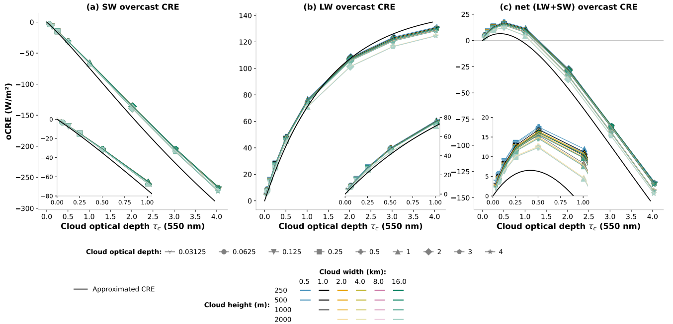
Figure 3. Overcast cloud radiative effect in the (a) SW, (b) LW and (c) net (SW+LW) as a function of cloud optical depth. Calculations done with htrdr using the ICA are in identical colors as in Fig. 2. Compared with Fig. 2, all curves overlap because the oCRE is independent of cloud width. Symbols indicate cloud optical depth. The oCRE approximated with the simple model is plotted in black lines.
