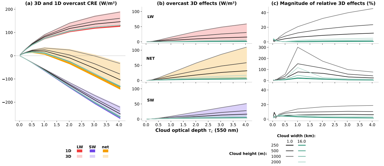
Figure 4. (a) Overcast cloud radiative effect, in W/m^2 , as a function of cloud optical depth. Dark lines represent 1D calculations, light shadings show the range of 3D calculations for various cloud heights and widths. Red is for LW, purple for SW and orange for net (SW+LW) CRE. Black and green lines correspond to two cloud configurations, with 1 km and 16 km width, respectively. They both come in different shades, from dark to light, to represent the cloud height h , between 250 m and 2 km. (b) 3D effects, i.e. difference between 3D and 1D oCREs in W/m^2 . Light shadings represent the range of the 3D effects, and the black and green lines are as in the first panel. (c) relative difference between 3D and 1D calculations, for each spectral domain : LW on top, SW on the bottom row and net in the middle.
