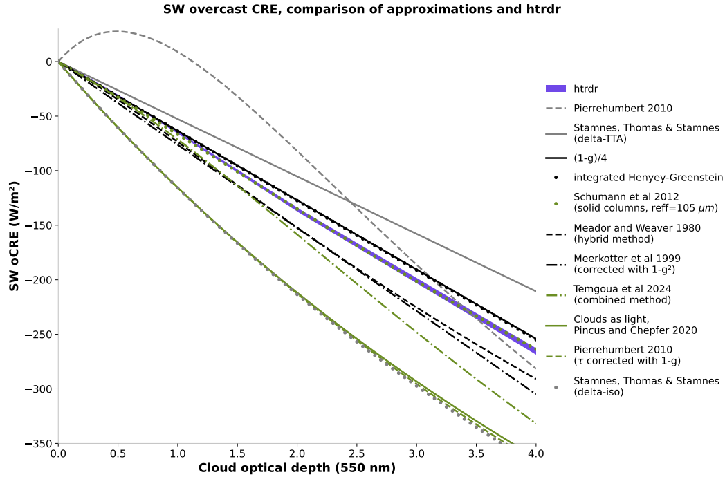
Figure C1. Comparison between SW CRE calculated with htrdr with the independent column approximation (purple) and the different expressions found in the literature listed in Table C2, for a Sun at zenith, as a function of cloud optical depth.
