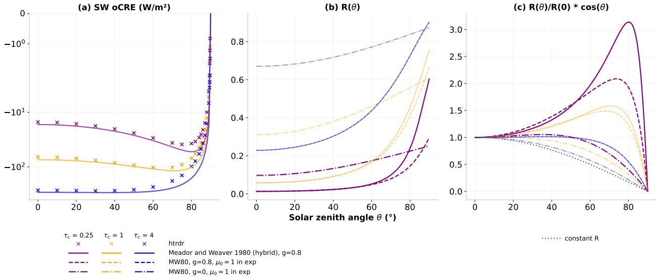
Figure 6. (a) SW overcast cloud radiative effect, in W/m 2 , as a function of solar zenith angle \theta for a cloud with width 1 km and height 500 m. Lines denote Meador and Weaver (1980) approximations and crosses denote htrdr calculations using the independent-column approximation ICA. Three cloud optical depths are shown : 0.25 in purple, 1 in yellow and 4 in blue. Note the logarithmic scale on the y-axis. (b) Cloud reflectivity and (c) Ratio of cloud reflectivity to cloud reflectivity at zenith multiplied by the cosine of solar zenith angle, for several approximations, as a function of solar zenith angle. Colors are as panel (a). Dashed lines show MW80 with \mu_0 = 1 in the exponential term, and dashdotted lines show MW80 with both \mu_0 = 1 and g = 0 . The dotted grey line in panel (c) illustrates the case of a constant reflectivity, i.e. \cos(\theta) .
