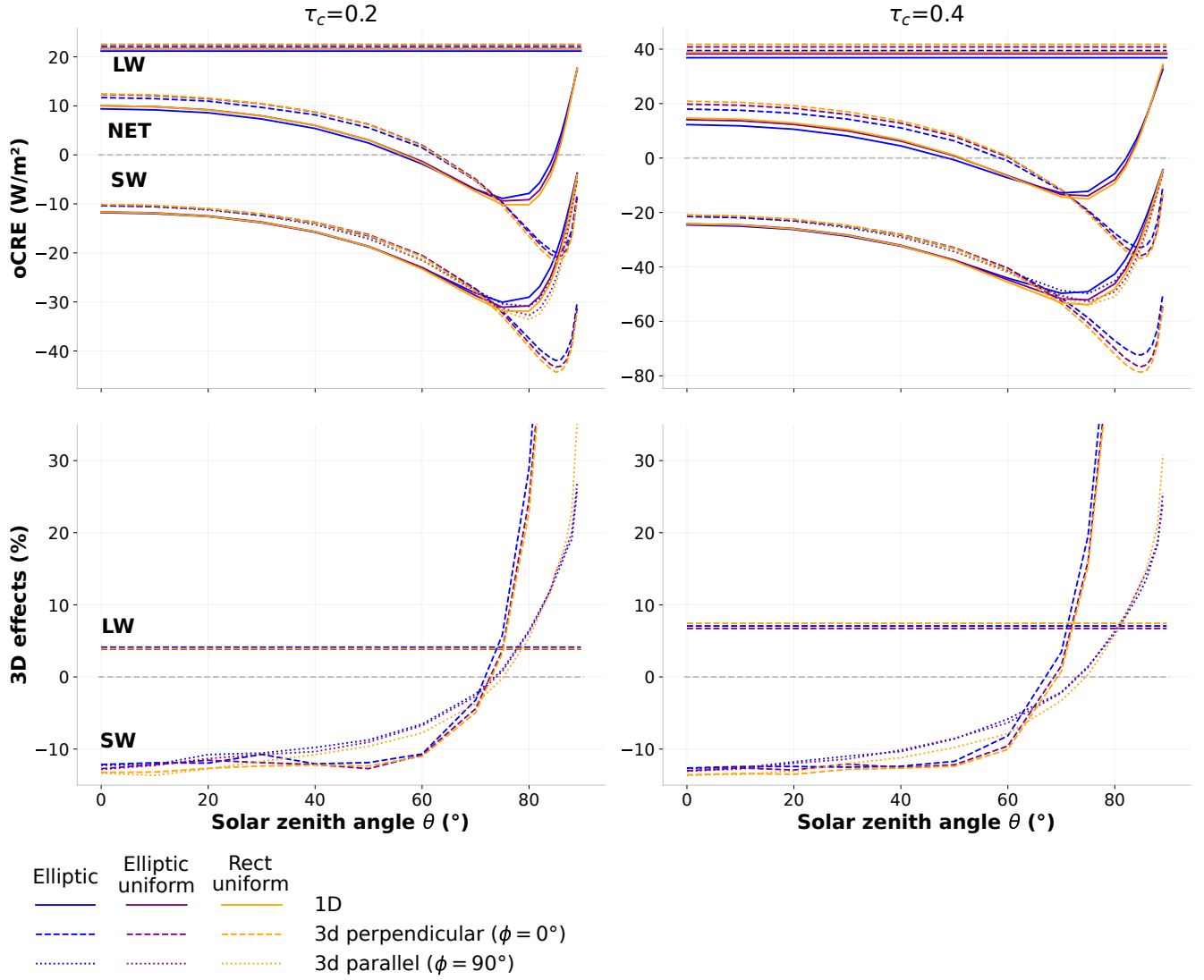
Figure 8. Top row: LW , SW and net oCRE (in \text{W/m}^2 ) as a function of solar zenith and azimuth angles, for a 800 m wide and 400 m thick cloud, for a cloud optical depth of 0.2 (left panel) and 0.4 (right panel). Bottom row: LW and SW 3D effects relative to 1D calculations, in %. Clouds with elliptic shape and inhomogeneous IWC are in blue, elliptic shape with uniform IWC in purple, and rectangle shape with uniform IWC in orange.
