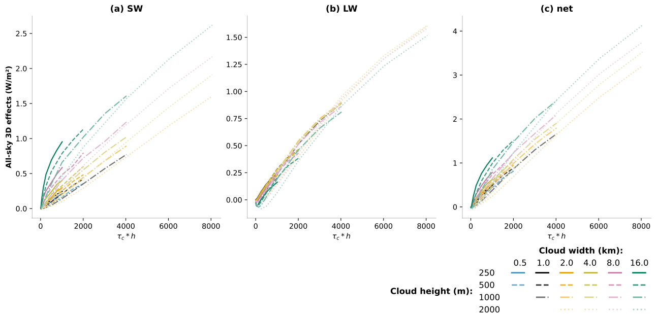
Figure 5. (a) SW, (b) LW and (c) net all-sky 3D effects in \text{W/m}^2 as a function of the product of cloud optical depth and cloud height \tau_c \times h . The colors and linestyles are as in figure 1.
