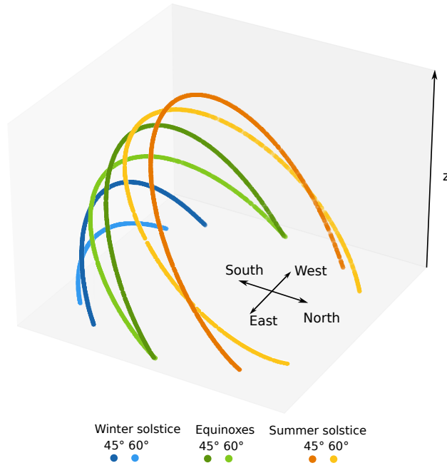
Figure 9. Illustration of Sun paths at selected dates and locations. Summer solstice in orange, equinox in green and winter solstice in blue. In the examples shown here, the Sun reaches the lowest zenith angle (i.e. the highest position in the sky) during summer solstice at 45 degrees of latitude. See also Fig. E1 in appendix.
