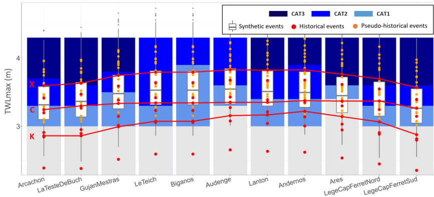
Figure 6: Categories of impact (CAT) related to SSH_{max}-TWL_{max} and repartition of the scenarios of the datasets: synthetic (box plots), historical (red points) and pseudo-historical (orange points). Red lines illustrate the variations of SSH_{max}-TWL_{max} for Klaus (K), Céline (C) and Xynthia (X).
