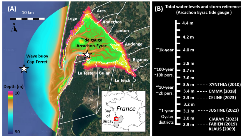
Figure 1: A) Location and bathymetric map of the study site: white stars indicate the location of the tide gauge named Arcachon-Eyrac (sea-level) and the wave buoy named Cap-Ferret. B) Total Sea-Water levels (m NGF) with associated return periods and historical storms references. Background is from GoogleEarth©
