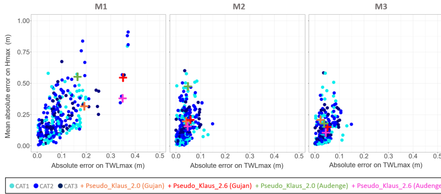
Figure 10: Relation between \text{SSHTWL}_{\text{max}} and Hmax errors for each method M1-M3. Each point represents the MAE calculated for one municipality and for one pseudo-historical event.
