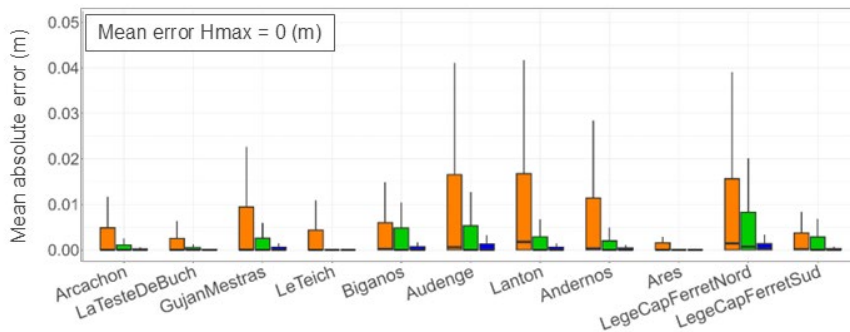
9 Figure C1: Mean absolute error (MAE) calculated over the non-flooded mesh nodes (with Hmax=0 in the 10 numerical simulations) of each municipality from the cross-validation procedure. 11 12 13
