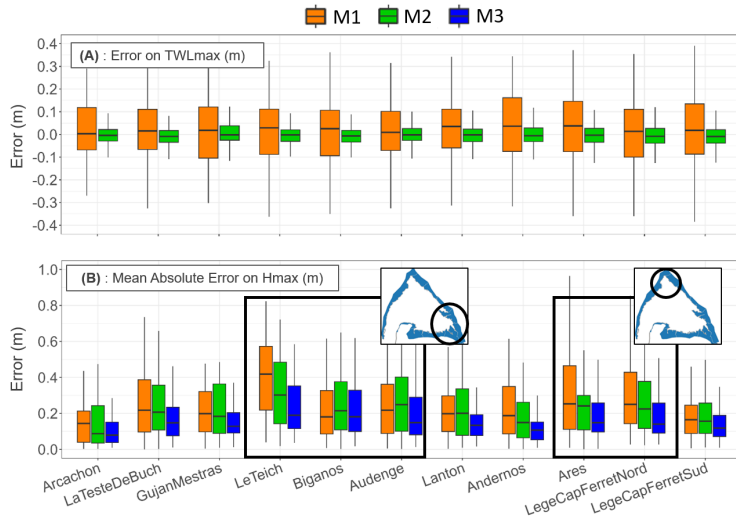
Figure 8: Error on SSH TWL max (A) and Mean Absolute Errors for Hmax by restricting the analysis to the mesh nodes that are flooded, i.e. for Hmax > 0, in the numerical simulation (B) calculated with the 10-fold cross validation (Seet,Section 3.2). Box plots represent the 25 th and 75 th percentiles.
