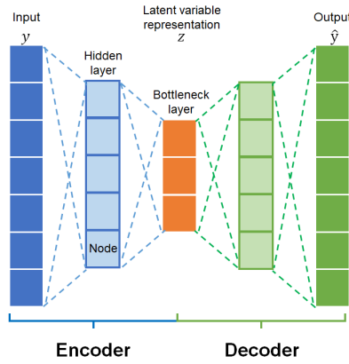
Figure B1: Typical autoencoder architecture.
