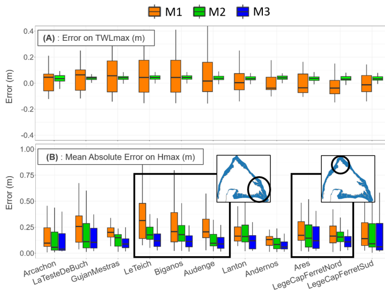
Figure 9: Errors on SSH TWL max (A) and Mean Absolute Errors on Hmax by restricting the analysis to the mesh nodes that are flooded, i.e. for Hmax > 0, in the numerical simulation (B) calculated with the validation cases ( Sect. Section 3.2 ). Box plots represent the 25 th and 75 th percentiles.
