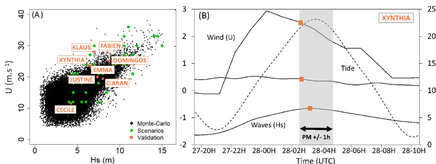
Figure 2: A) Monte-Carlo simulations (black points), synthetic (green points) and historical or validation (orange points) storm conditions at high tide. B) Example of storm parameters time series and extraction of conditions at high tide (orange points) for storm Xynthia (2010).
