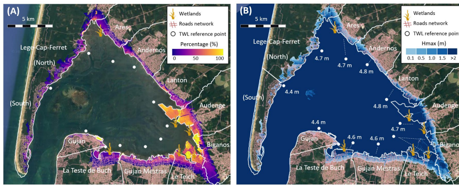
Figure 5: A) Percentage of scenarios (calculated from the learning database) leading to marine flooding on each node of the model mesh. B) Sea-level water levels denoted SSH_{max}TWL_{max} on the municipalities
