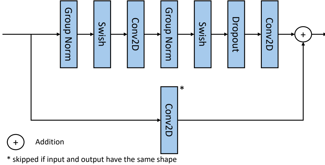
Figure B1. Structure of the residual block employed in our deep learning model. The arrangement is based on the design of Esser et al. (2020)
