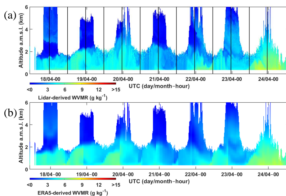
Figure 3. a) Raman lidar- and b) ERA5-derived WVMR vertical profiles during the ADM-AEOLUS field campaign. Average radiosonde times are indicated by vertical black lines in a).
