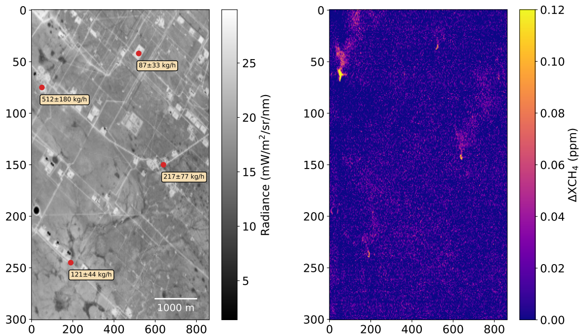
Figure 2. \Delta\text{XCH}_4 map retrieved from a MethaneAIR data granule from the RF06 Permian campaign. A map of the at-sensor radiance at 1623 nm is shown on the left panel, and the retrieved \Delta\text{XCH}_4 map is displayed on the right. The red points and the text boxes on the radiance map depict the location and flux rate of the four plumes detected in this subset.
